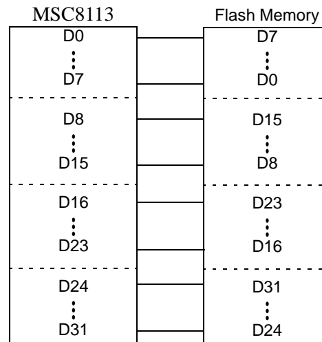
Figure 1. MSC8113 to Flash Memory Byte Lane Reversal
