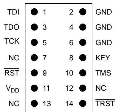
Figure 2. 14-Pin Header for JTAG/EOnCE Interface
