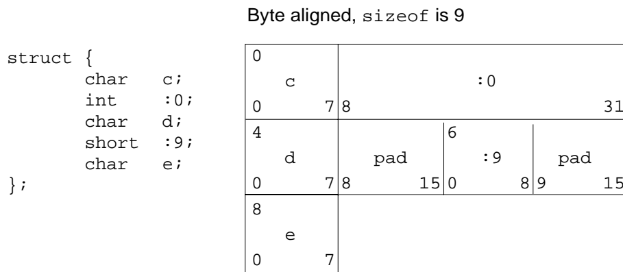
Figure 3-24 Unnamed Bit-Fields—Big-Endian
