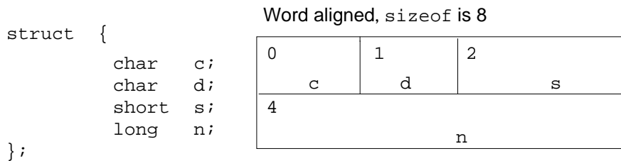
Figure 3-7 No Padding—Big-Endian
