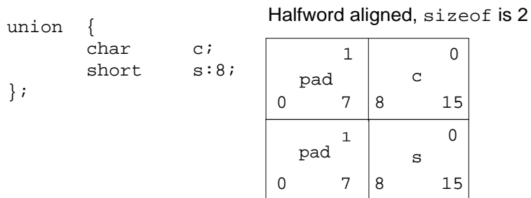
Figure 3-21 union Allocation—Little-Endian
