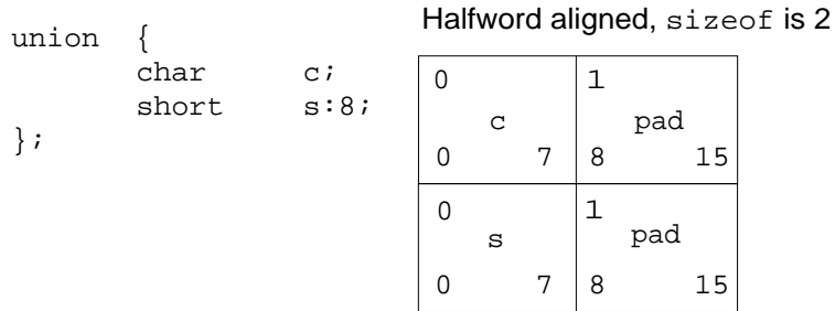
Figure 3-22 union Allocation—Big-Endian
