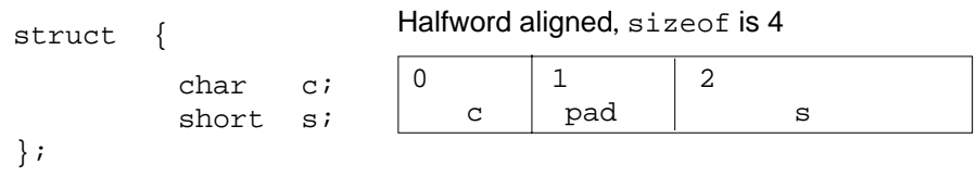
Figure 3-9 Internal Padding—Big-Endian
