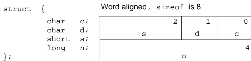
Figure 3-6 No Padding—Little-Endian
