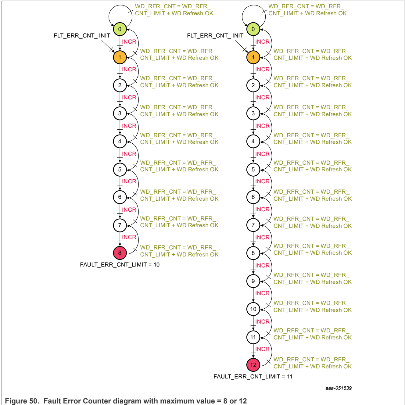
Figure 50. Fault Error Counter diagram with maximum value = 8 or 12
