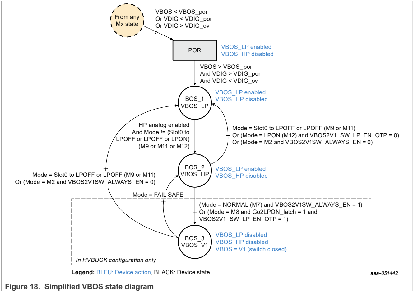
Figure 18. Simplified VBOS state diagram
