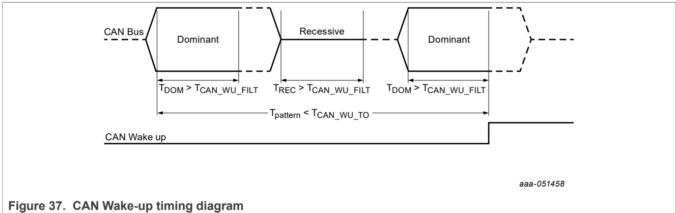
Figure 37. CAN Wake-up timing diagram
