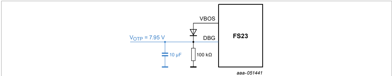
Figure 17. Debug pin (DBG) circuitry
