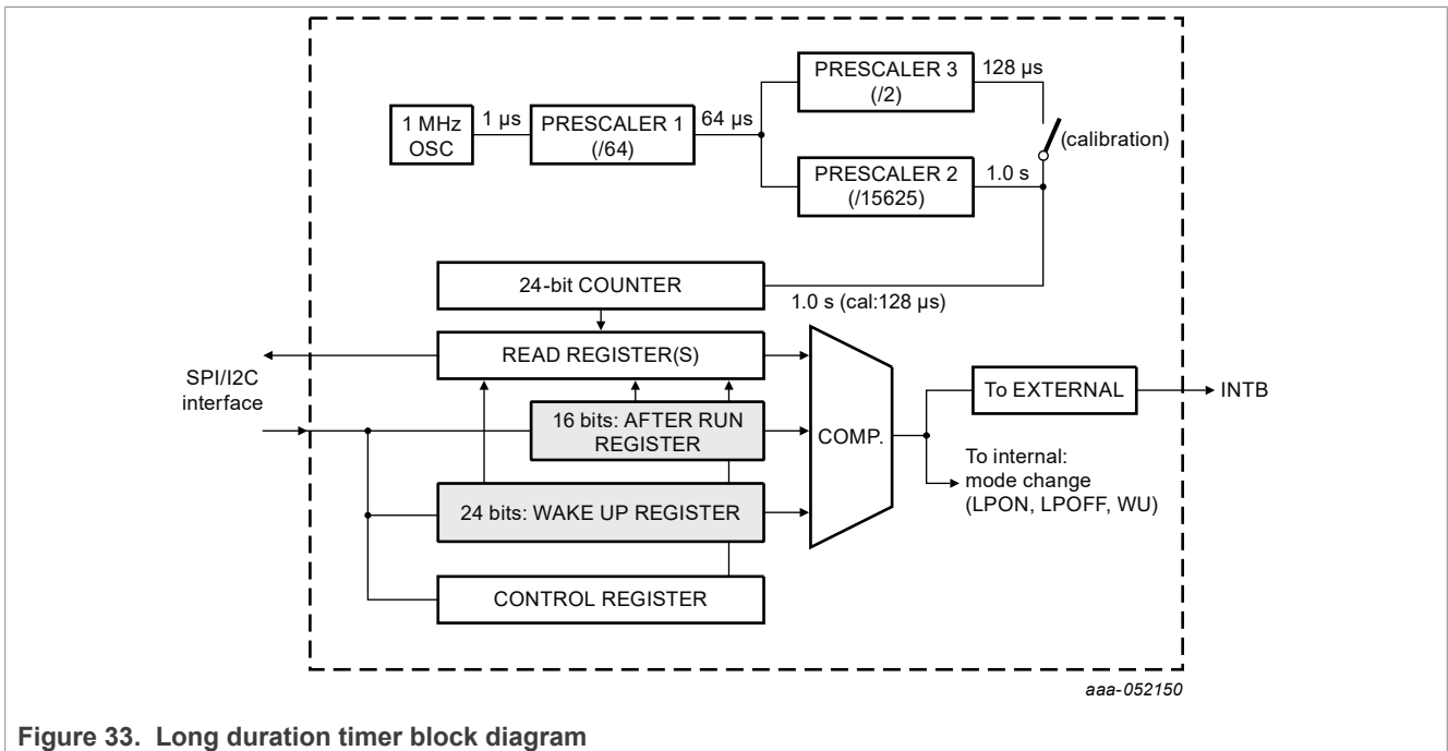
Figure 33. Long duration timer block diagram
