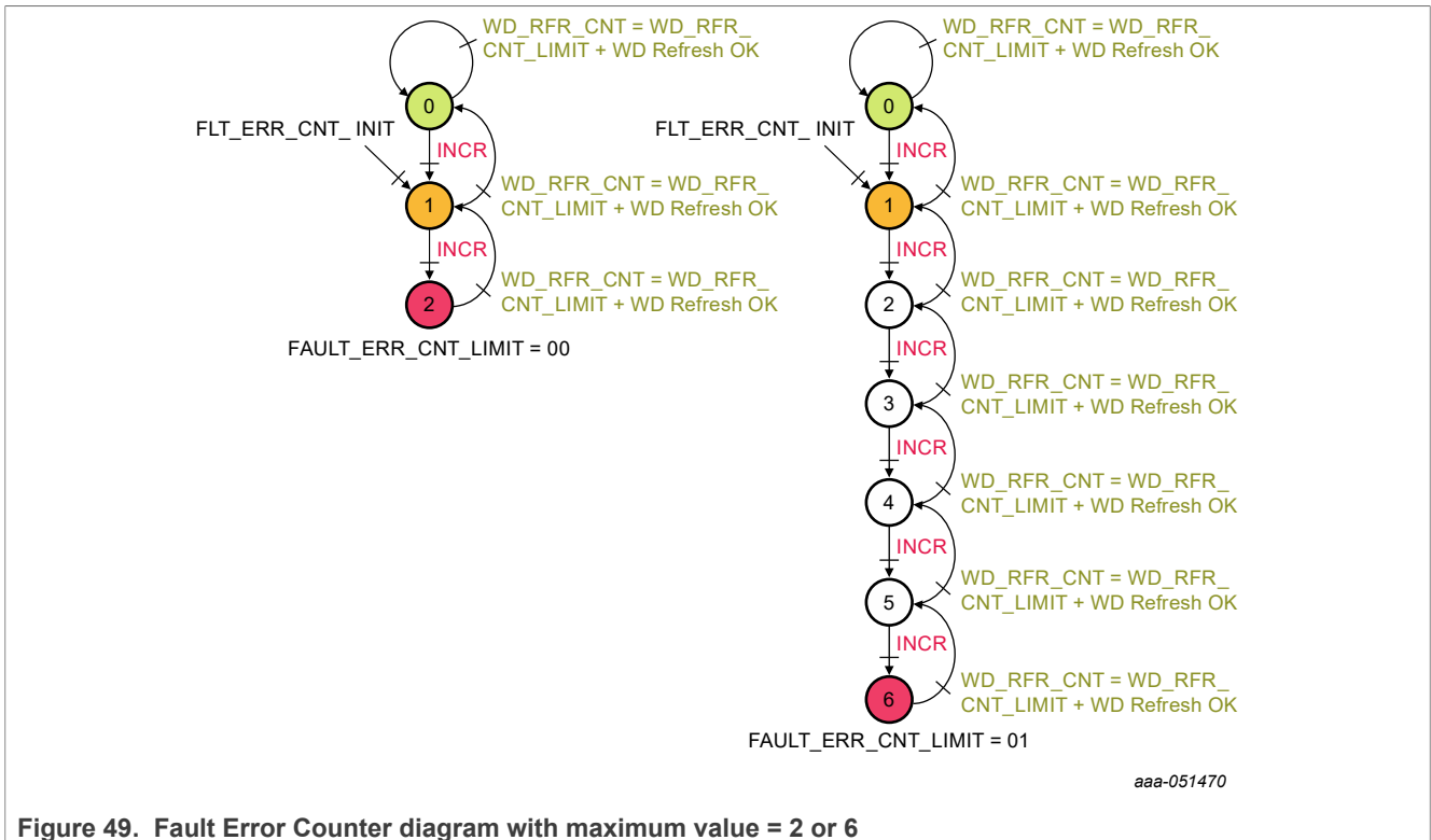
Figure 49. Fault Error Counter diagram with maximum value = 2 or 6
