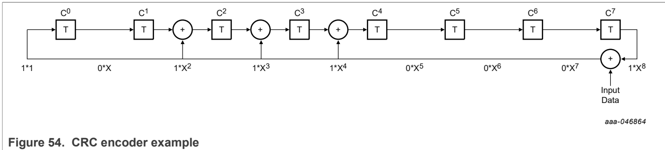
Figure 54. CRC encoder example
