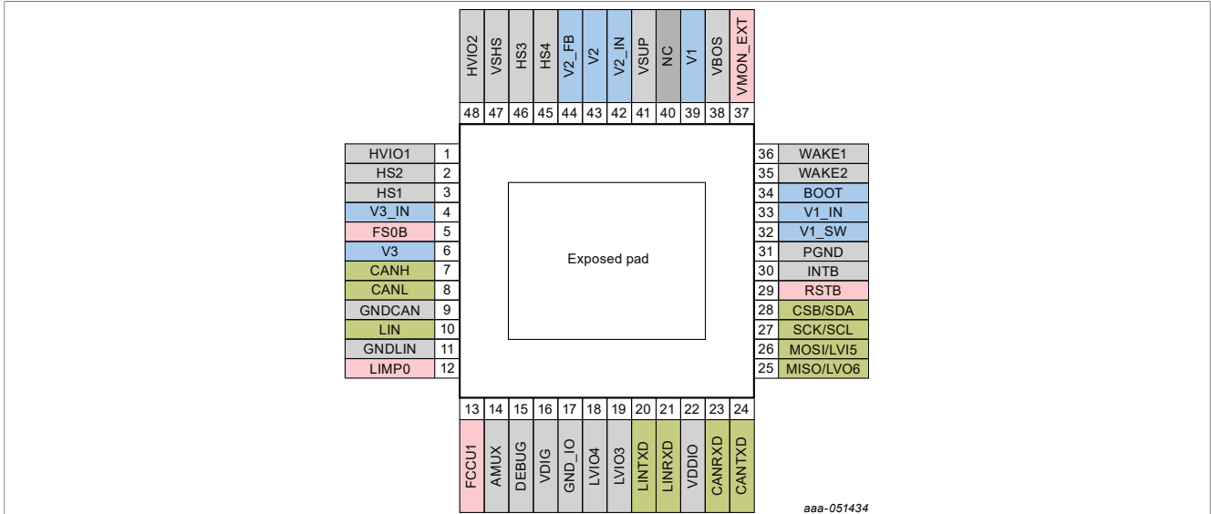
Figure 8. FS2320 Pin configuration (HVBUCK)
