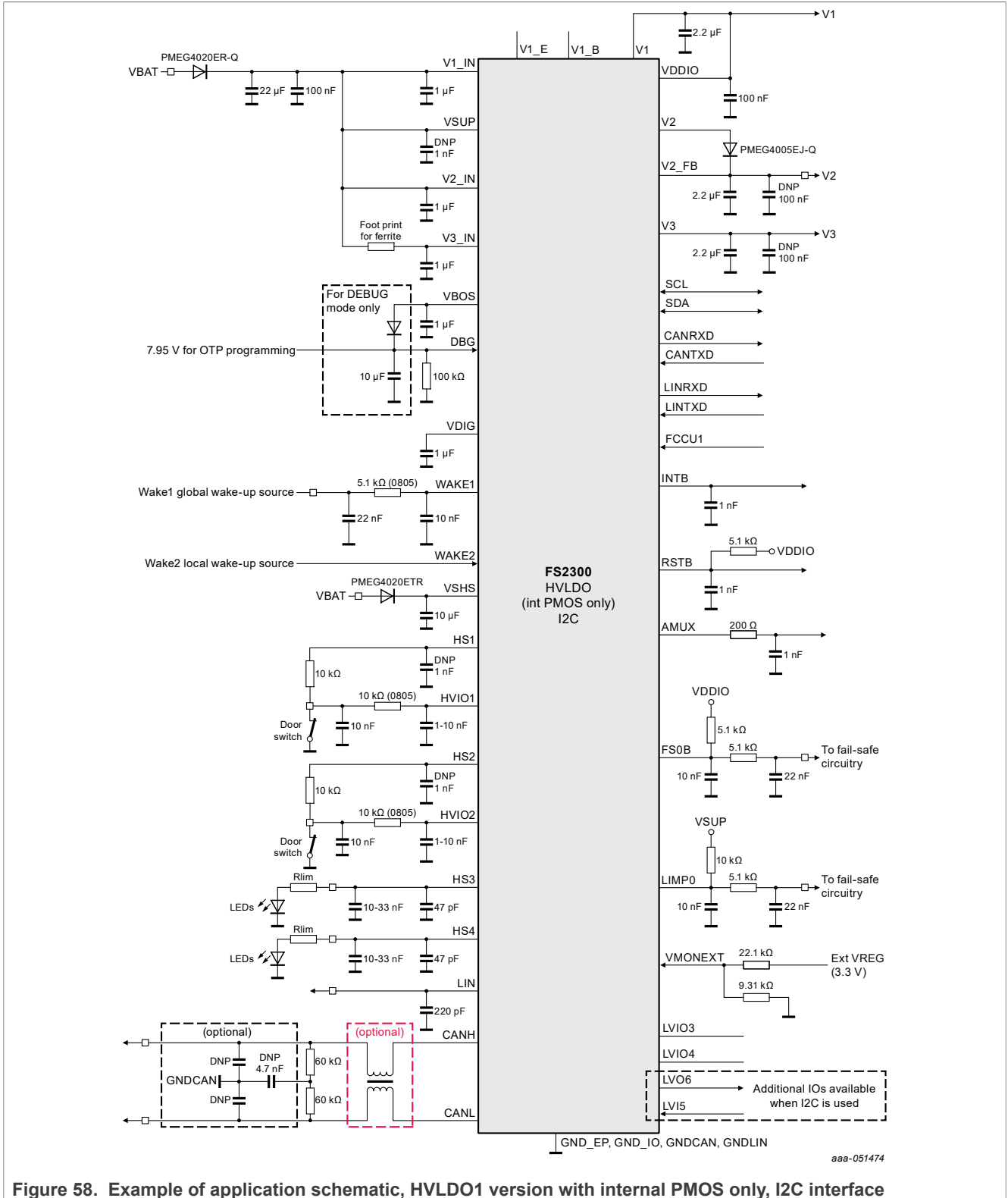
Figure 58. Example of application schematic, HVLDO1 version with internal PMOS only, I2C interface
