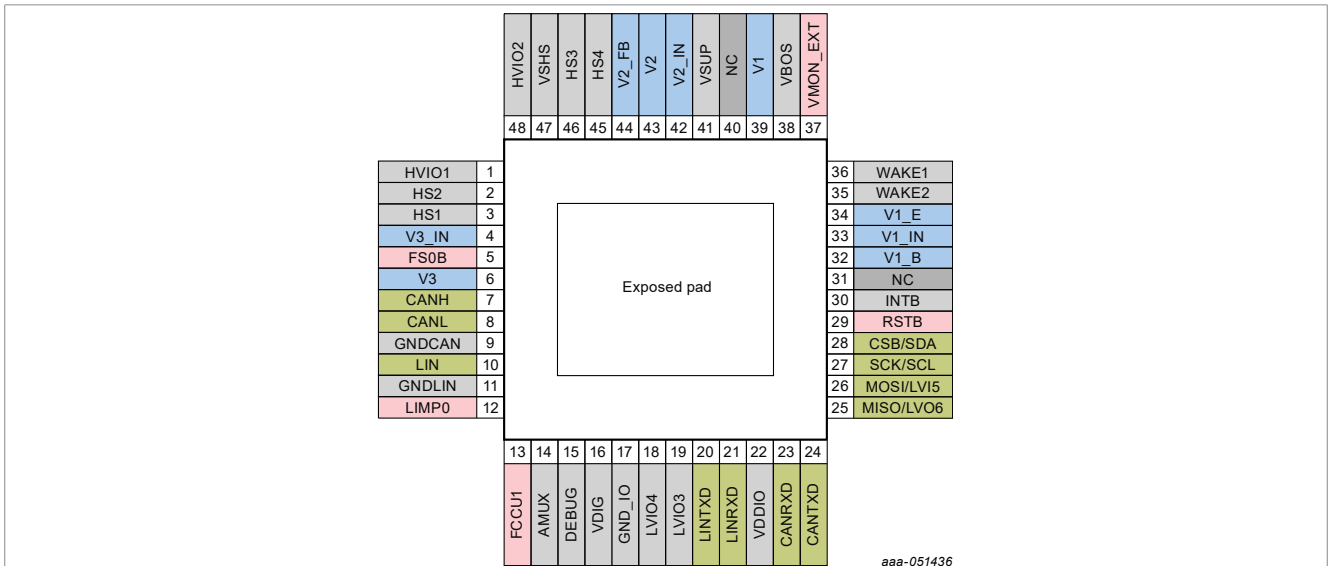
Figure 9. FS2300 Pin configuration (HVLDO1)
