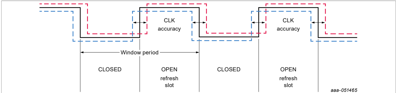
Figure 44. Window watchdog time diagram
