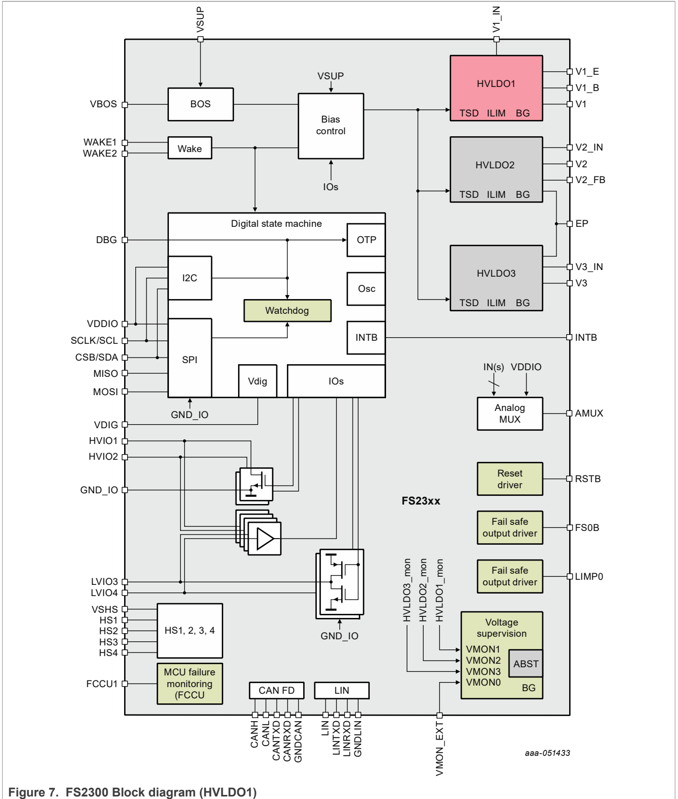
Figure 7. FS2300 Block diagram (HVLDO1)
