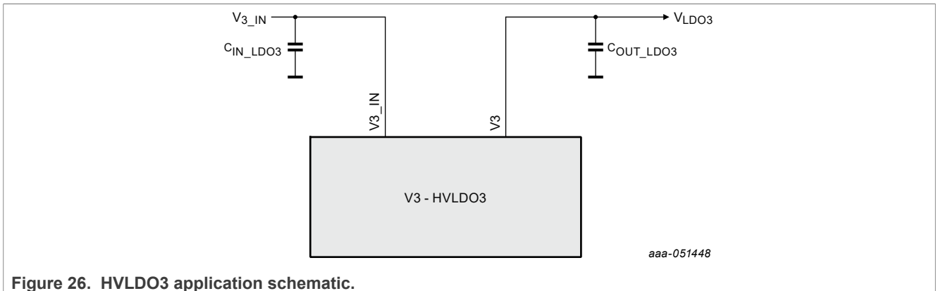
Figure 26. HVLDO3 application schematic.
