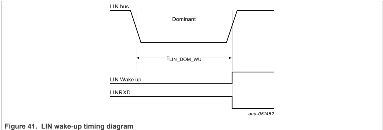
Figure 41. LIN wake-up timing diagram
