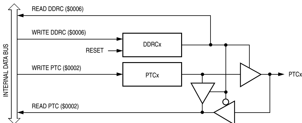
Figure 9-11. Port C I/O Circuit
