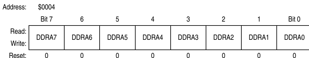
Figure 9-3. Data Direction Register A (DDRA)
