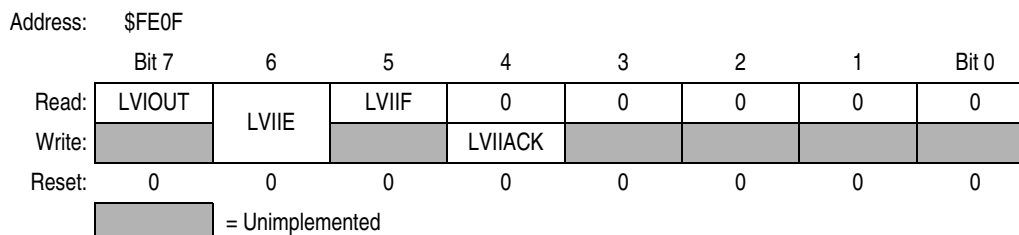
Figure 13-2. LVI Status Register (LVISR)
