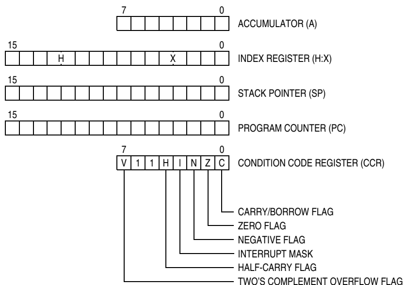
Figure 14-1. CPU Registers
