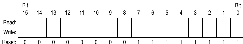
Figure 14-4. Stack Pointer (SP)
