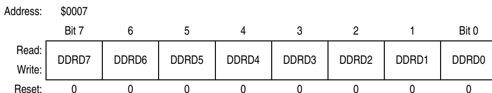
Figure 9-13. Data Direction Register D (DDRD)
