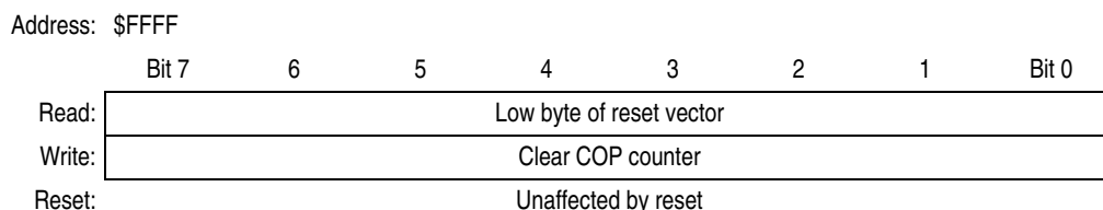
Figure 12-2. COP Control Register (COPCTL)
