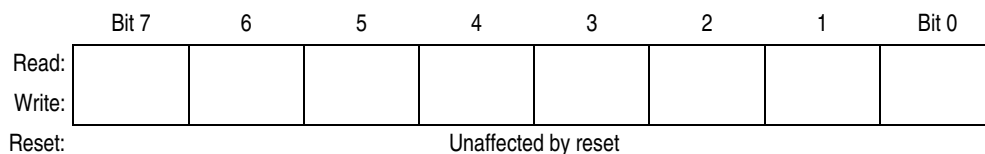
Figure 14-2. Accumulator (A)
