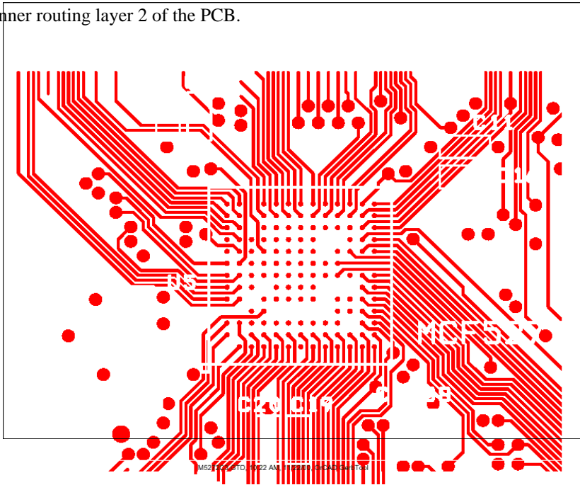
Bottom routing layer of the PCB.
