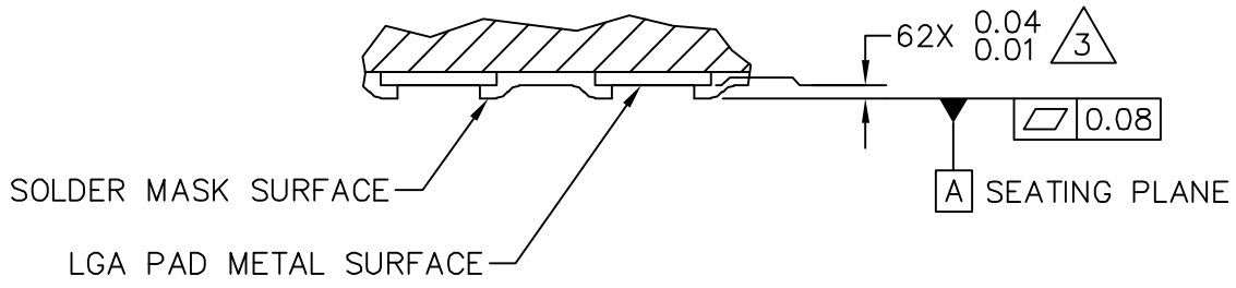
DETAIL D VIEW ROTATED 90° CW
