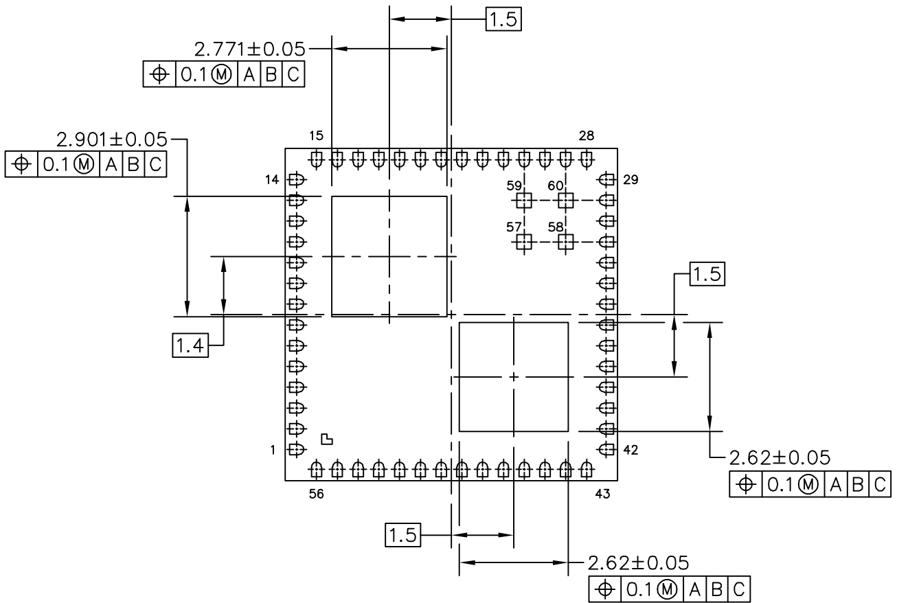
BOTTOM VIEW
