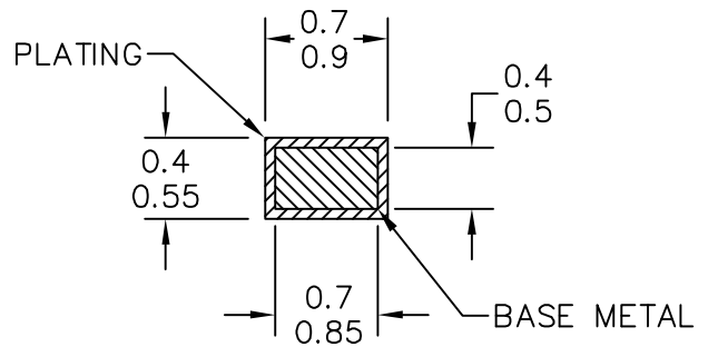
SECTION G-G
