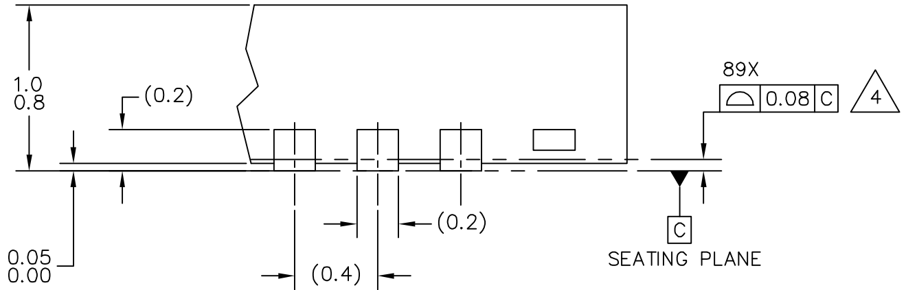
DETAIL G VIEW ROTATED 90°CW
