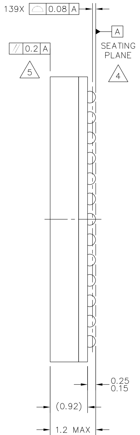
SIDE VIEW
