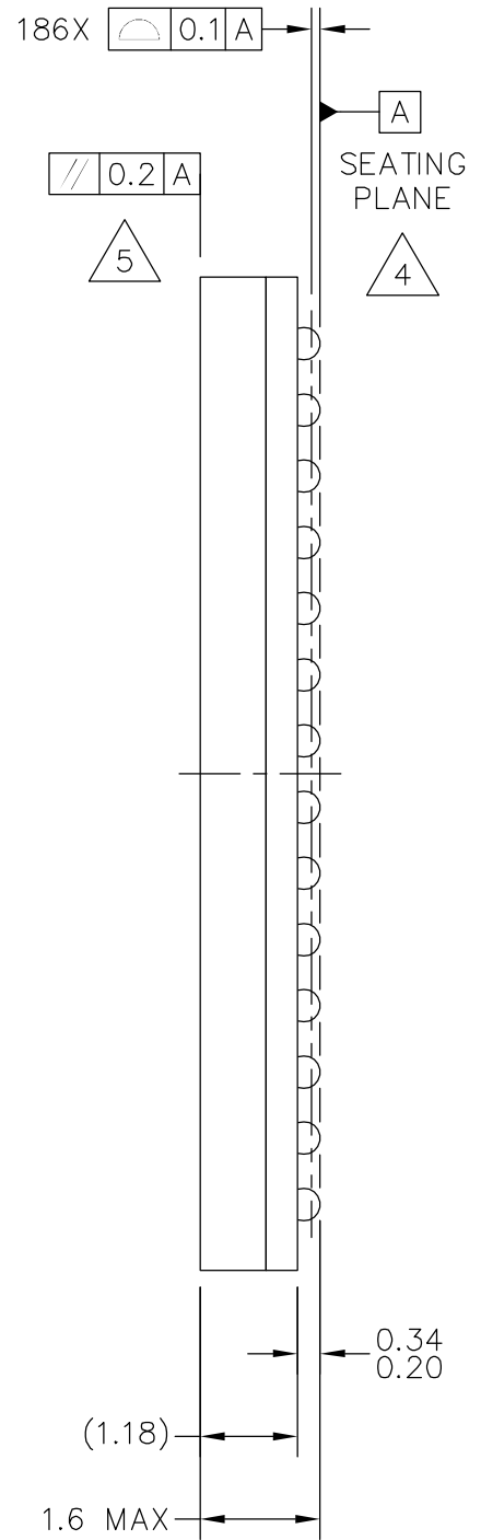
SIDE VIEW
