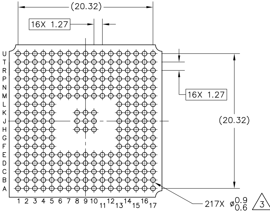
BOTTOM VIEW
