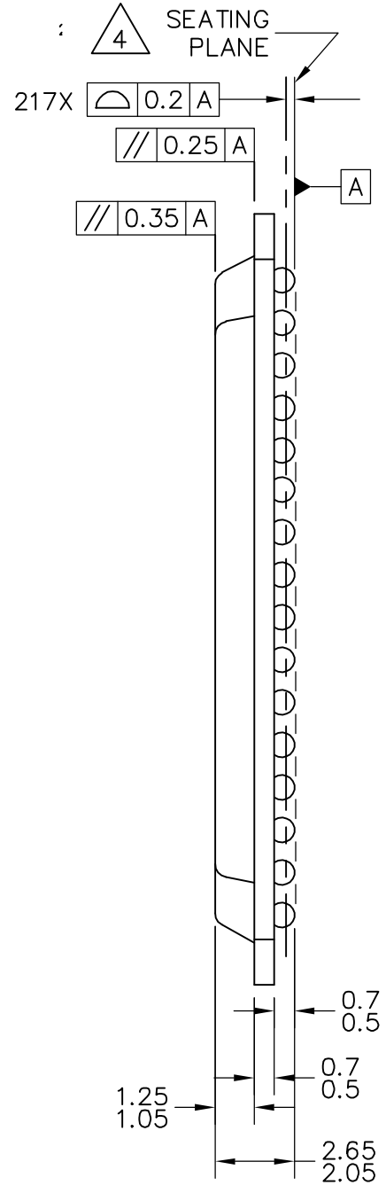
SIDE VIEW
