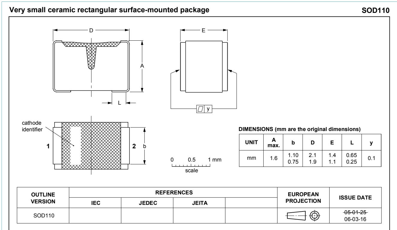
Fig. 1. Package outline SOD2 (SOD110)
