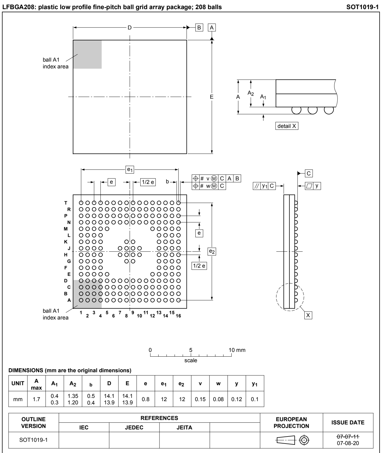
Fig. 1. Package outline LFPGA208 (SOT1019-1)
