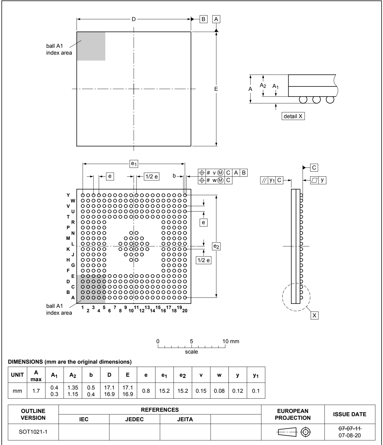
Fig. 1. Package outline LFBGA324 (SOT1021-1)
