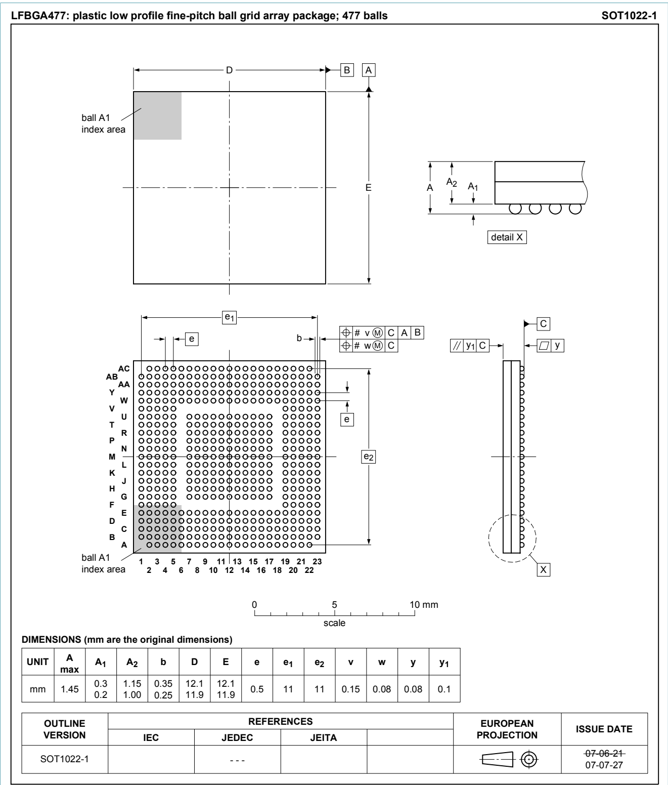
Fig. 1. Package outline LFBGA477 (SOT1022-1)
