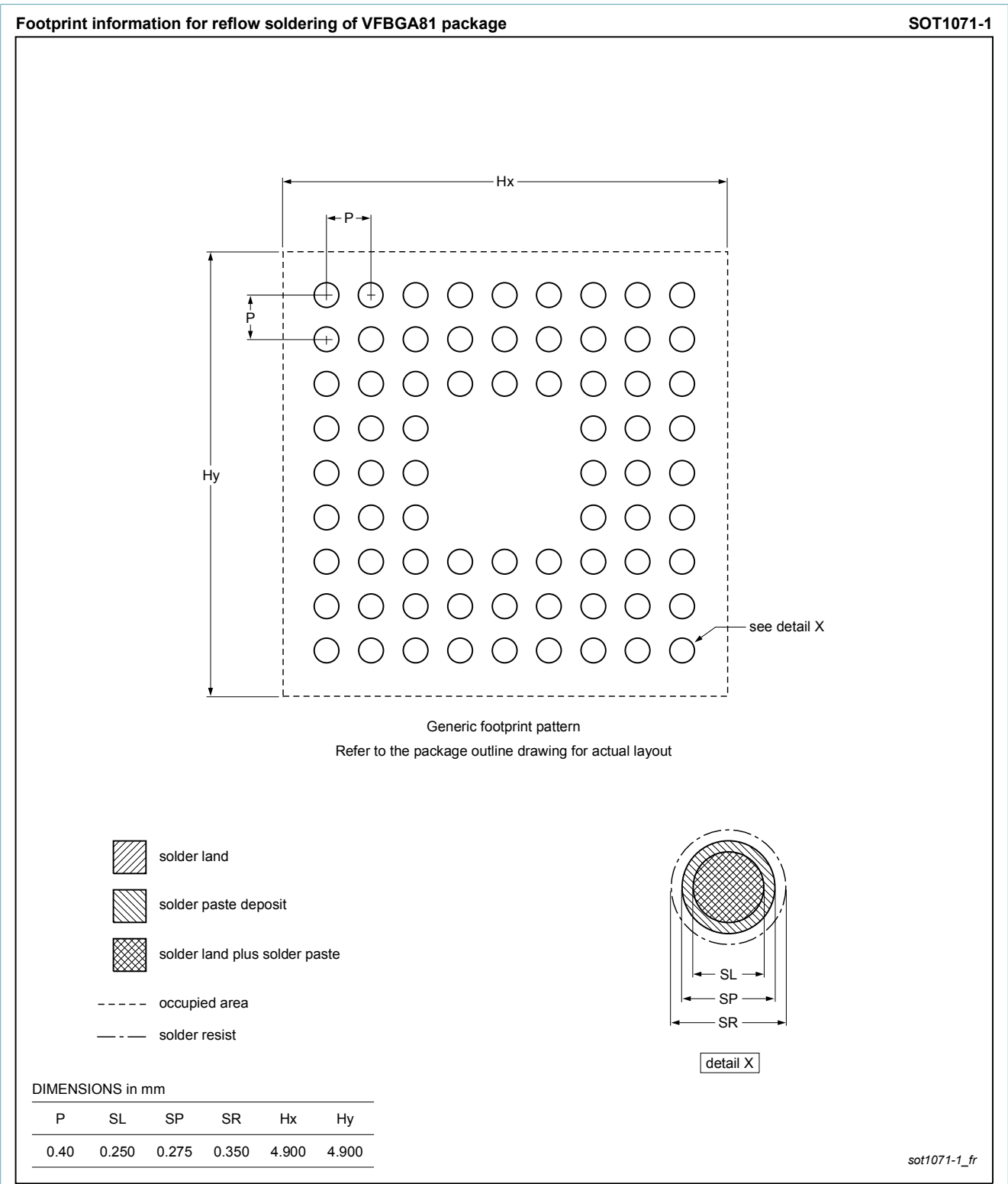
Fig. 2. Reflow soldering footprint for VFBGA81 (SOT1071-1)
