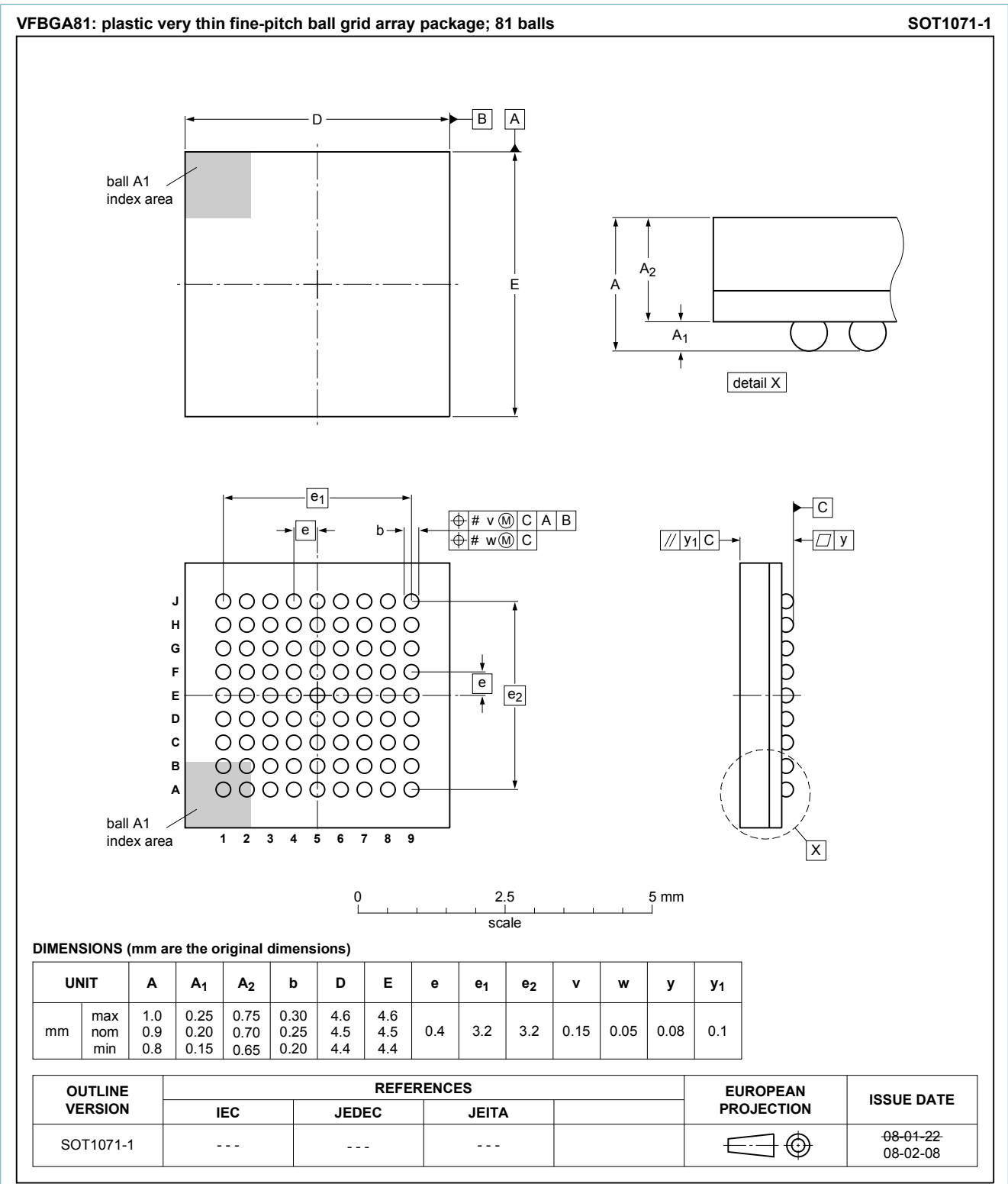
Fig. 1. Package outline VFBGA81 (SOT1071-1)
