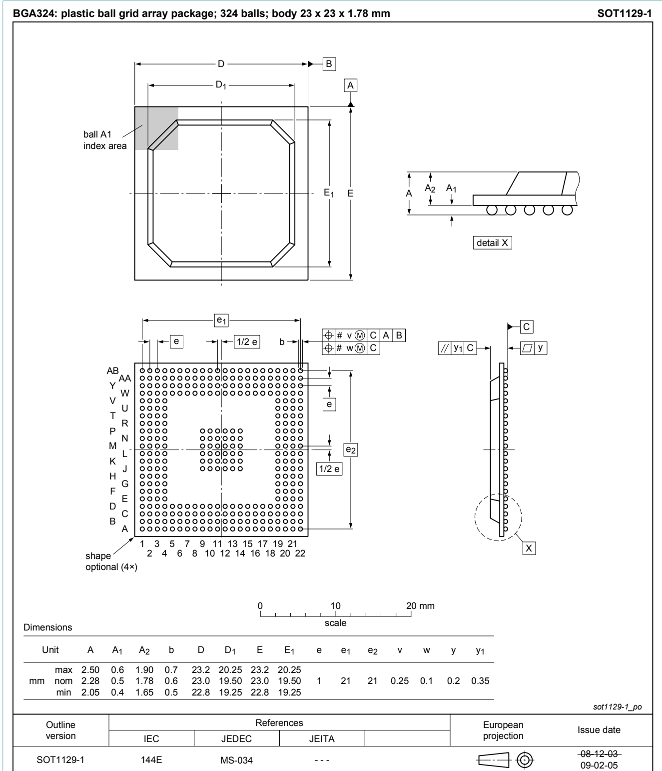
Fig. 1. Package outline BGA324 (SOT1129-1)
