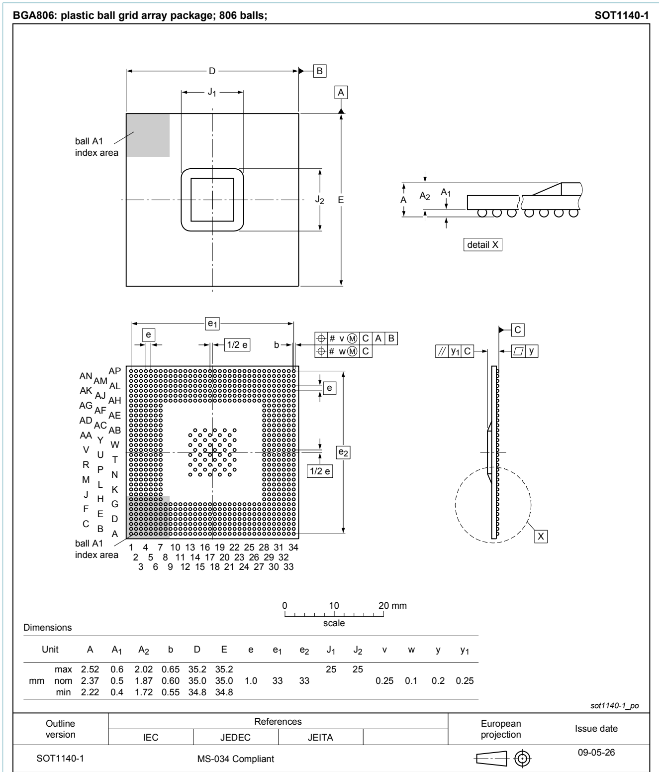
Fig. 1. Package outline BGA806 (SOT1140-1)
