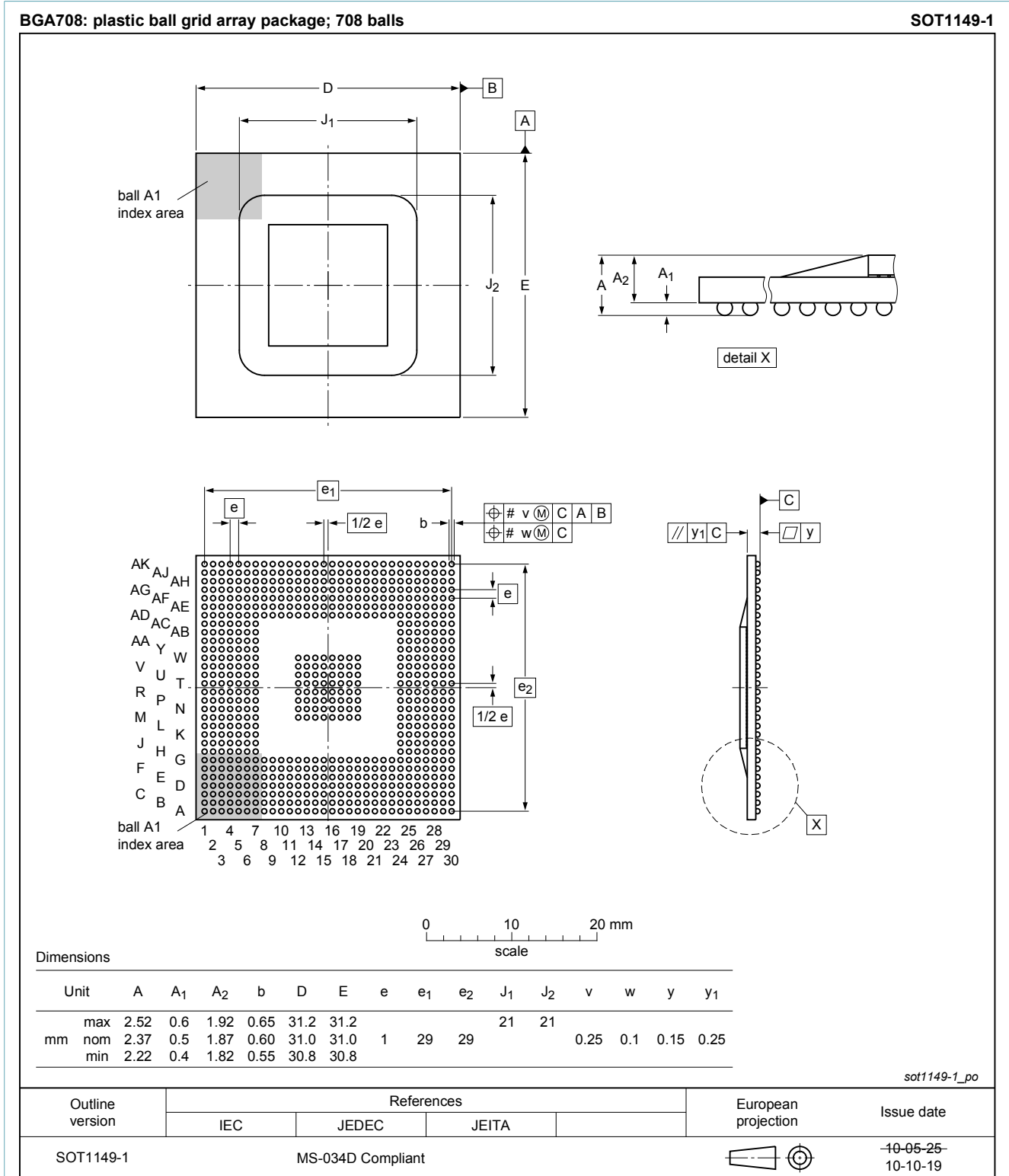
Fig. 1. Package outline BGA708 (SOT1149-1)
