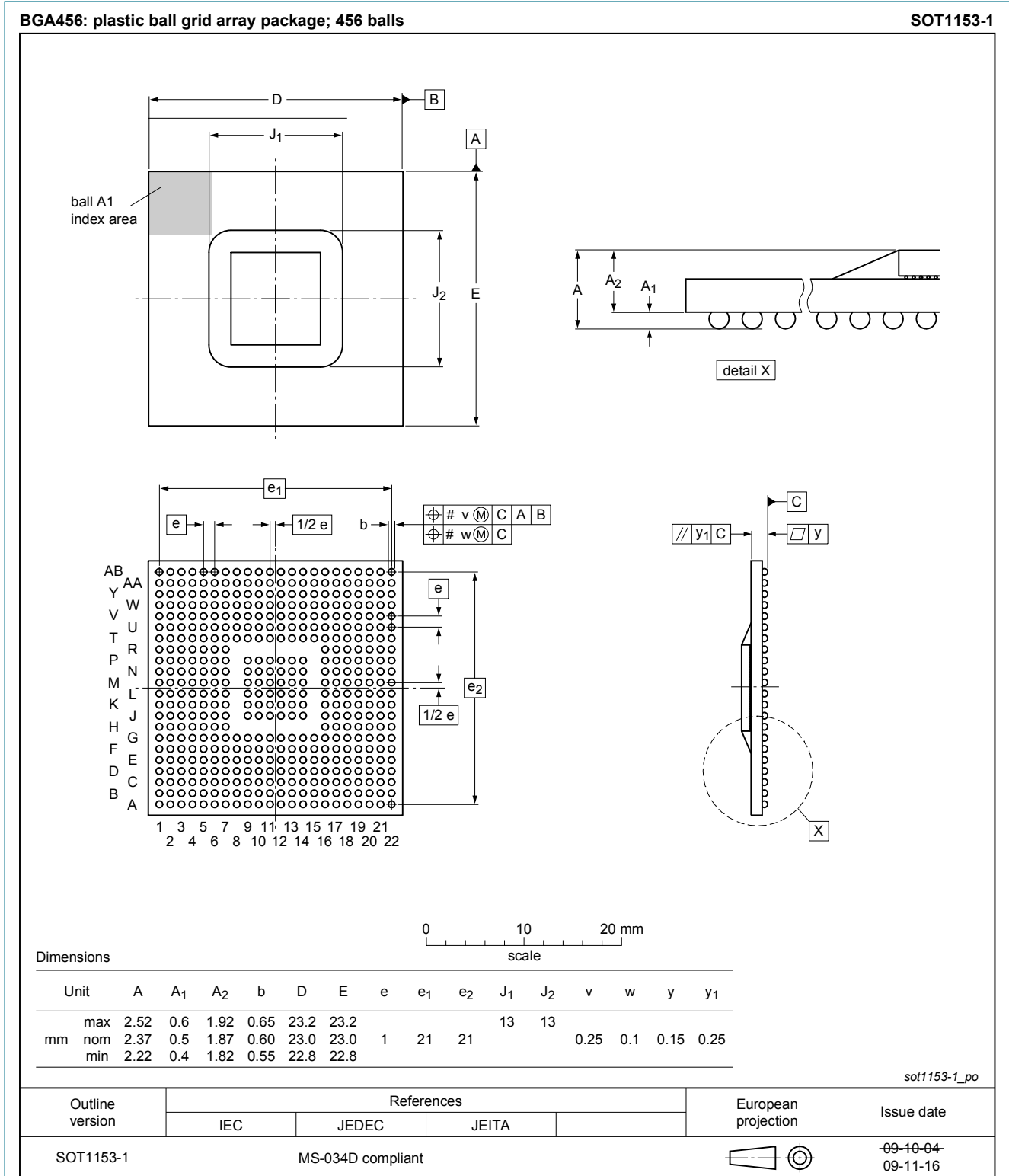
Fig. 1. Package outline BGA456 (SOT1153-1)
