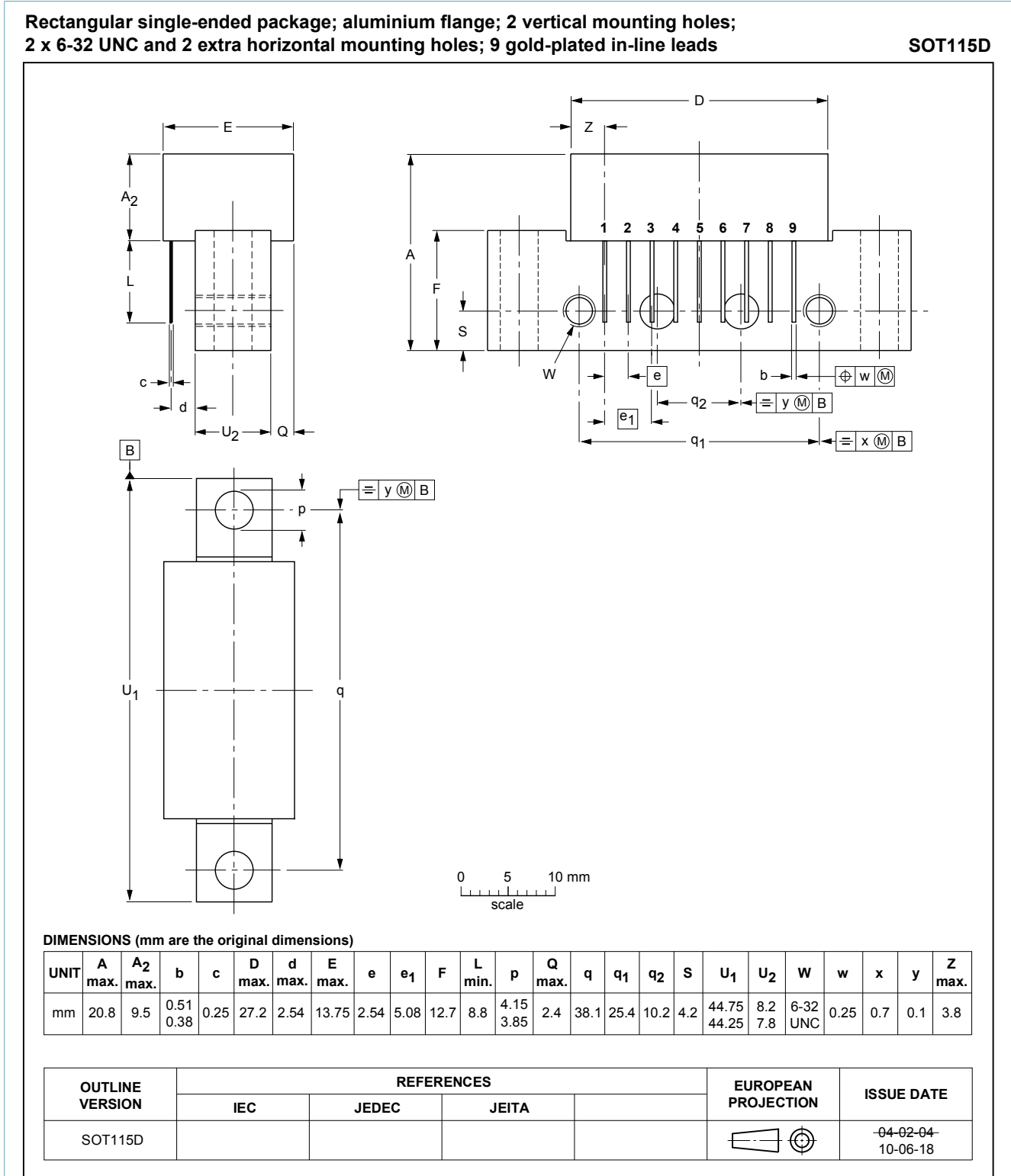
Fig. 1. Package outline SFM9 (SOT115D)
