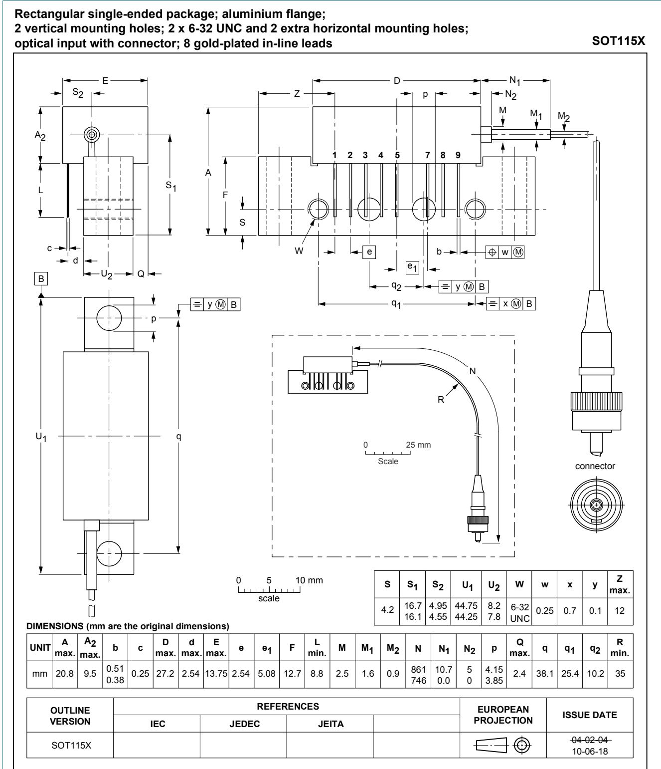
Figure 1. Package outline SFO8 (SOT115X)
