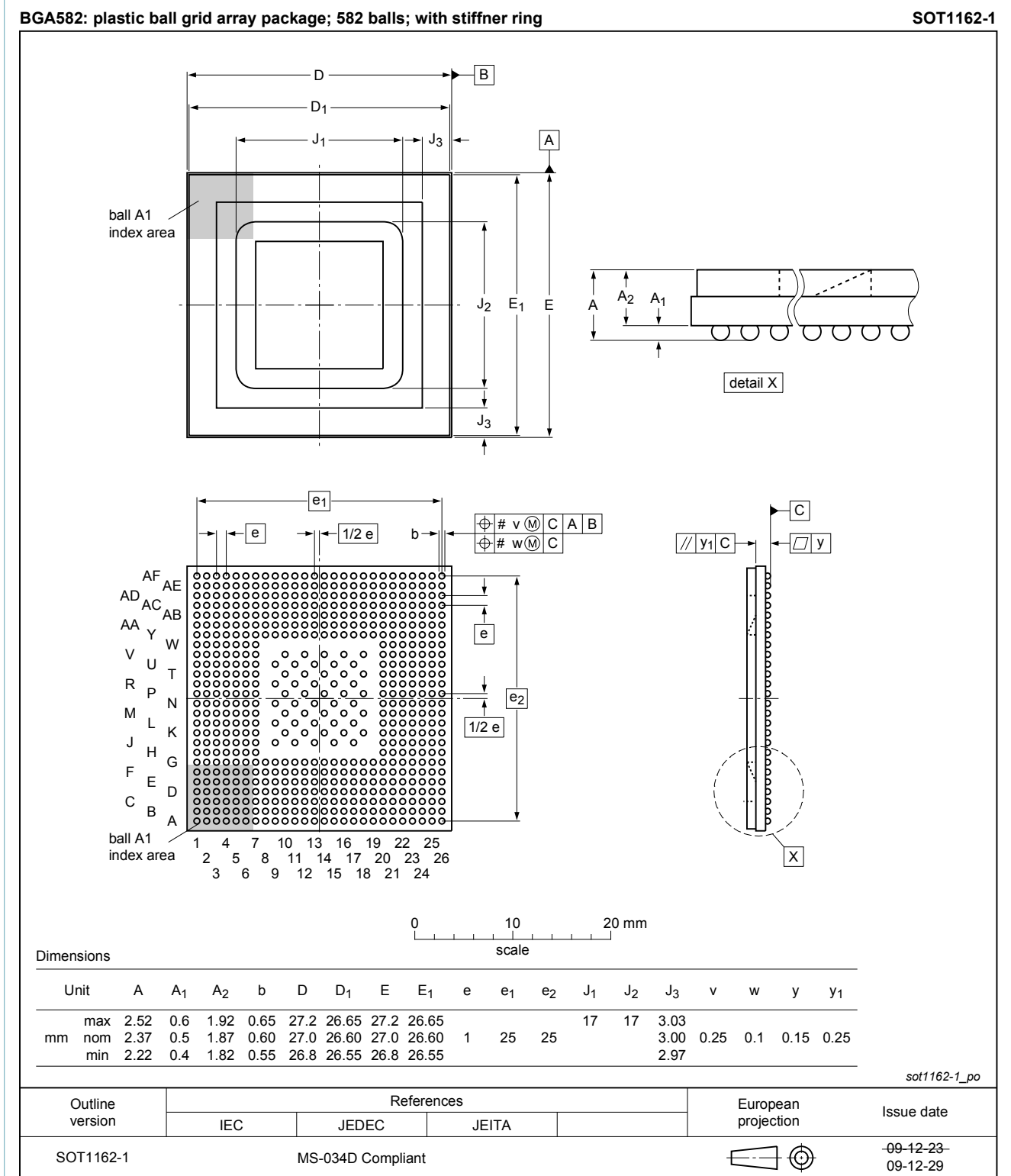
Fig. 1. Package outline BGA582 (SOT1162-1)
