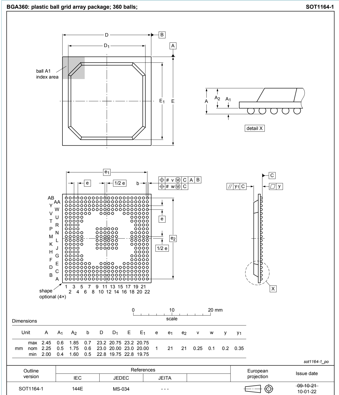
Fig. 1. Package outline BGA360 (SOT1164-1)
