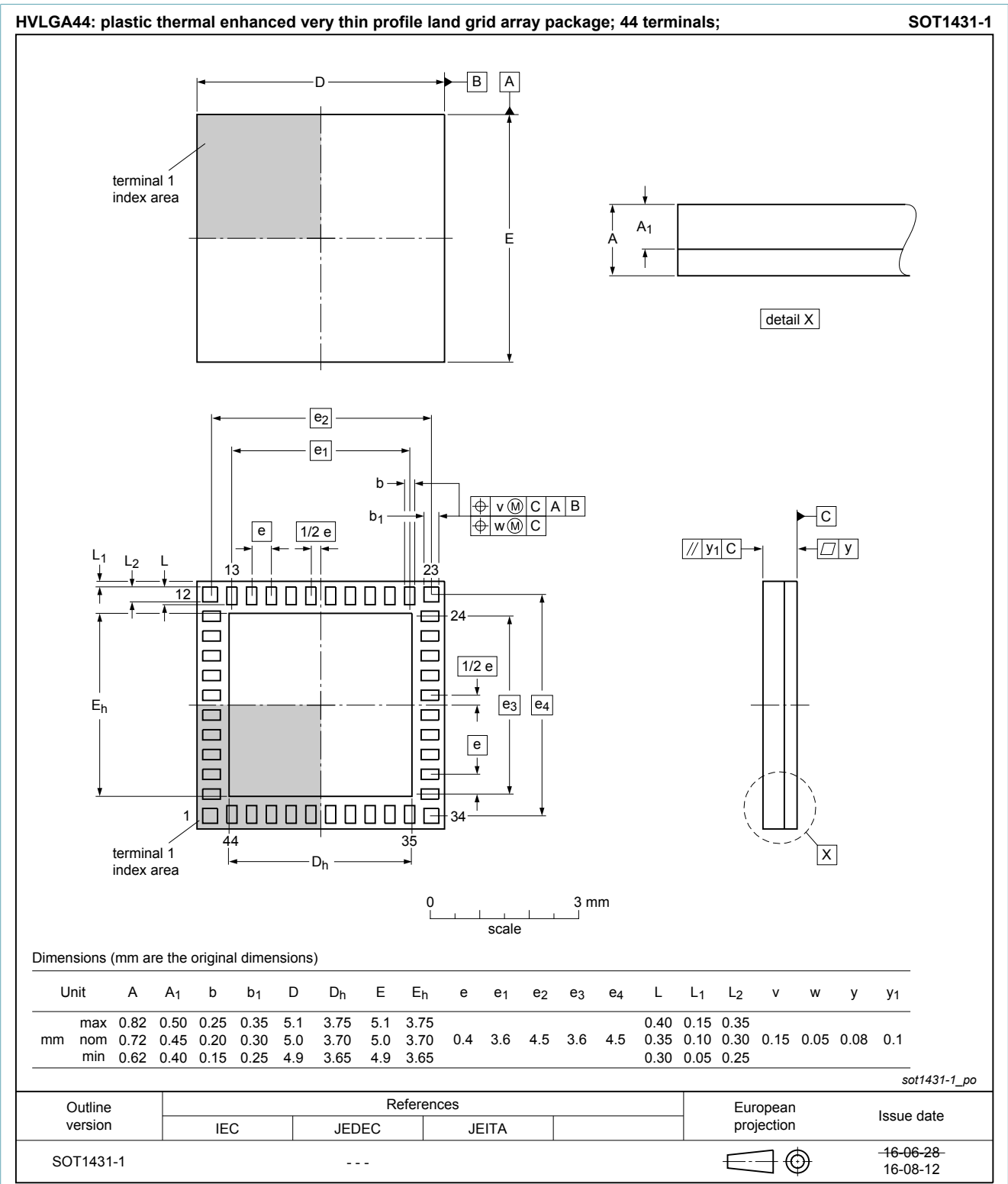
Fig. 1. Package outline HVLGA44 (SOT1431-1)
