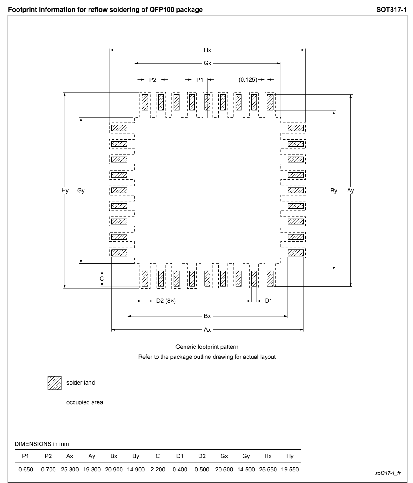
Fig. 2. Reflow soldering footprint for QFP100 (SOT317-1)
