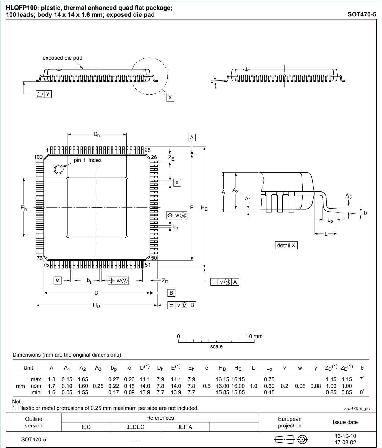
Fig. 1. Package outline HLQFP100 (SOT470-5)
