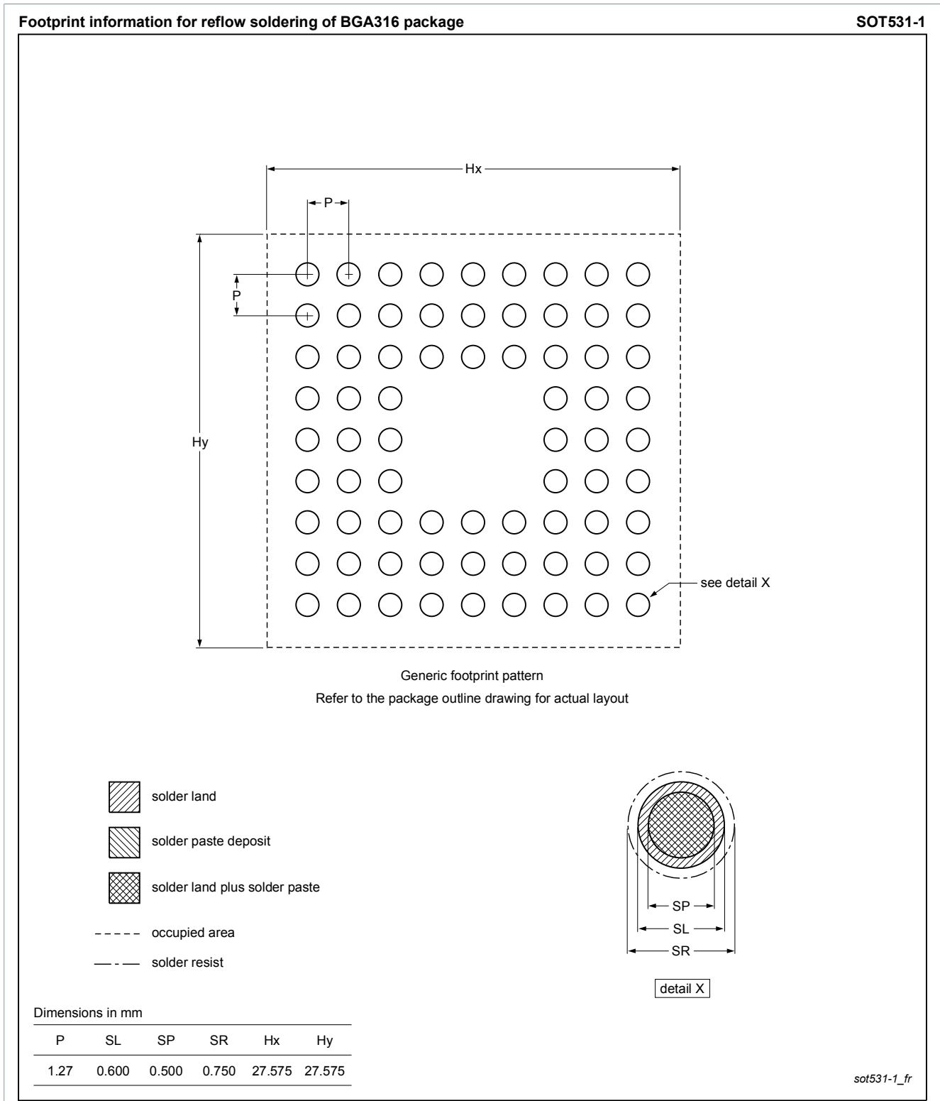
Fig. 2. Reflow soldering footprint for BGA316 (SOT531-1)
