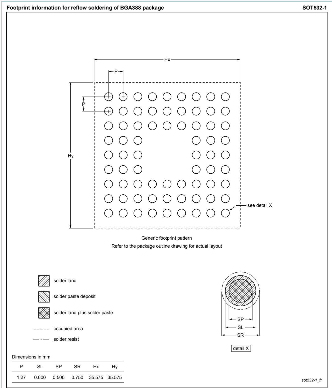
Fig. 2. Reflow soldering footprint for BGA388 (SOT532-1)
