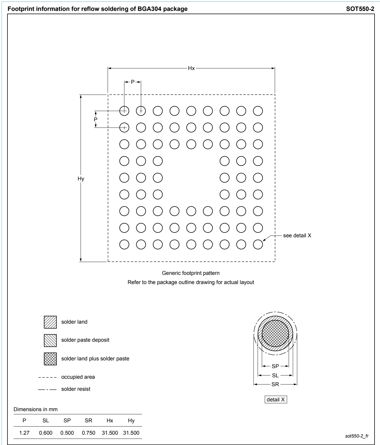
Fig. 2. Reflow soldering footprint for BGA304 (SOT550-2)
