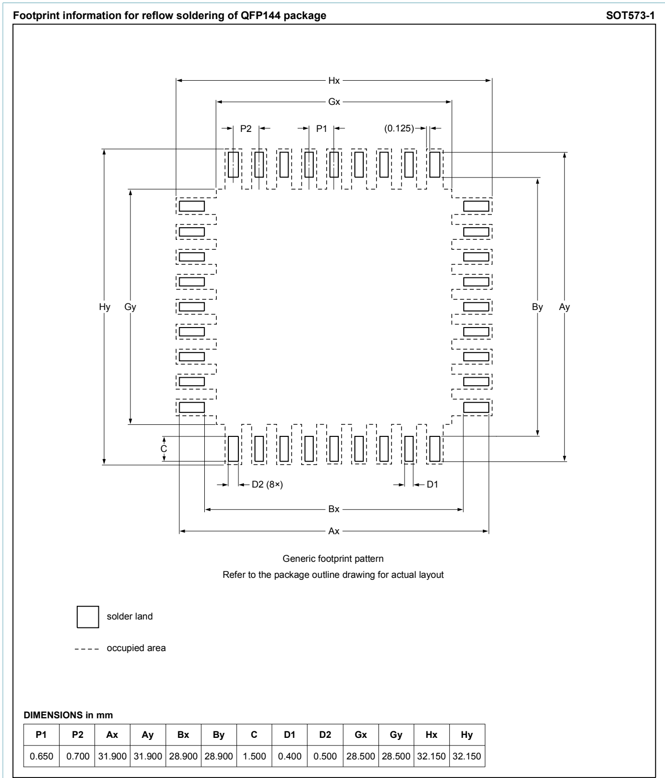
Fig. 2. Reflow soldering footprint for QFP144 (SOT573-1)
