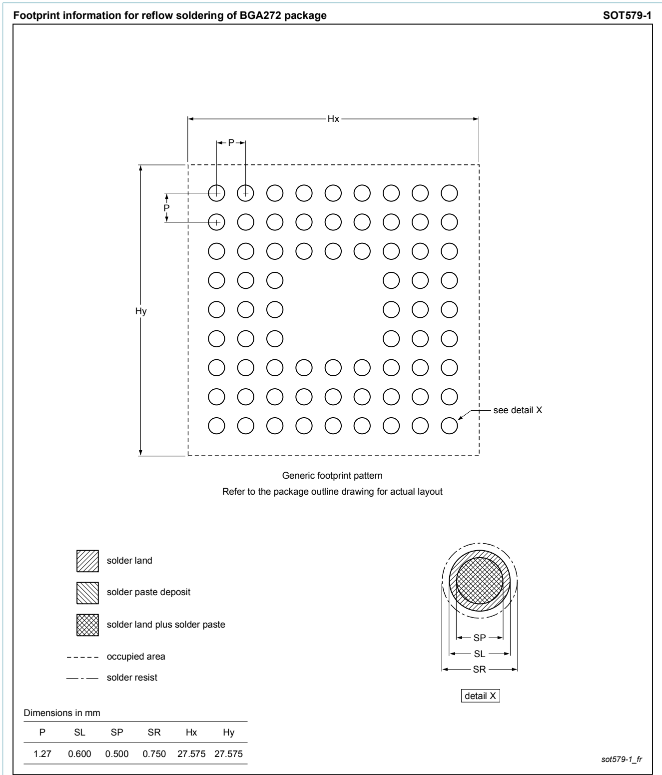
Fig. 2. Reflow soldering footprint for BGA272 (SOT579-1)
