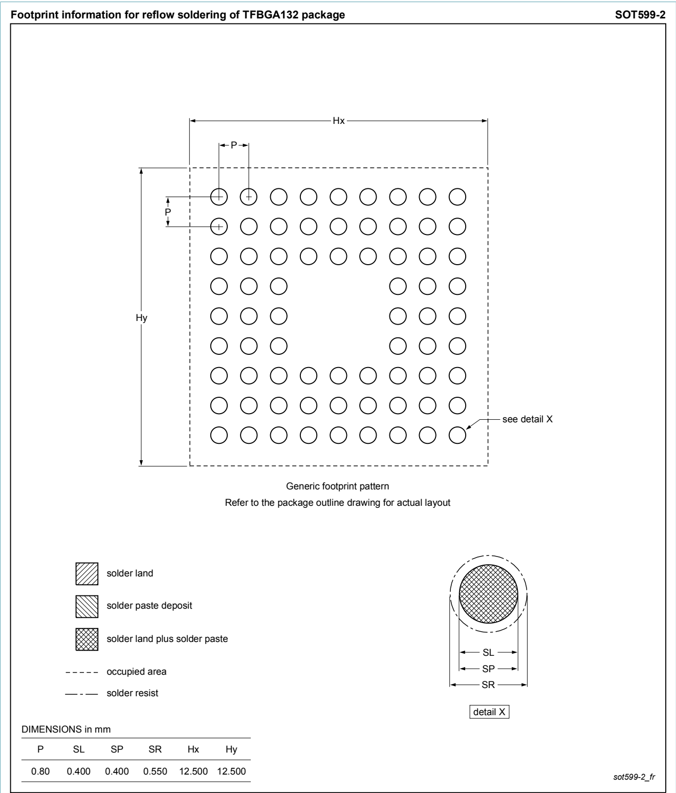
Fig. 2. Reflow soldering footprint for TFBGA132 (SOT599-2)
