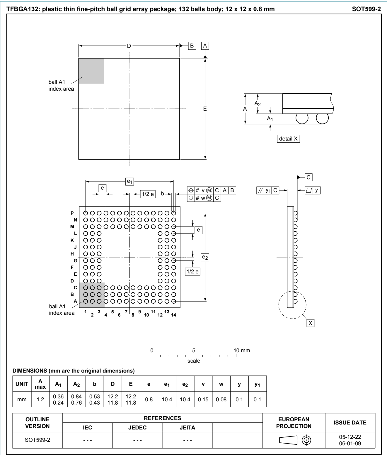
Fig. 1. Package outline TFBGA132 (SOT599-2)
