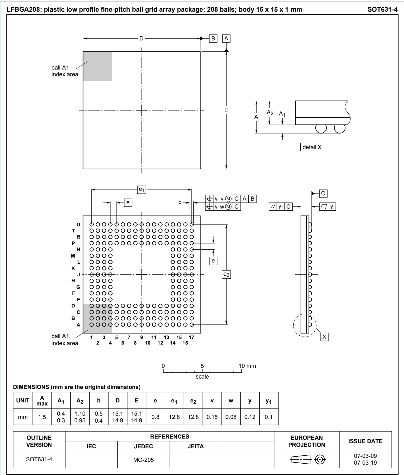
Fig. 1. Package outline LFBGA208 (SOT631-4)
