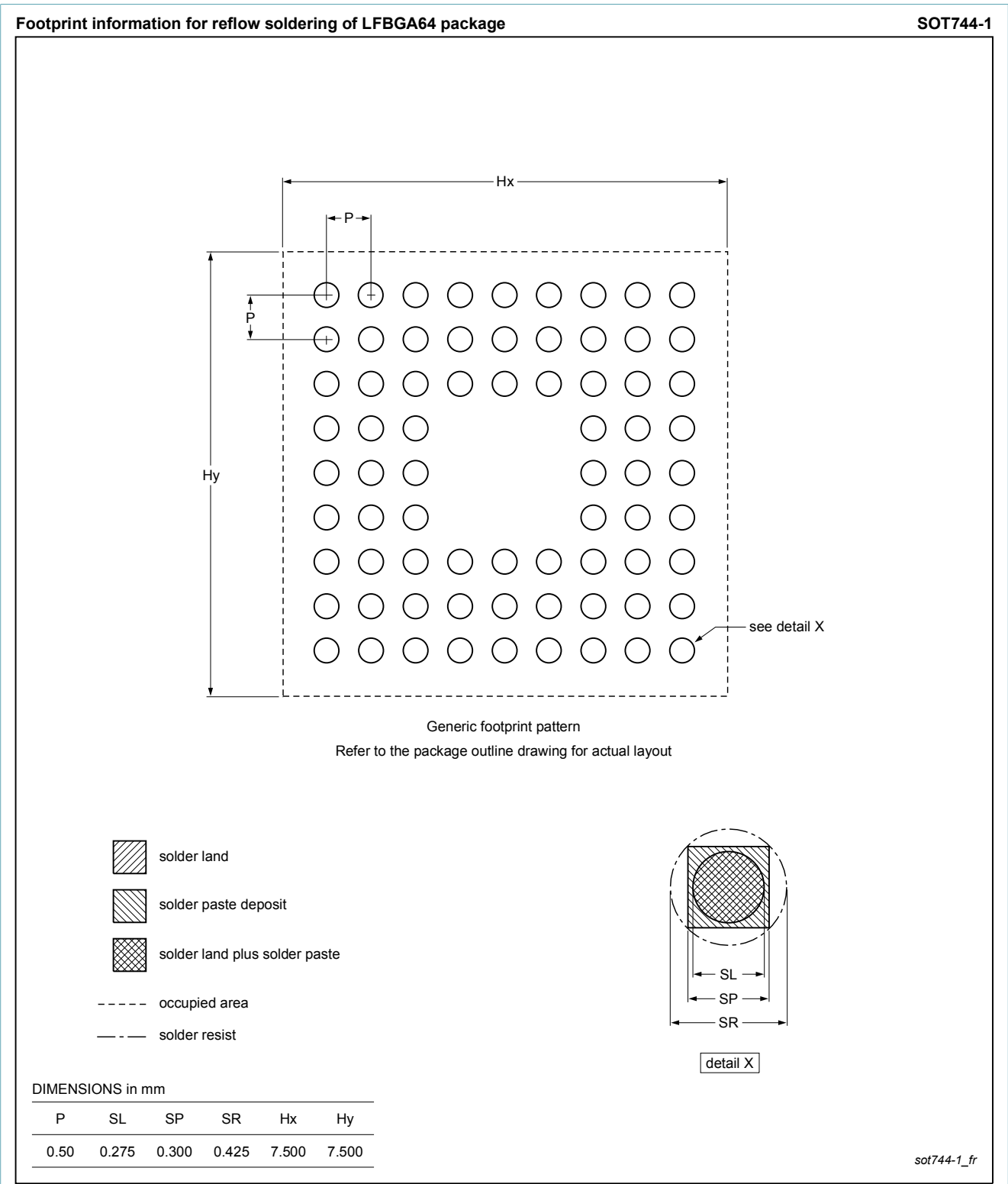
Fig. 2. Reflow soldering footprint for LFBGA64 (SOT744-1)
