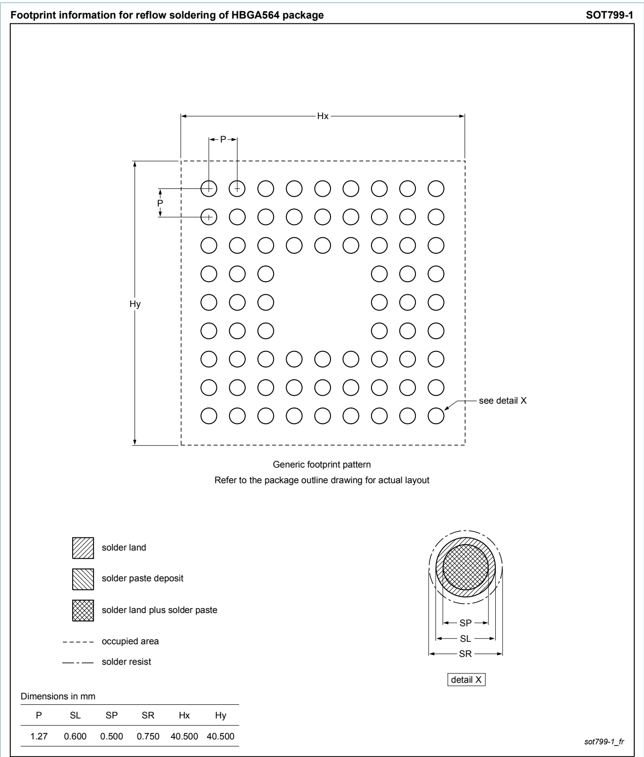
Fig. 2. Reflow soldering footprint for HBGA564 (SOT799-1)
