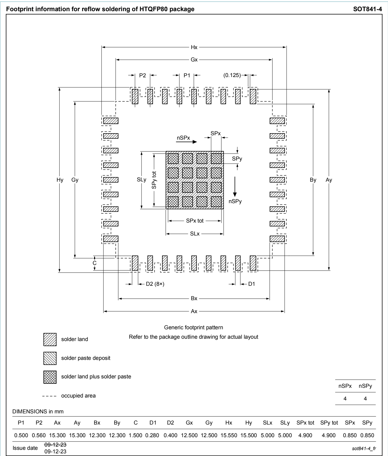
Fig. 2. Reflow soldering footprint for HTQFP80 (SOT841-4)
