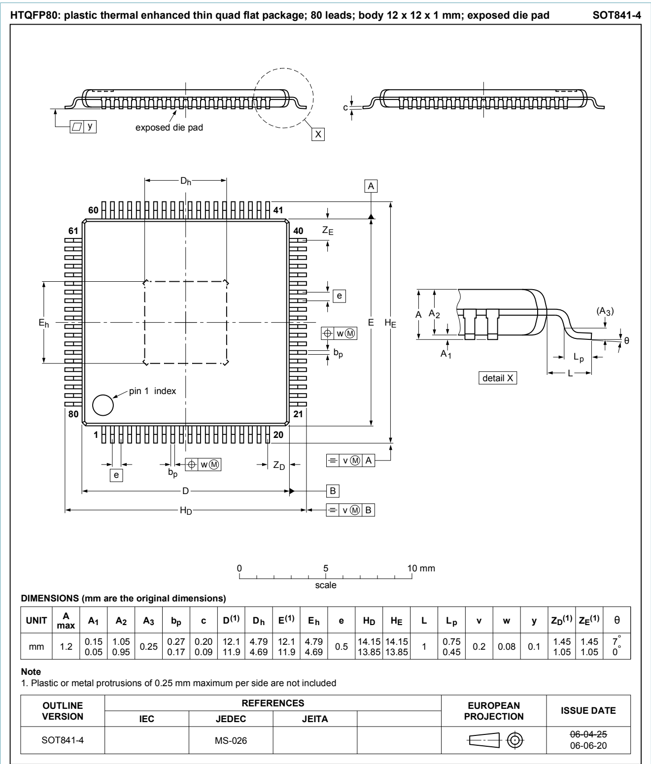
Fig. 1. Package outline HTQFP80 (SOT841-4)
