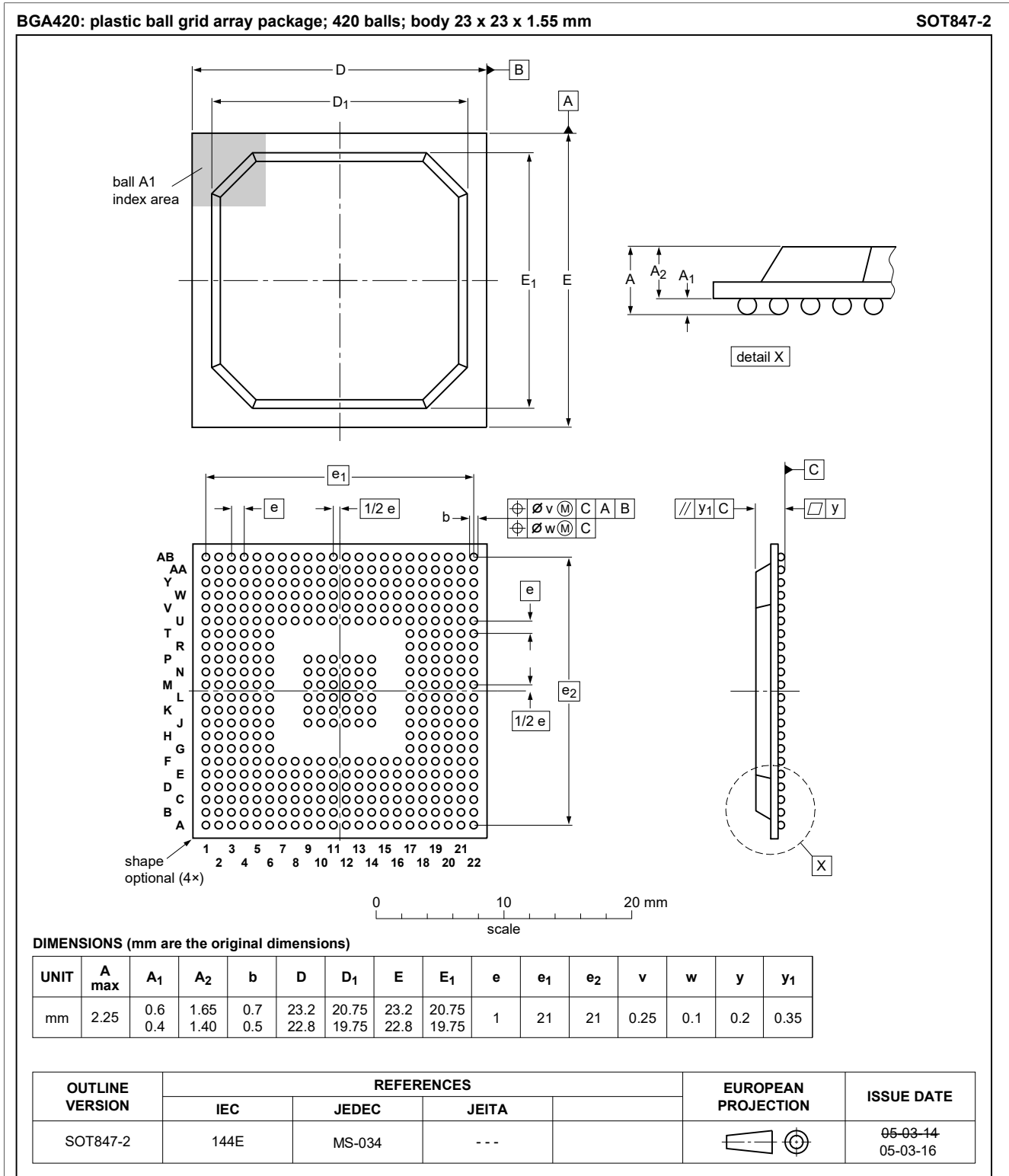
Figure 1. Package outline BGA420 (SOT847-2)
