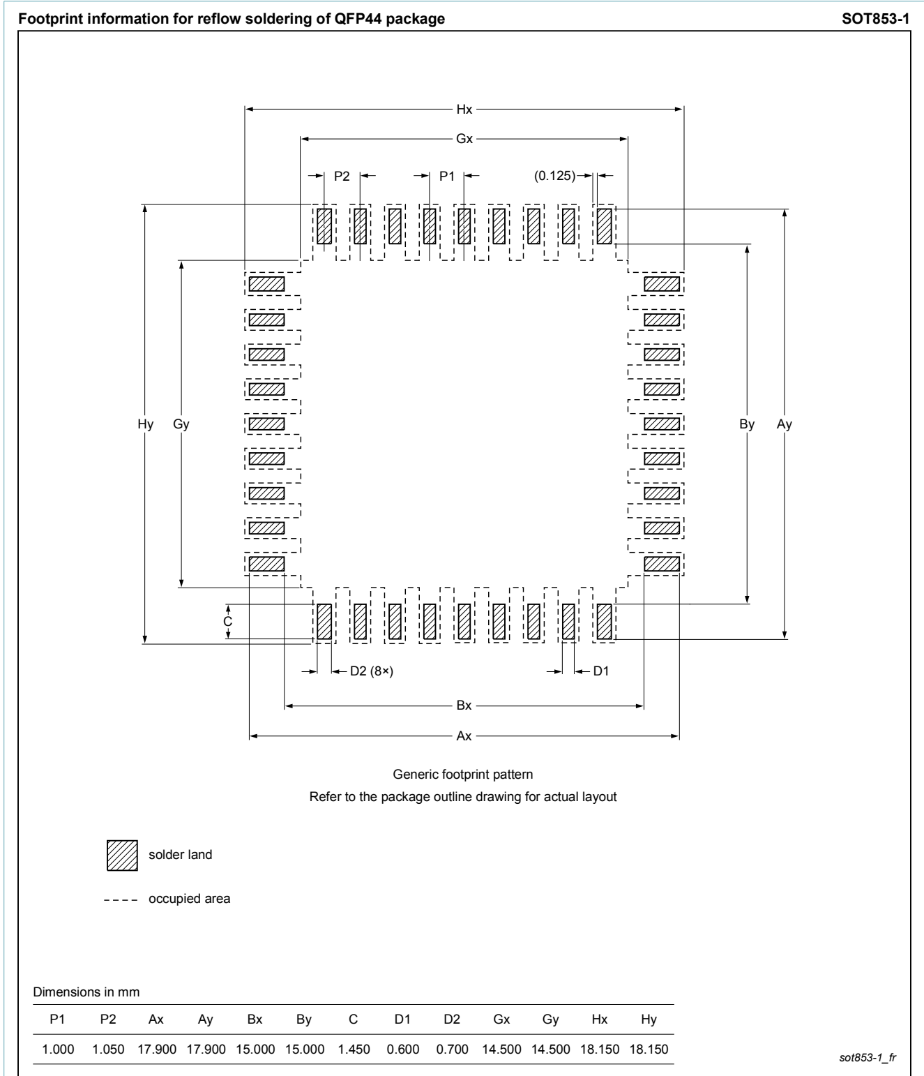
Fig. 2. Reflow soldering footprint for QFP44 (SOT853-1)
