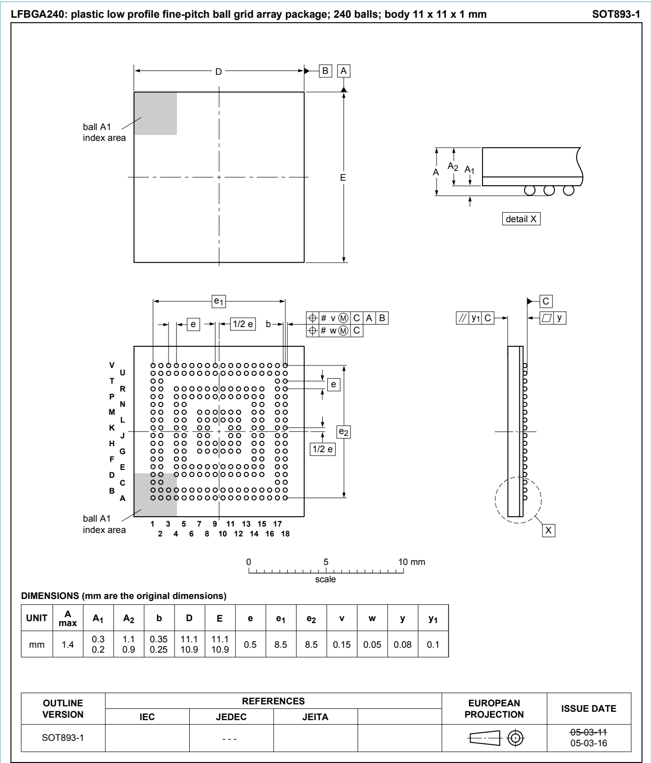
Fig. 1. Package outline LFBGA240 (SOT893-1)
