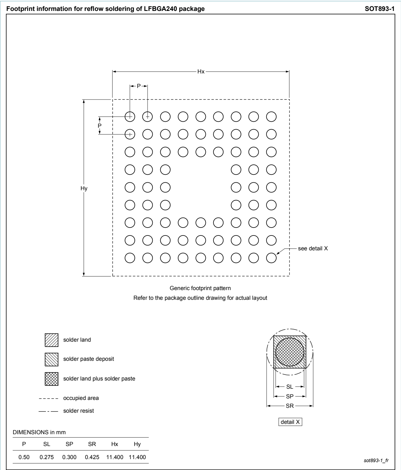
Fig. 2. Reflow soldering footprint for LFBGA240 (SOT893-1)
