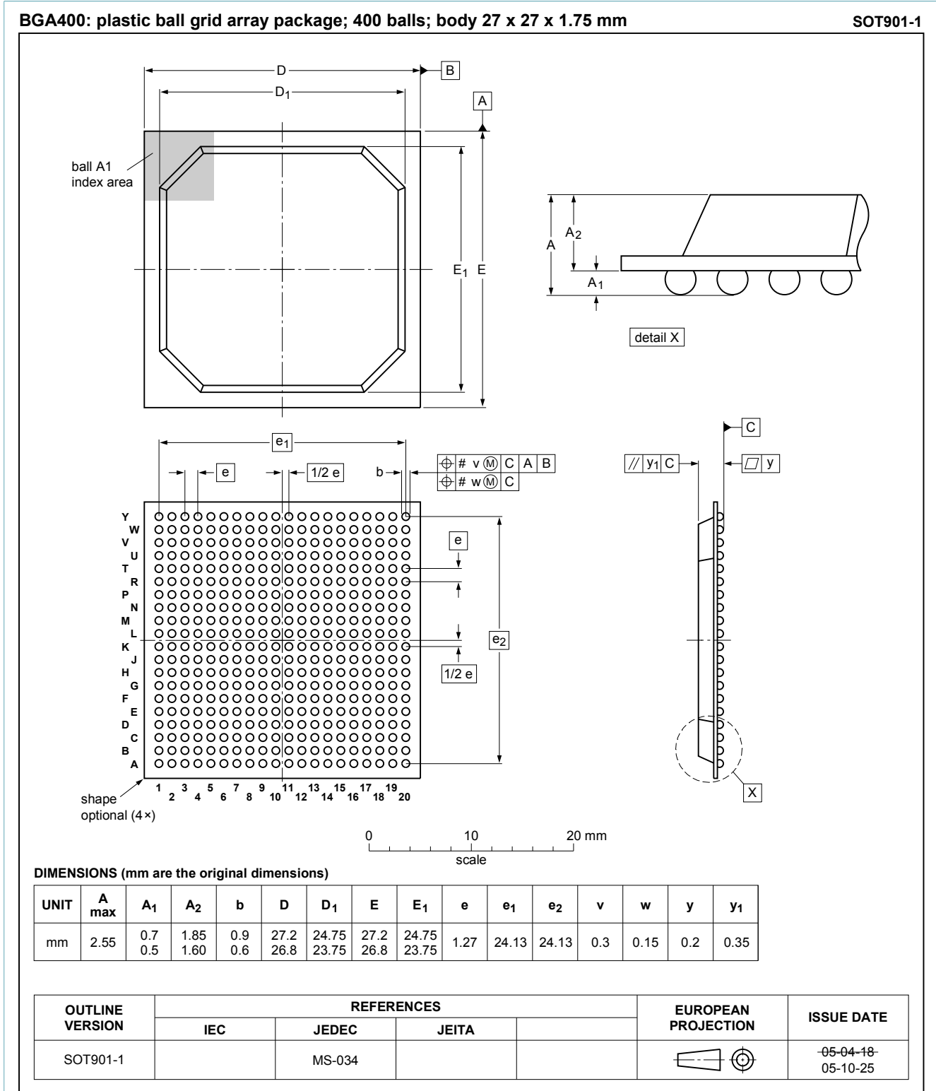
Fig. 1. Package outline BGA400 (SOT901-1)
