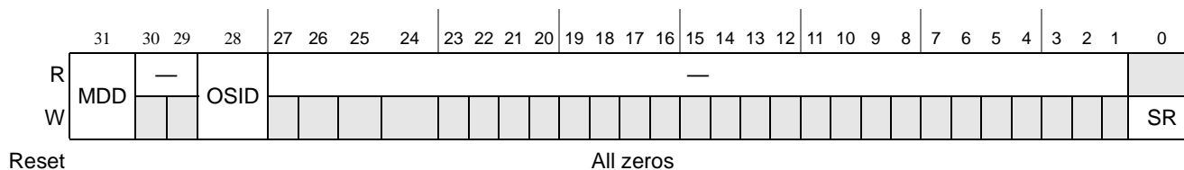
Figure 16-145. Message Unit Mode Register (MUMR)
