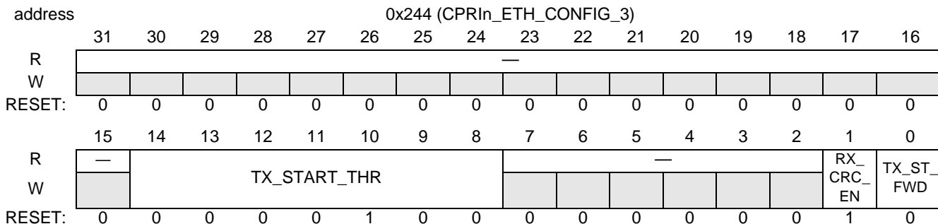
Figure 18-67. CPRIn_ETH_CONFIG_3
