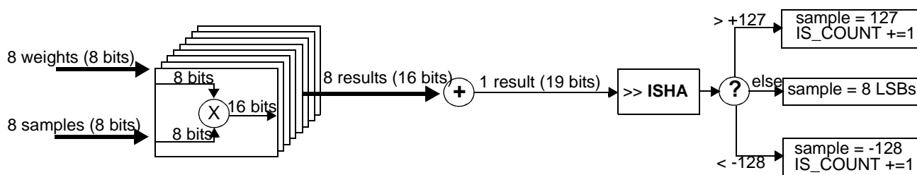
Figure 26-118. Internal Interpolation Calculation Flow
