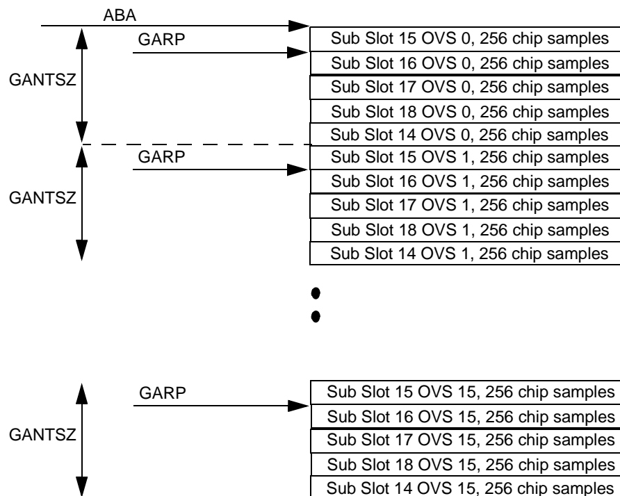
Figure 26-111. Single Antenna Input Data Structure Where GANTSZ=5 , INT\_MODE = 0 , IIL=3
