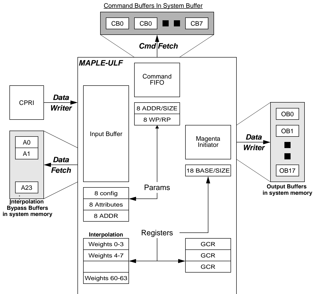
Figure 26-128. ULF Data Structure
