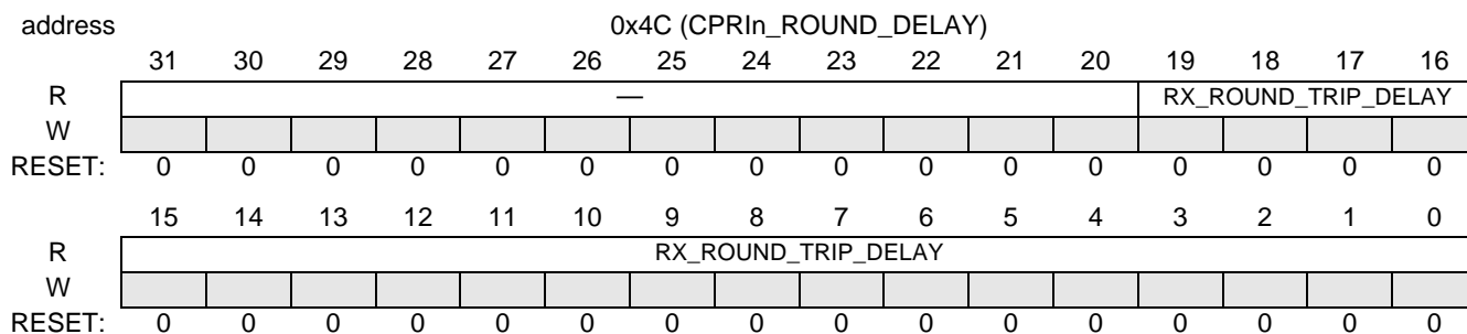
Figure 18-44. CPRIn_ROUND_DELAY
