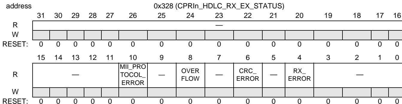
Figure 18-73. CPRIn_HDLC_RX_EX_STATUS
