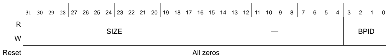
Figure 16-59. Inbound Block m Type9 Classification n Data Buffer Pool Register (IB m T9C n DBPR)
