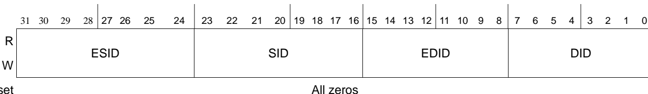
Figure 16-47. Inbound Block m Type8 Classification n Rule Mask Register 0 (IB m T8C n RMR0)
