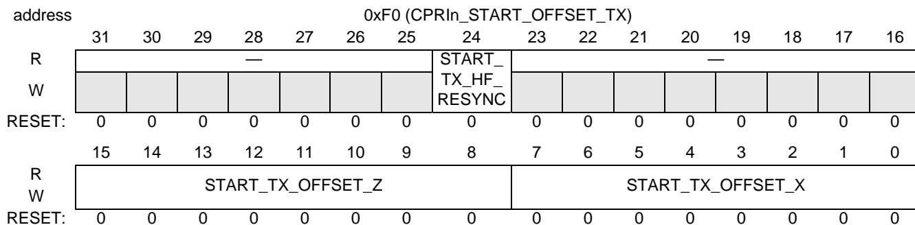
Figure 18-56. CPRIn_START_OFFSET_TX
