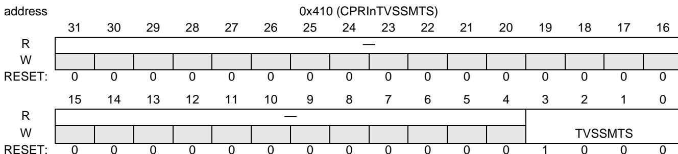
Figure 18-80. CPRInTVSSMTS
