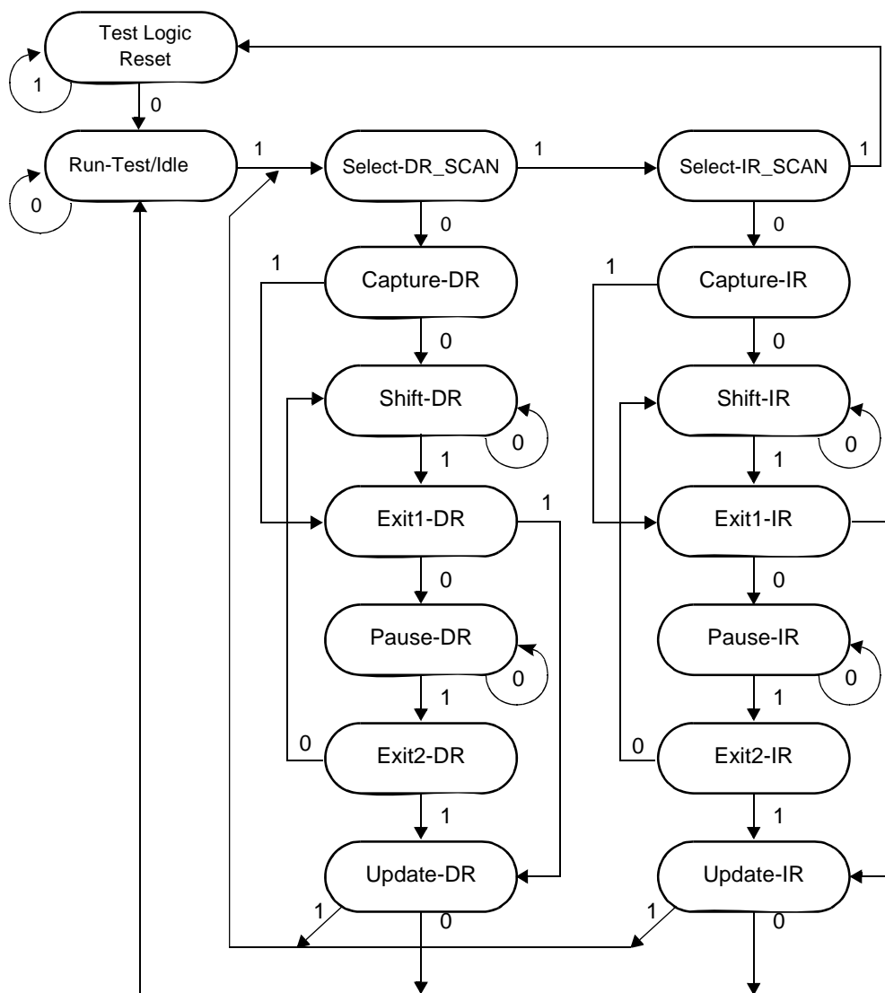
Figure 25-2. TAP Controller State Machine
