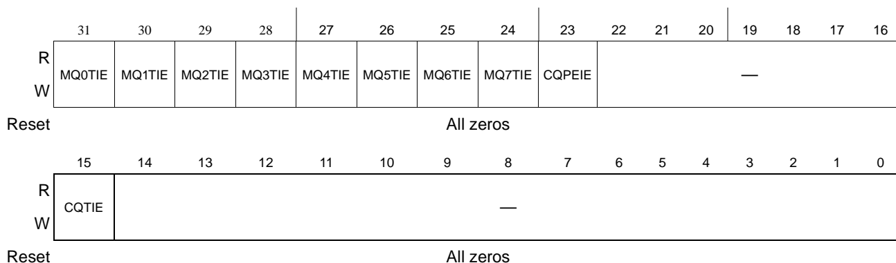
Figure 16-89. Outbound Block m Message Queue Interrupt Enable Register (OB m MQIER)
