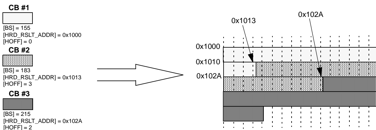
Figure 26-34. Concatenating Hard outputs
