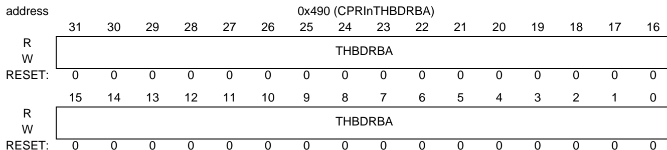
Figure 18-94. CPRInTHBDRBA
