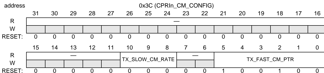
Figure 18-41. CPRIn_CM_CONFIG
