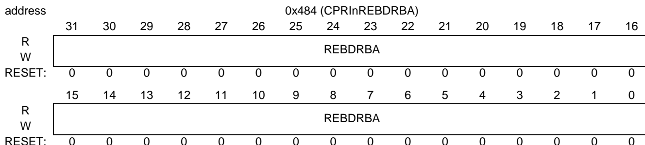
Figure 18-91. CPRInREBDRBA
