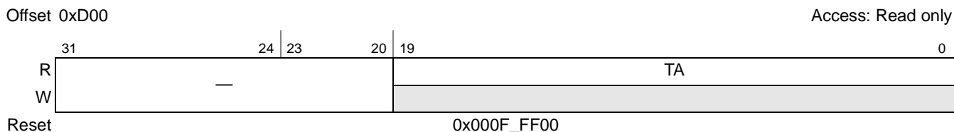
Figure 17-37. PCI Express MSI Inbound Translation Address Register (PEXMSIITAR)
