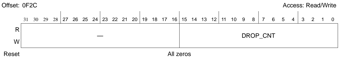
Figure 16-150. Message Unit T8 Drop Counter Registers (MUT8DCR)
