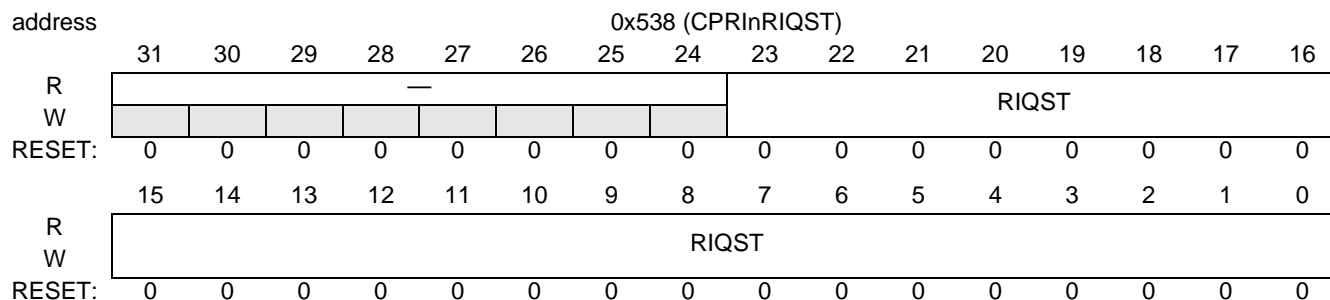
Figure 18-122. CPRInRIQST
