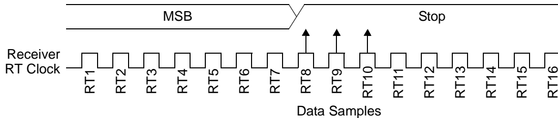
Figure 20-17. Slow Data
