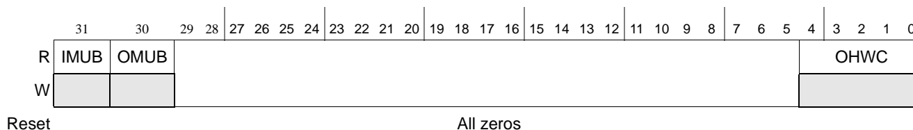
Figure 16-146. Message Unit Status Register (MUSR)
