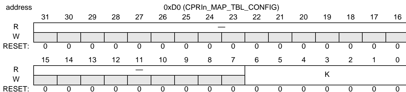
Figure 18-53. CPRIn_MAP_TBL_CONFIG
