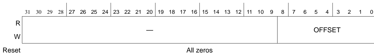
Figure 16-70. Inbound Block m Type10 Classification n Data Offset Register (IB m T10C n DOR)
