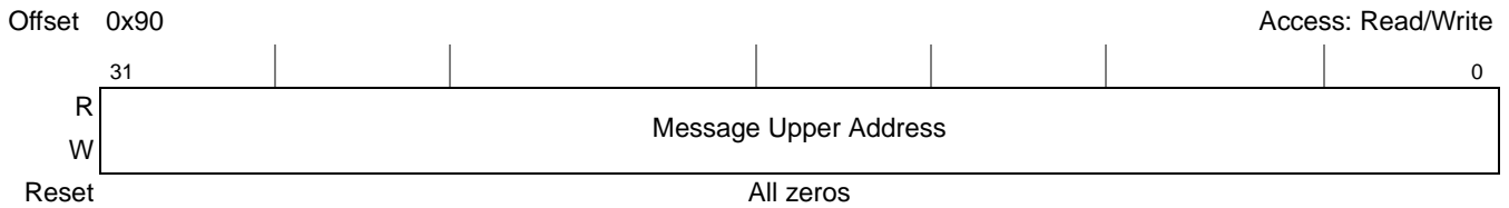
Figure 17-120. PCI Express MSI Message Upper Address Register
