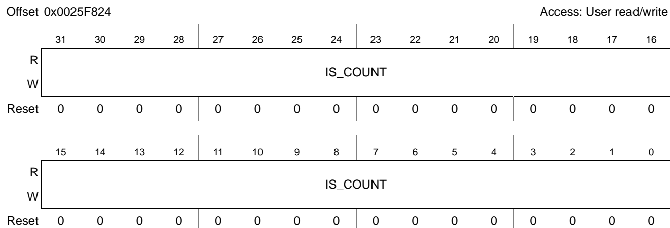
Figure 26-289. CRPE-ULB Interpolation Saturation Counter Status Register
