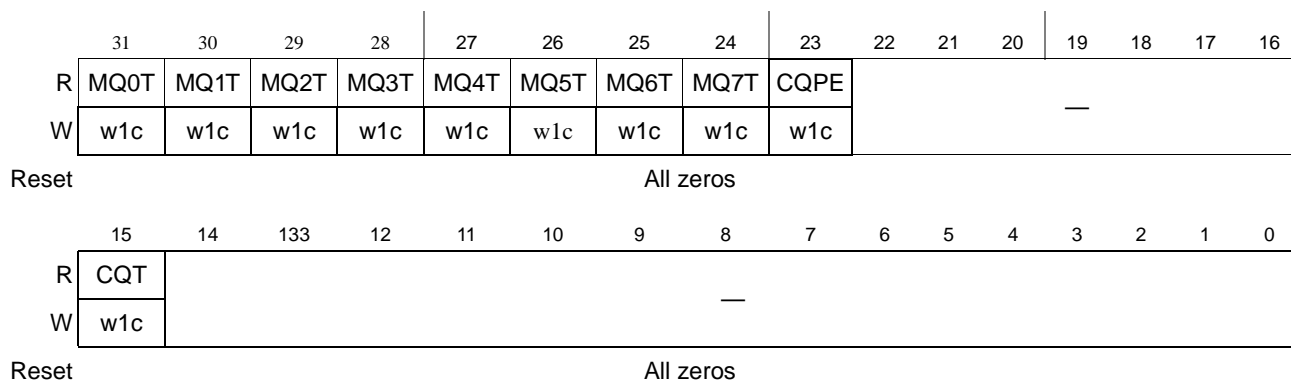
Figure 16-90. Outbound Block m Message Queue Interrupt Detect Register (OB m MQIDR)
