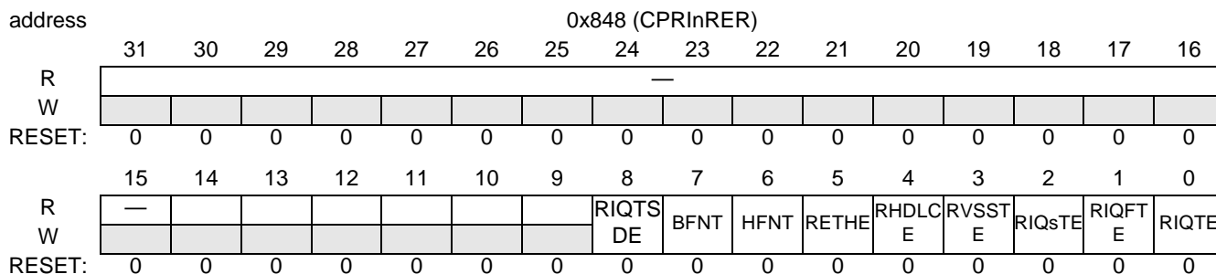
Figure 18-158. CPRInRER
