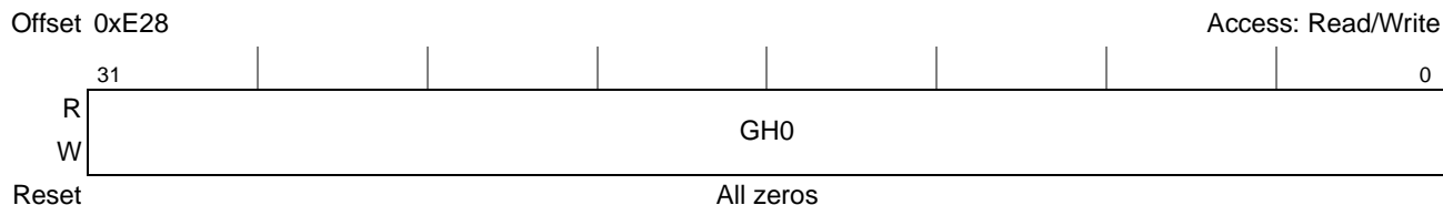
Figure 17-46. PCI Express Error Capture Register 0 (PEX_ERR_CAP_R0) External Source, Inbound Transaction
