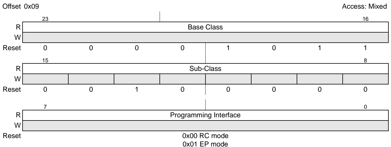
Figure 17-59. PCI Express Class Code Register
