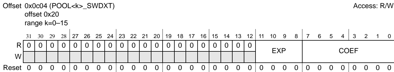
Figure 16-118. S/W Portal Depletion Exit Threshold Register (POOL k _SWDXT)
