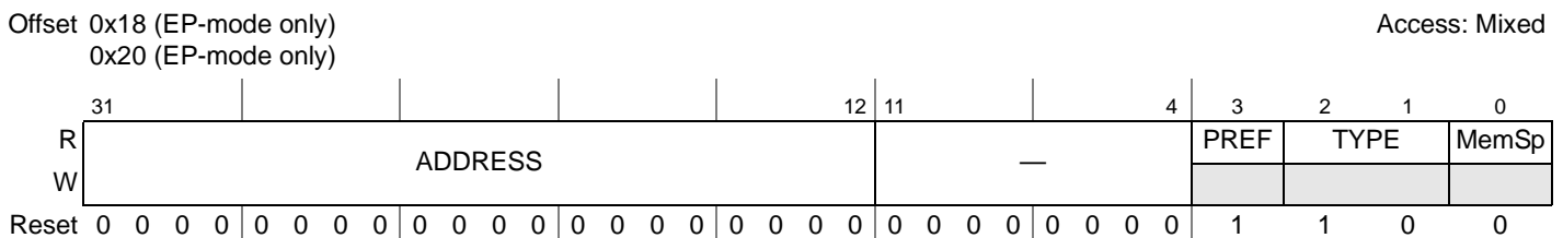
Figure 17-66. 64-Bit Low Memory Base Address Register
