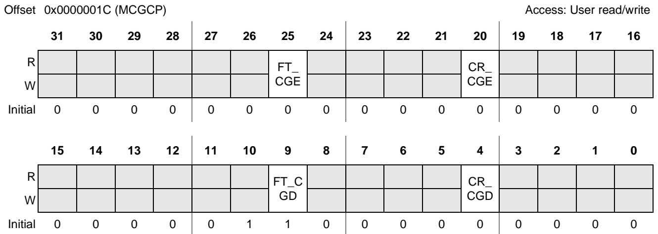
Figure 26-188. MAPLE Clock Gating Control Parameter
