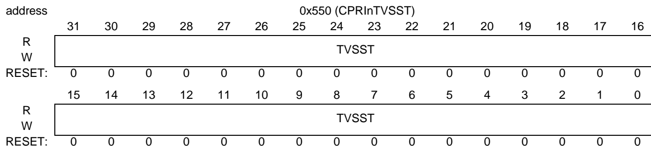
Figure 18-128. CPRInTVSST
