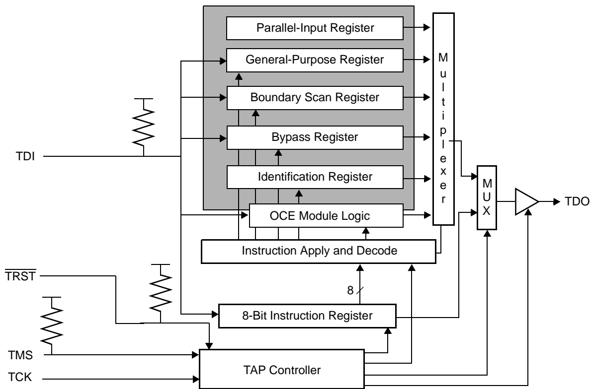
Figure 25-1. Test Logic Block Diagram
