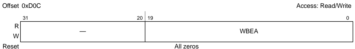
Figure 17-39. PCI Express MSI Inbound Window Base Extended Address Register (PEXMSIIWBEAR)
