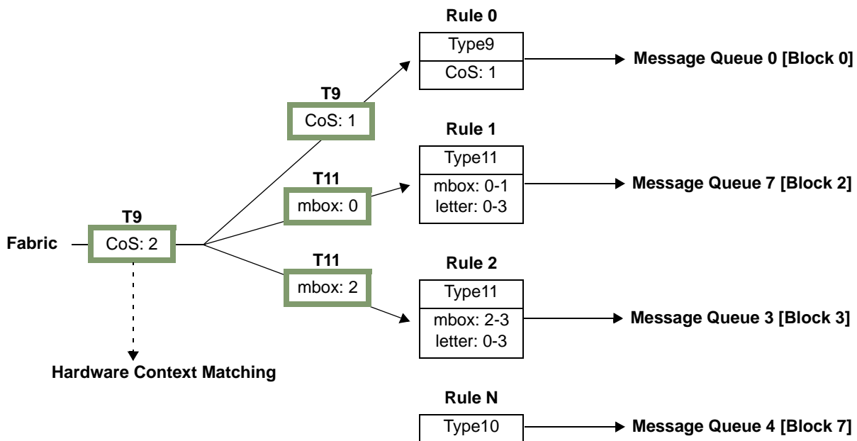
Figure 16-40. Inbound Traffic Classification
