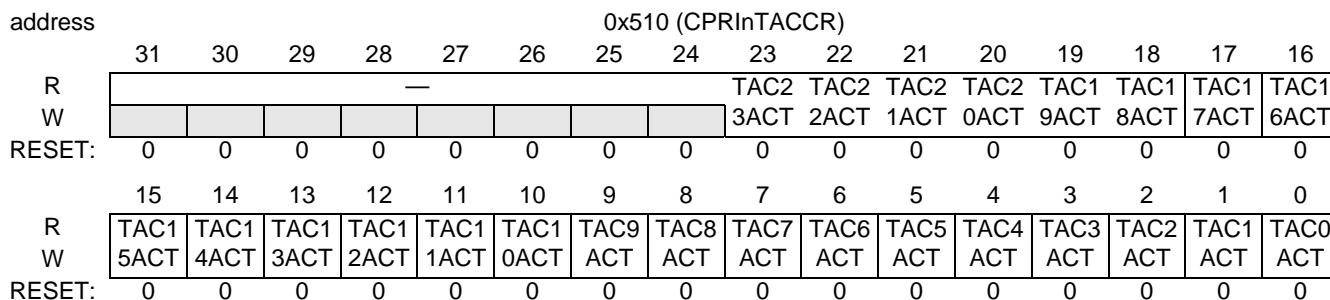
Figure 18-112. CPRInTACCR
