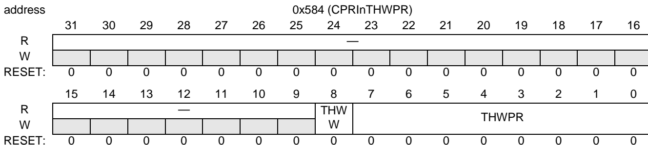
Figure 18-139. CPRInTHWPR
