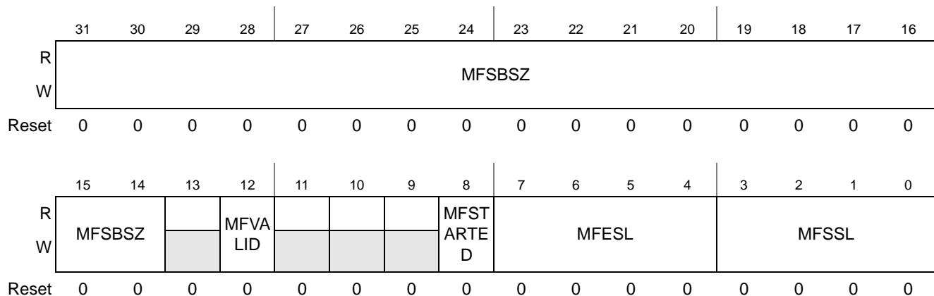
Figure 26-226. MAPLE CRPE-DL Fast Channel <x> Parameter 0
