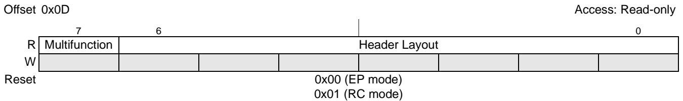
Figure 17-62. PCI Express Bus Latency Timer Register
