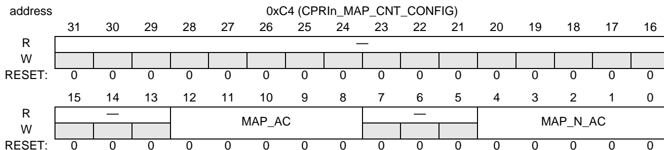
Figure 18-52. CPRIn_MAP_CNT_CONFIG
