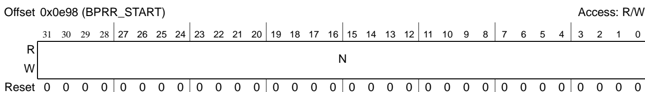
Figure 16-127. Buffer Pointer Range Release Start Register (BPRR_START)
