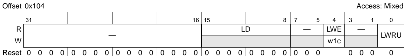
Figure 17-23. PCI Express Link Width Status Register (PEX_LWSR)
