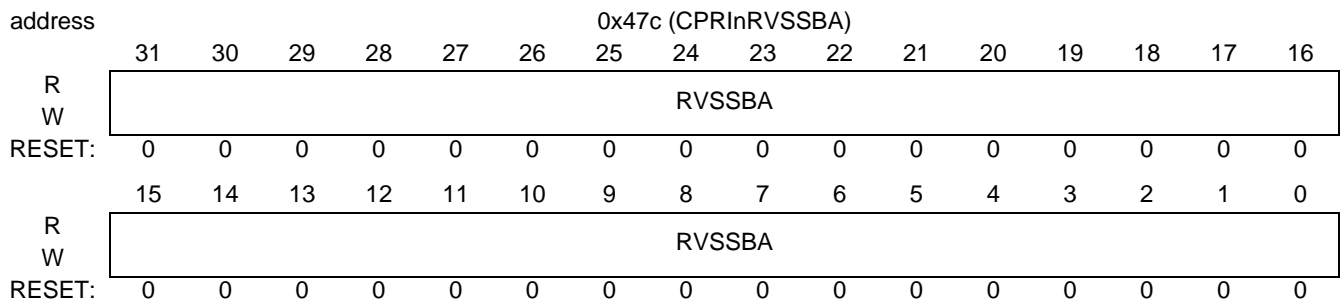
Figure 18-89. CPRInRVSSBA
