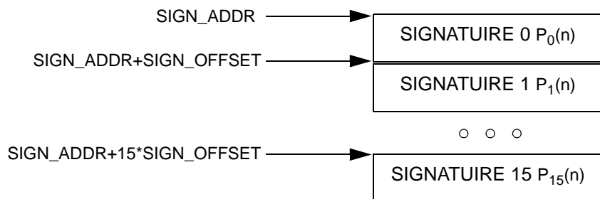
Figure 26-174. Signatures Data Structure in system memory
