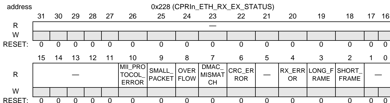
Figure 18-63. CPRIn_ETH_RX_EX_STATUS
