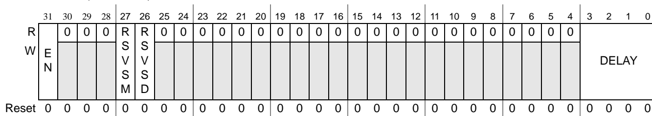
Figure 16-131. Dynamic Power Management Configuration (DPM_CFG)
