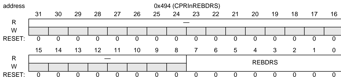
Figure 18-95. CPRInREBDRS
