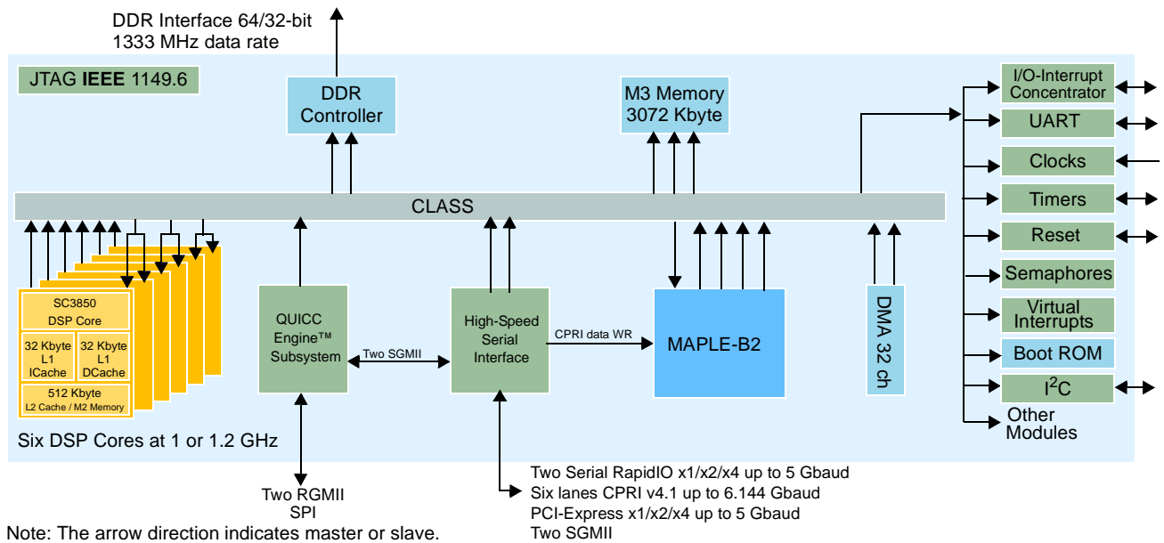
Figure 1-1. MSC8157 Block Diagram
