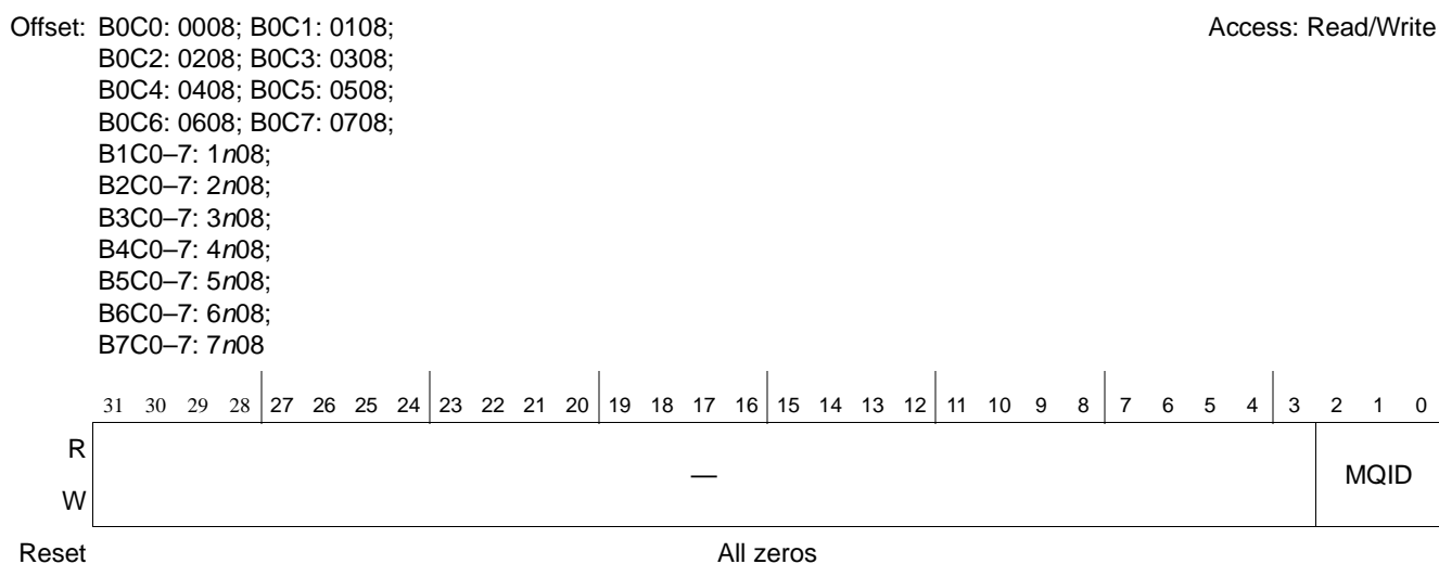
Figure 16-64. Inbound Block m Type10 Classification n Message Queue Register (IBmT10CnMQR)
