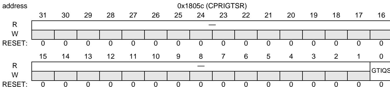
Figure 18-172. CPRIGtSR
