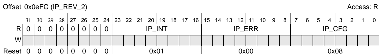
Figure 16-144. IP Block Revision 2 Register (IP_REV_2)
