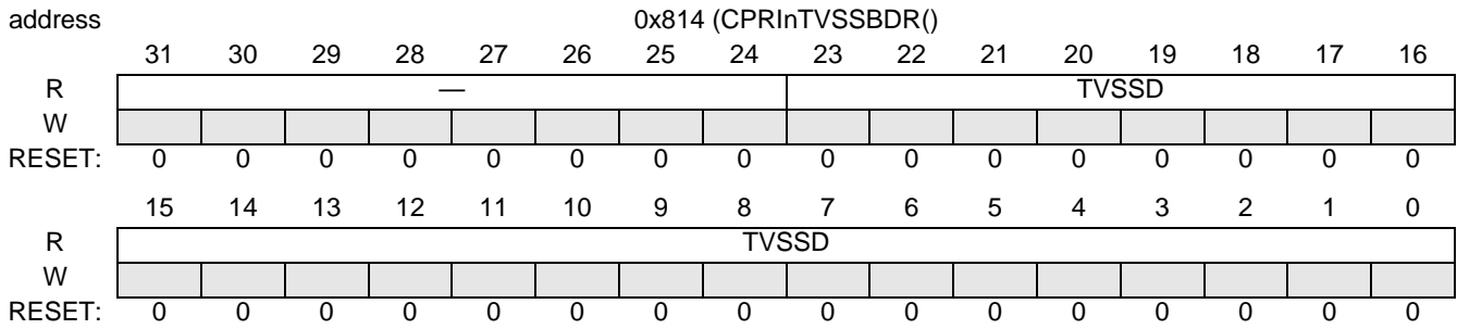
Figure 18-149. CPRInTVSSBDR
