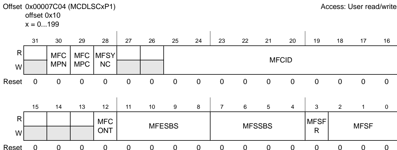
Figure 26-227. MAPLE CRPE-DL Fast Channel <x> Parameter 1
