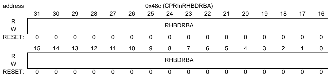
Figure 18-93. CPRInRHBDRBA
