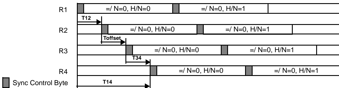
Figure 18-32. Single-Hop CPRI Frame Timing Diagram
