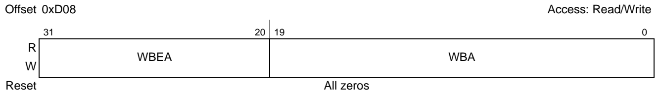
Figure 17-38. PCI Express MSI Inbound Window Base Address Register (PEXMSIIWBAR)
