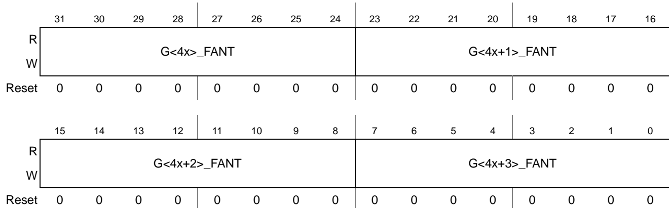
Figure 26-285. CRPE-ULB Group First Antenna x Configuration Register
