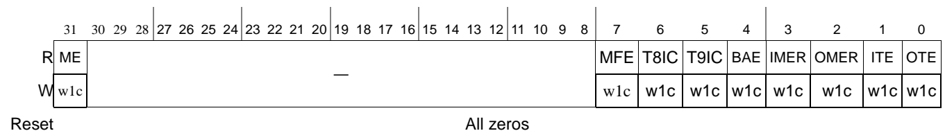
Figure 16-148. Message Unit Error Detect Register (MUEDR)
