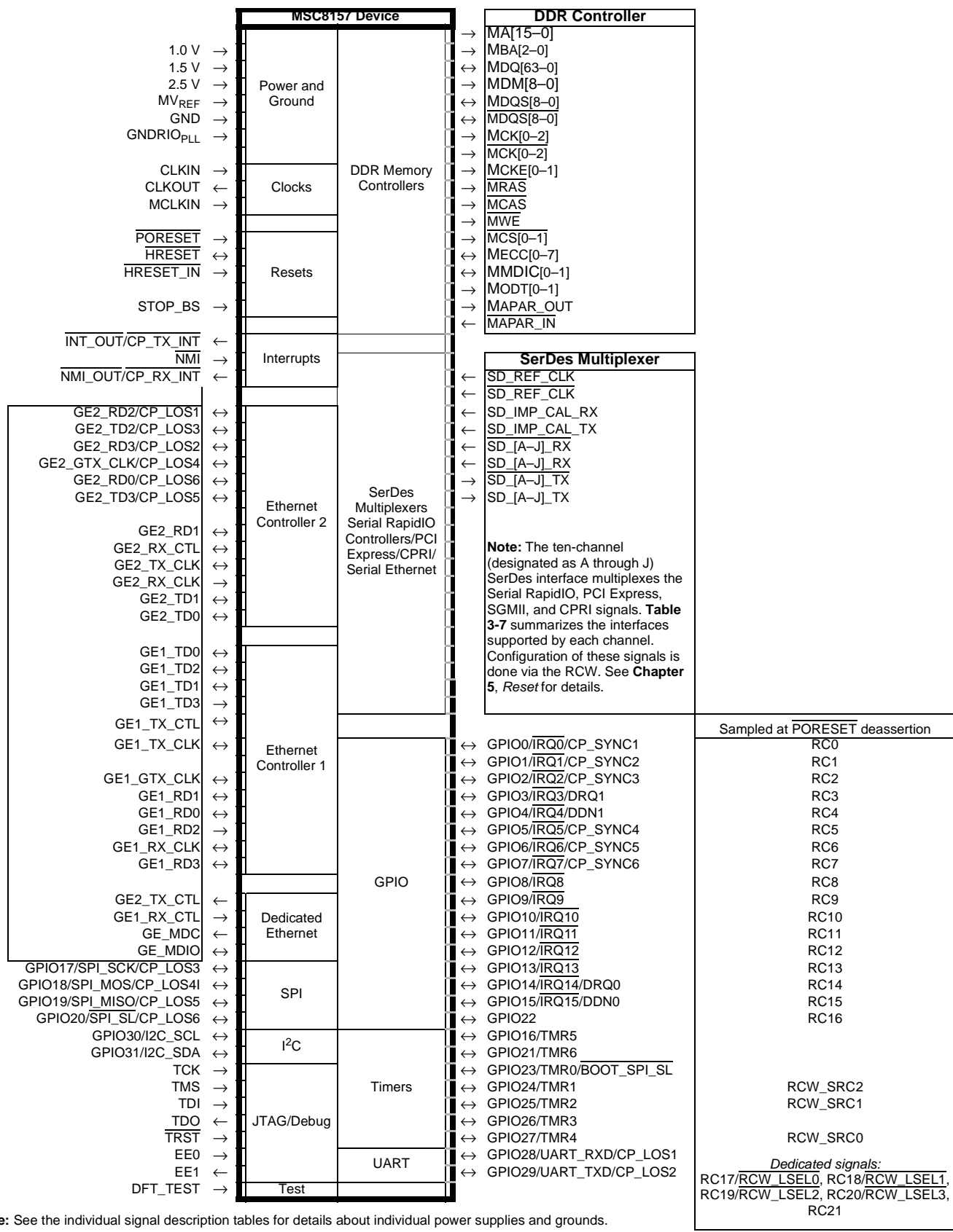
Figure 3-1. MSC8157 External Signals
