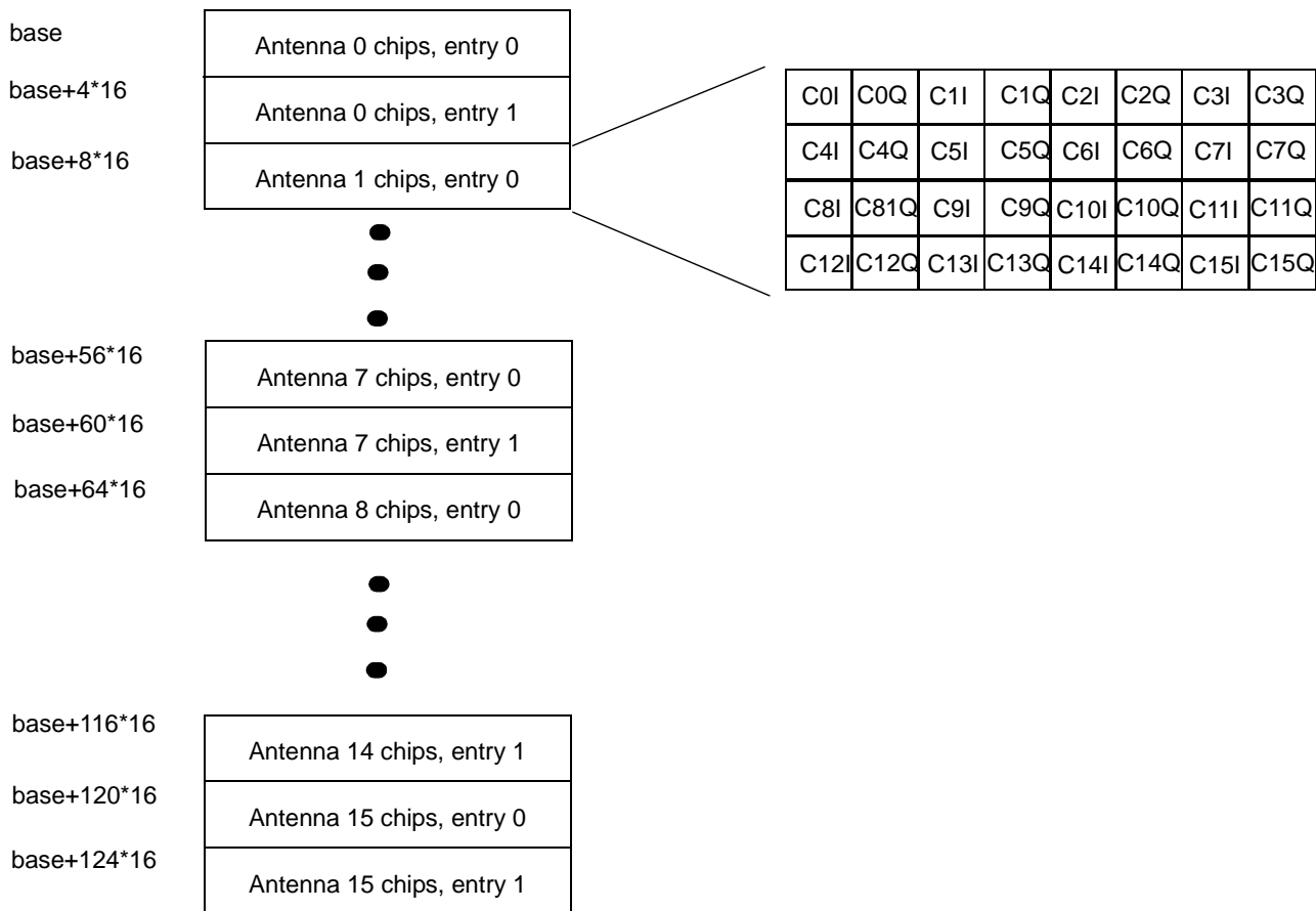
Figure 26-158. CRPE-DL Output Buffer Entry Data Organization Illustration
