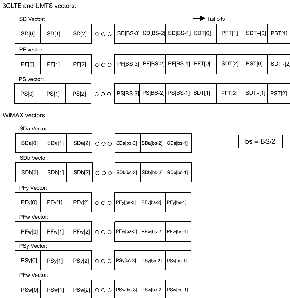
Figure 26-15. Expected Vectors Structure for Separate Vectors
