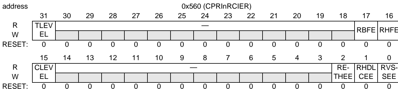
Figure 18-131. CPRInRCIER
