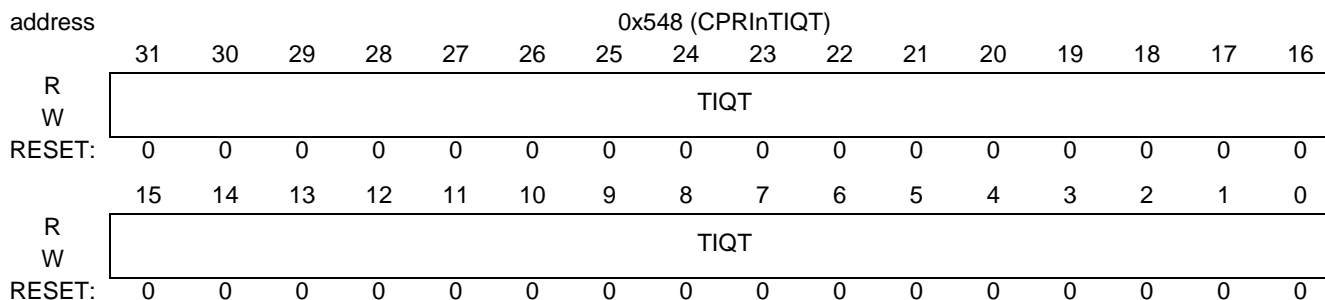
Figure 18-126. CPRInTIQT
