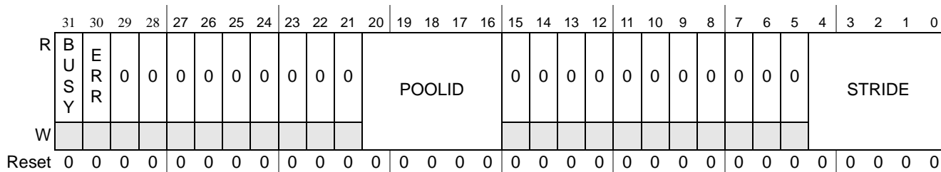
Figure 16-126. Buffer Pointer Range Release Configuration Register (BPRR_CFG)
