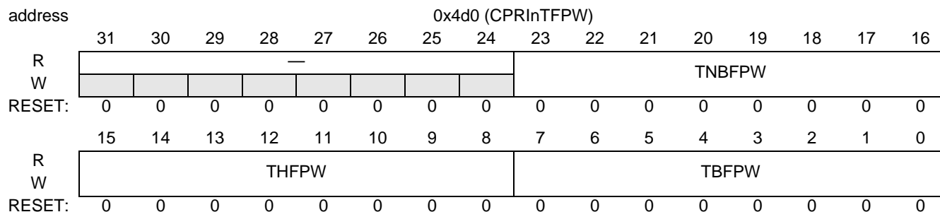
Figure 18-108. CPRInTFPW
