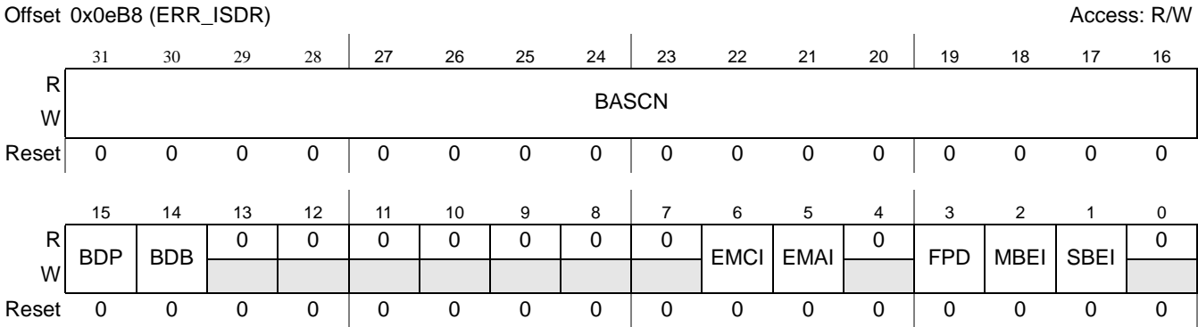
Figure 16-134. Interrupt Status Disable Register (ERR_ISDR)
