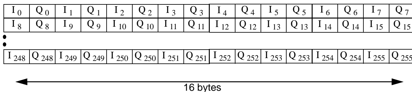
Figure 26-112. Sub Slot Data Structure
