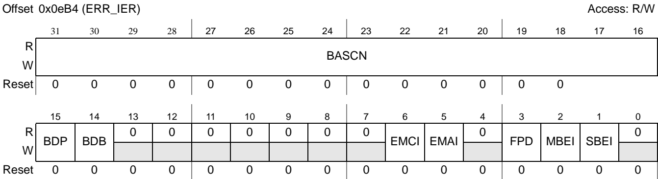
Figure 16-133. Error Interrupt Enable Register (ERR_IER)
