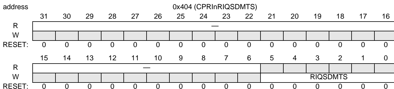
Figure 18-77. CPRInRIQSDMTS
