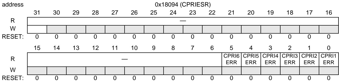
Figure 18-173. CPRIESR
