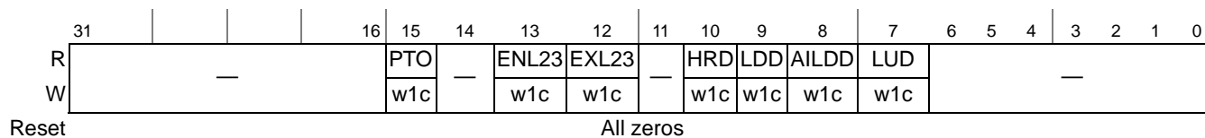
Figure 17-18. PCI Express PME and Message Detect Register (PEX_PME_MES_DR)
