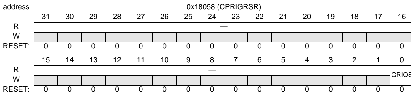
Figure 18-171. CPRIGRSR
