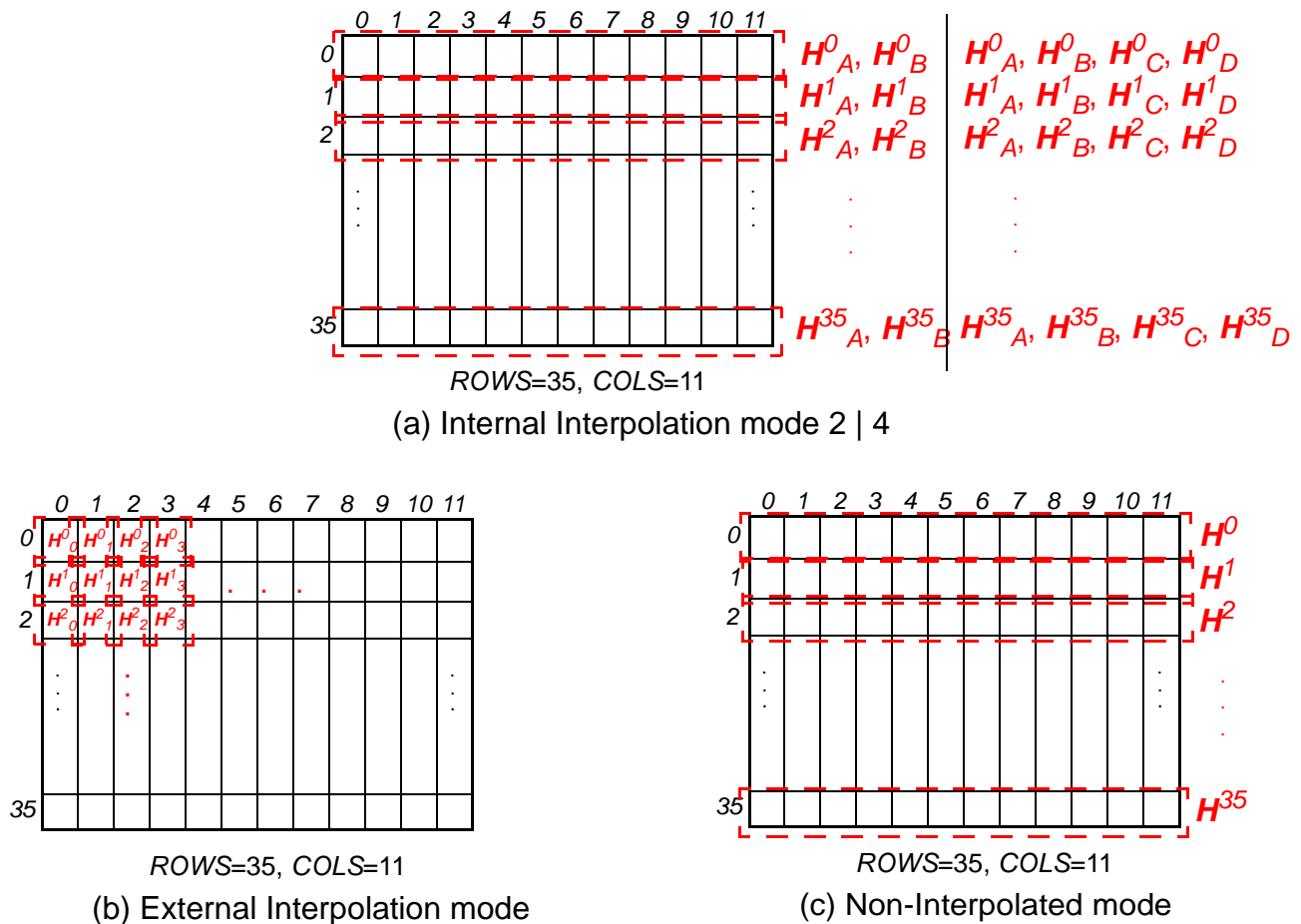
Figure 26-88. H Matrices Arrangement on Sub-Carrier Grid
