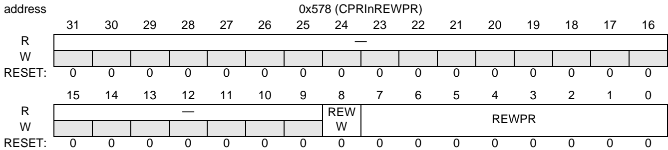
Figure 18-136. CPRInREWPR
