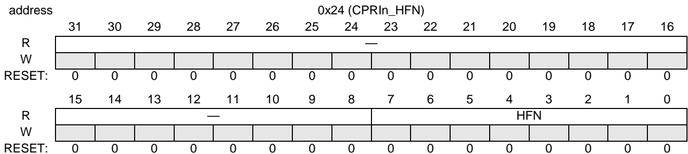
Figure 18-39. CPRIn_HFN
