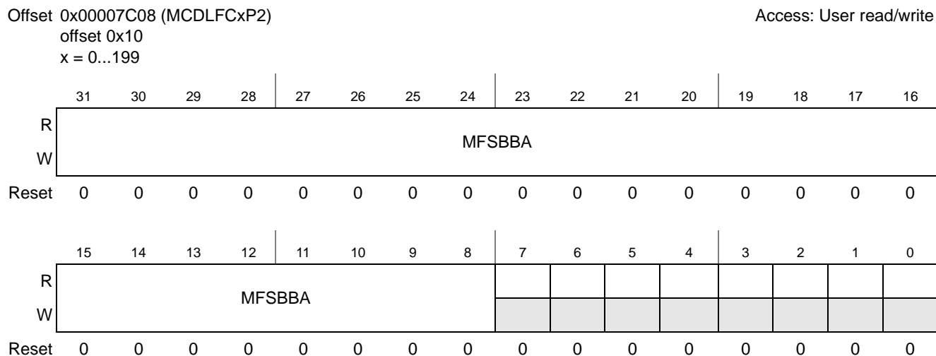
Figure 26-228. MAPLE CRPE-DL Fast Channel <x> Parameter 2
