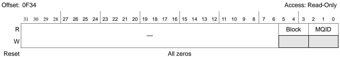
Figure 16-152. Message Unit Error Capture MQ Register (MUECMQR)
