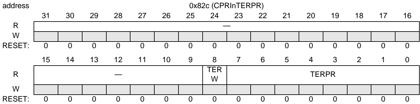
Figure 18-153. CPRInTERPR
