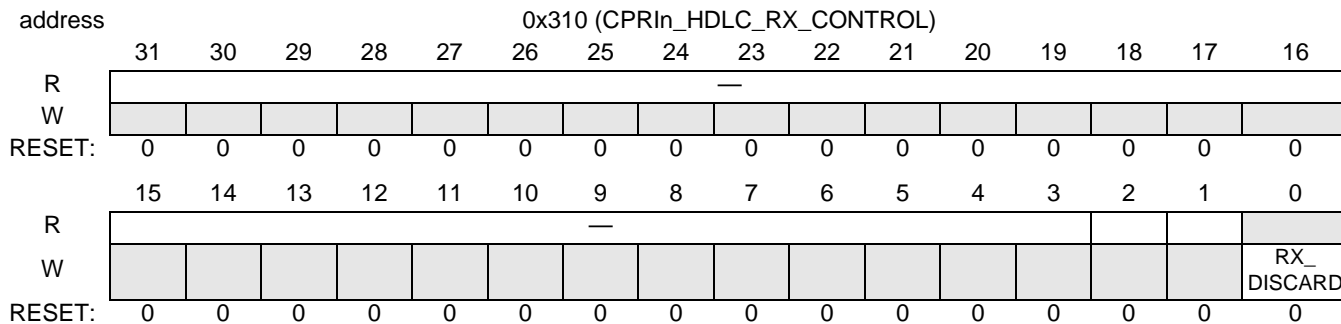
Figure 18-72. CPRIn_HDLC_RX_CONTROL
