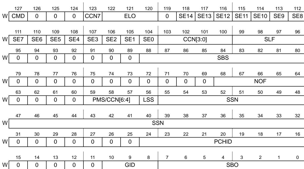
Figure 26-145. PCHC Structure
