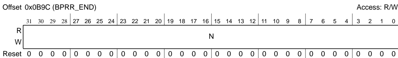
Figure 16-128. Buffer Pointer Range Release End Register (BPRR_END)
