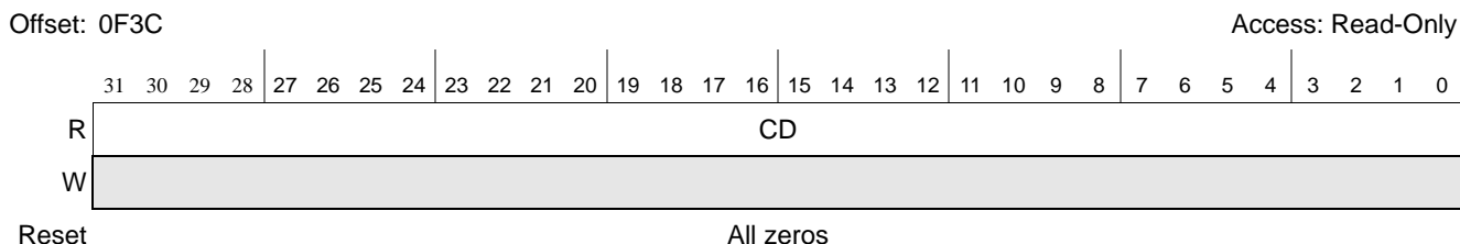
Figure 16-154. Message Unit Error Capture CD Register 1
