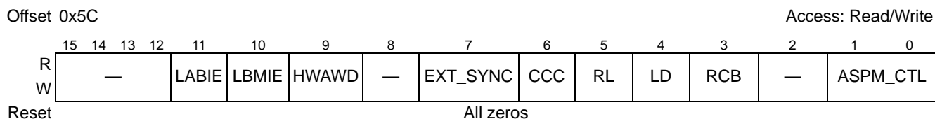
Figure 17-106. PCI Express Link Control Register
