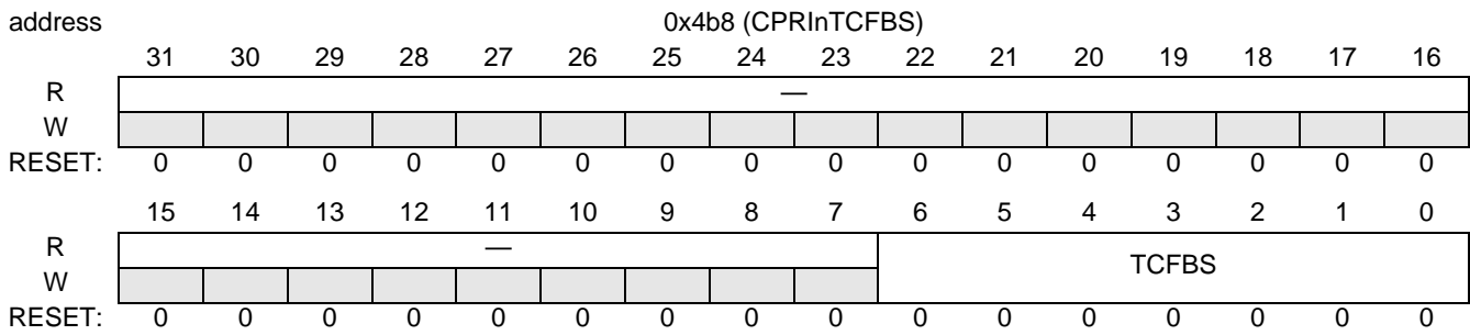
Figure 18-103. CPRInTCFBS
