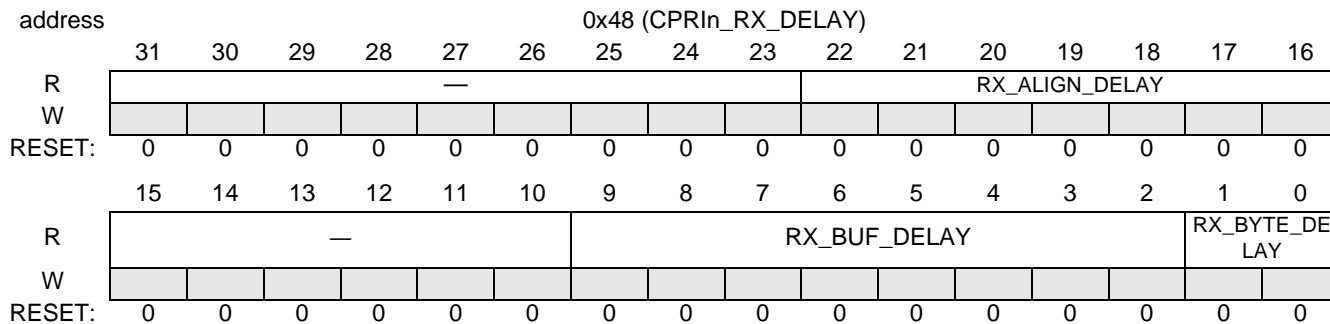
Figure 18-43. CPRIn_RX_DELAY
