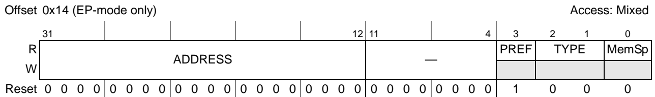
Figure 17-65. 32-Bit Memory Base Address Register (BAR1)
