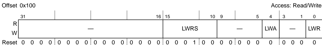
Figure 17-22. PCI Express Link Width Control Register (PEX_LWCR)
