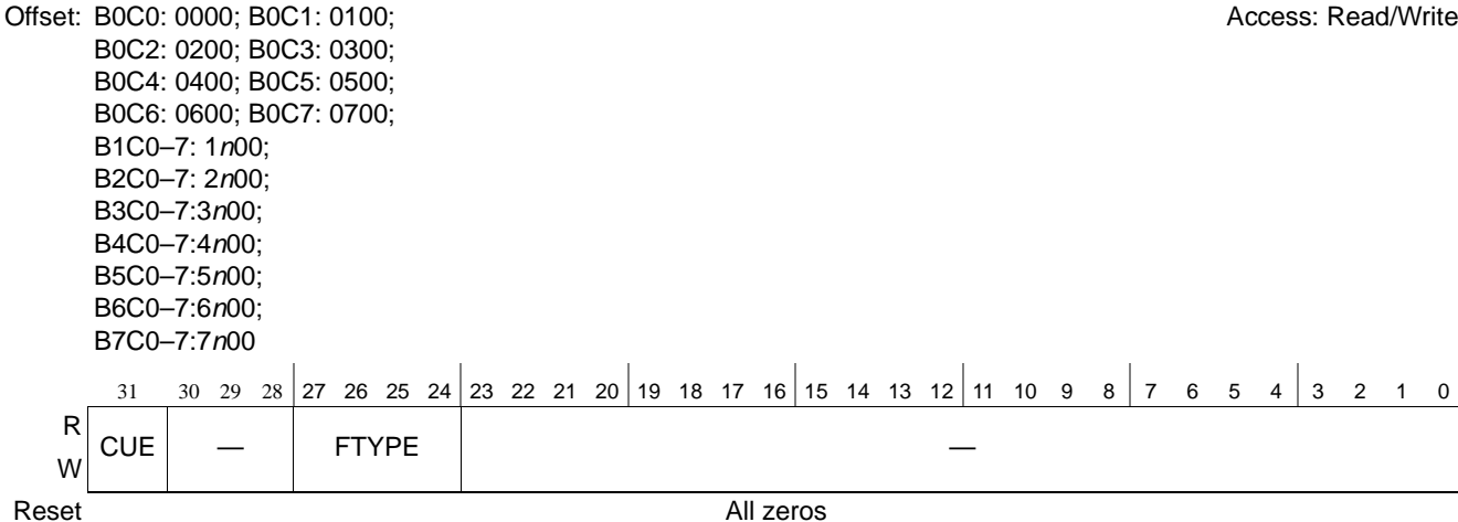
Figure 16-42. Inbound Block m Type8 Classification n Mode Register (IB m T8C n MR)
