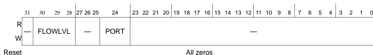
Figure 16-46. Inbound Block m Type8 Classification n Rule Value Register 1 (IB m T8C n RVR1)
