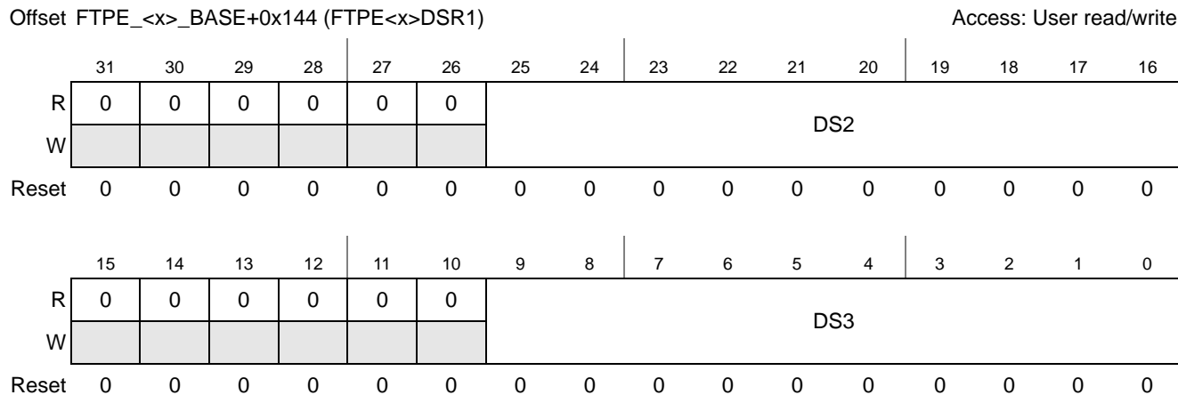
Figure 26-277. EFTPE_<x> Data Size Register 1
