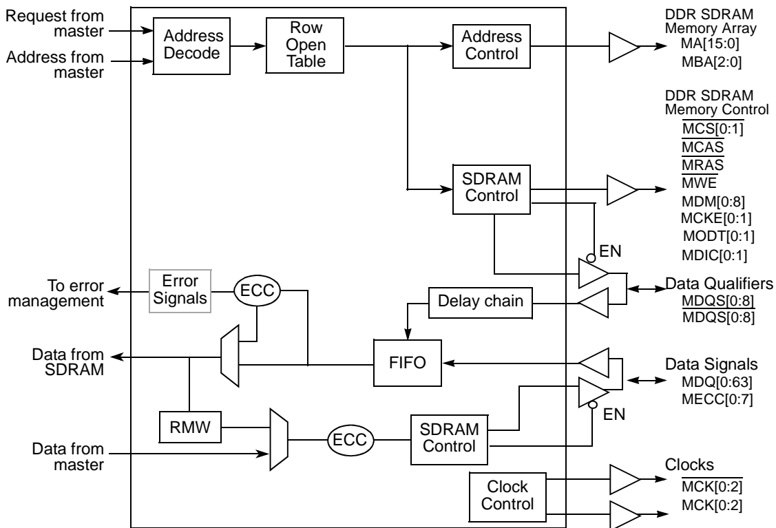
Figure 12-1. DDR SDRAM Memory Controller Simplified Block Diagram
