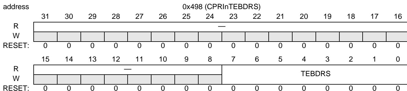
Figure 18-96. CPRInTEBDRS
