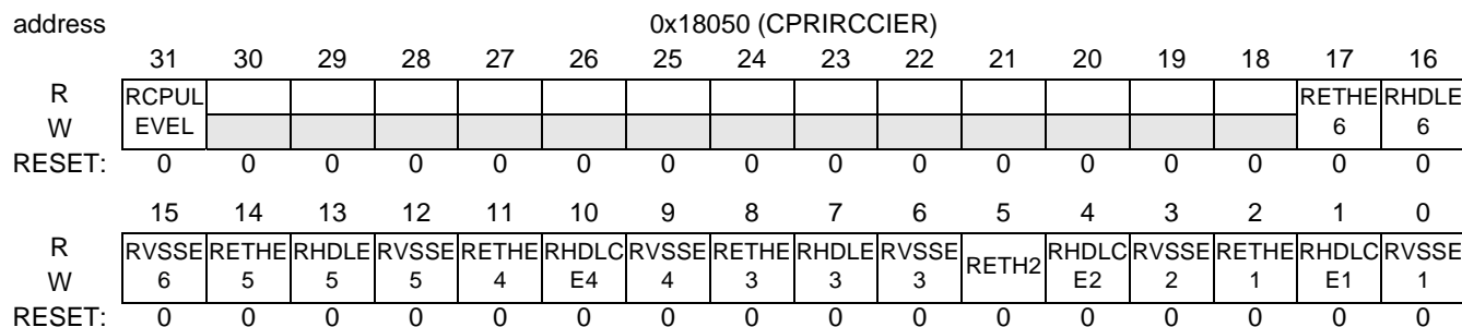
Figure 18-169. CPRIRCCIER
