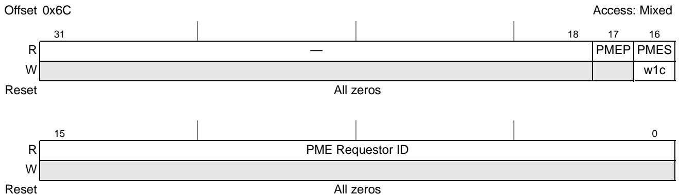
Figure 17-112. PCI Express Root Status Register
