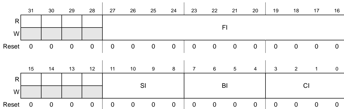
Figure 26-323. CRPE-DL Processing Stage Status Register
