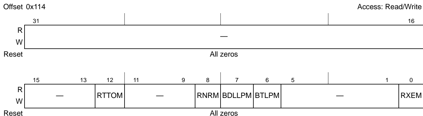
Figure 17-128. PCI Express Correctable Error Mask Register
