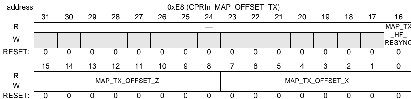
Figure 18-55. CPRIn_MAP_OFFSET_TX
