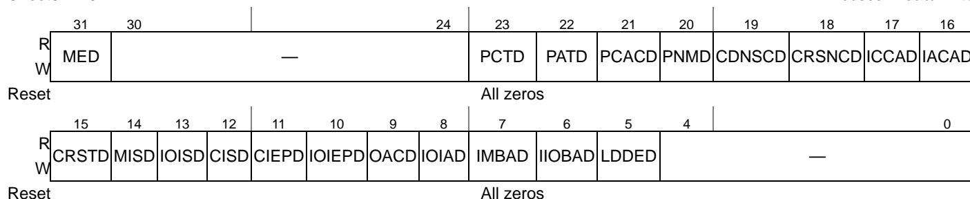
Figure 17-43. PCI Express Error Disable Register (PEX_ERR_DISR)
