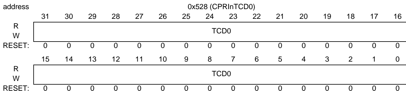
Figure 18-118. CPRInTCD0
