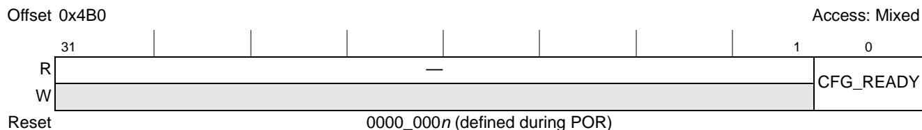
Figure 17-140. PCI Express Configuration Ready Register (PEX_CFG_READY)
