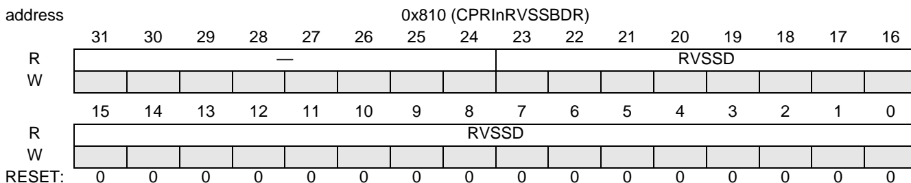
Figure 18-148. CPRInRVSSBDR
