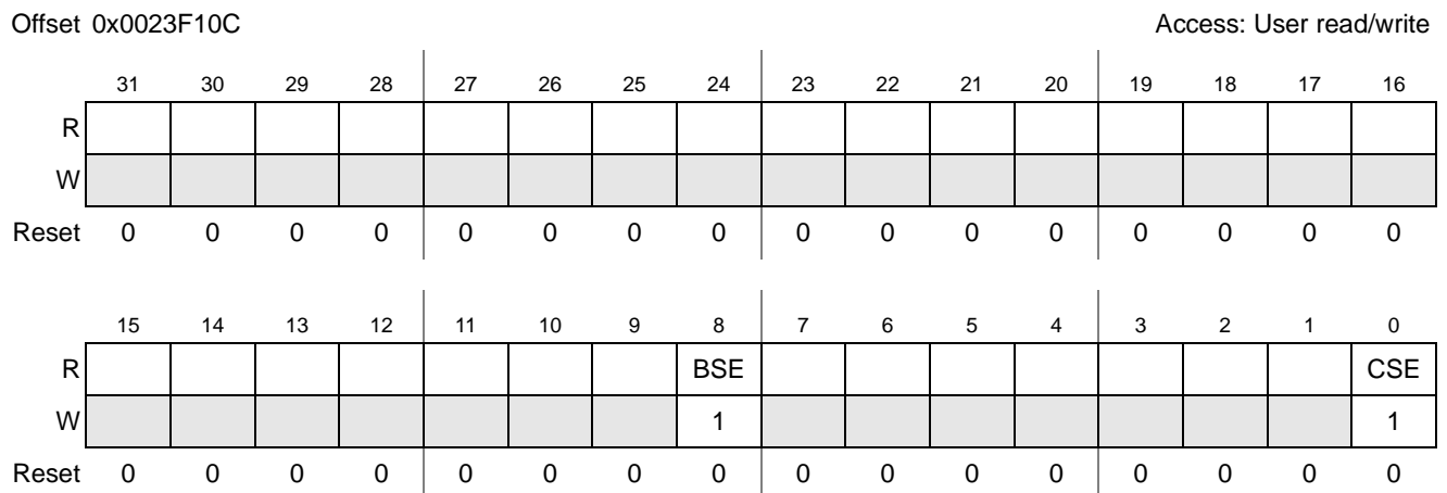
Figure 26-321. CRPE-DL Rate Control Register
