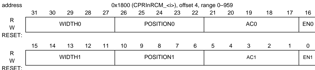
Figure 18-166. CPRInRCM_<i>)</i>
