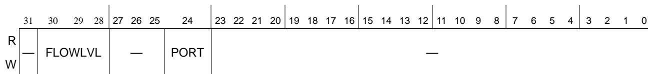
Figure 16-66. Inbound Block m Type10 Classification n Rule Value Register 1 (IBmT10CnRVR1)
