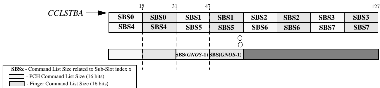
Figure 26-103. Command List Size Data Structure
