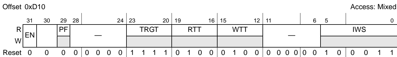
Figure 17-40. PCI Express MSI Inbound Window Attributes Register (PEXMSIIWAR)
