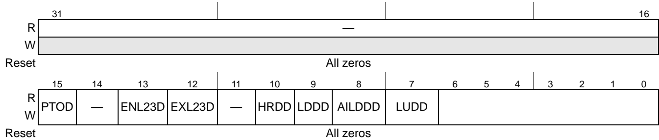
Figure 17-19. PCI Express PME and Message Disable Register (PEX_PME_MES_DISR)
