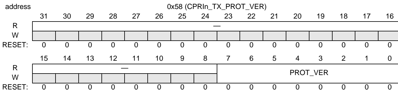
Figure 18-47. CPRIn_TX_PROT_VER
