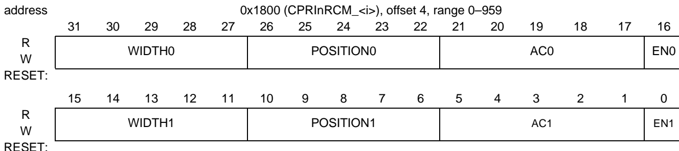
Figure 18-167. CPRInRCM_<i> </i>
