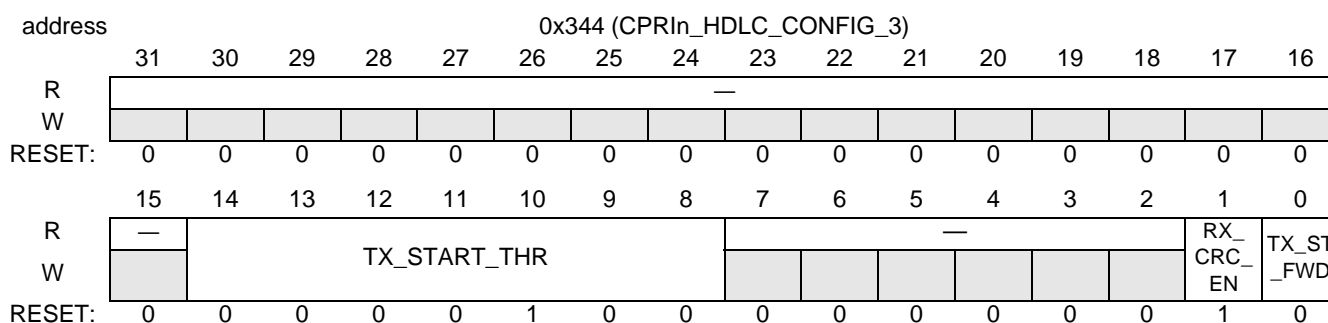
Figure 18-74. CPRIn_HDLC_CONFIG_3
