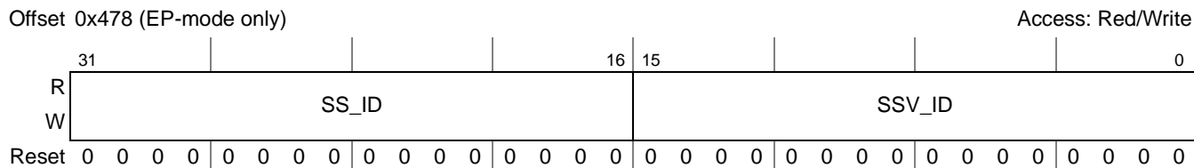
Figure 17-139. PCI Express Subsystem Vendor ID Update Register (PEX_SSVID_UPDATE)
