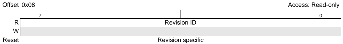
Figure 17-58. PCI Express Revision ID Register
