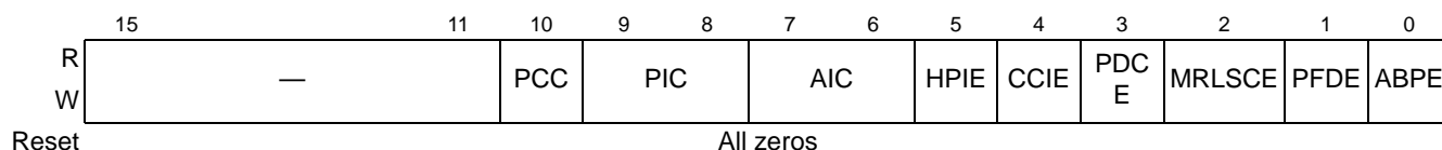
Figure 17-109. PCI Express Slot Control Register
