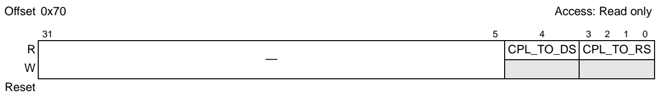
Figure 17-113. PCI Express Device Capabilities 2 Register
