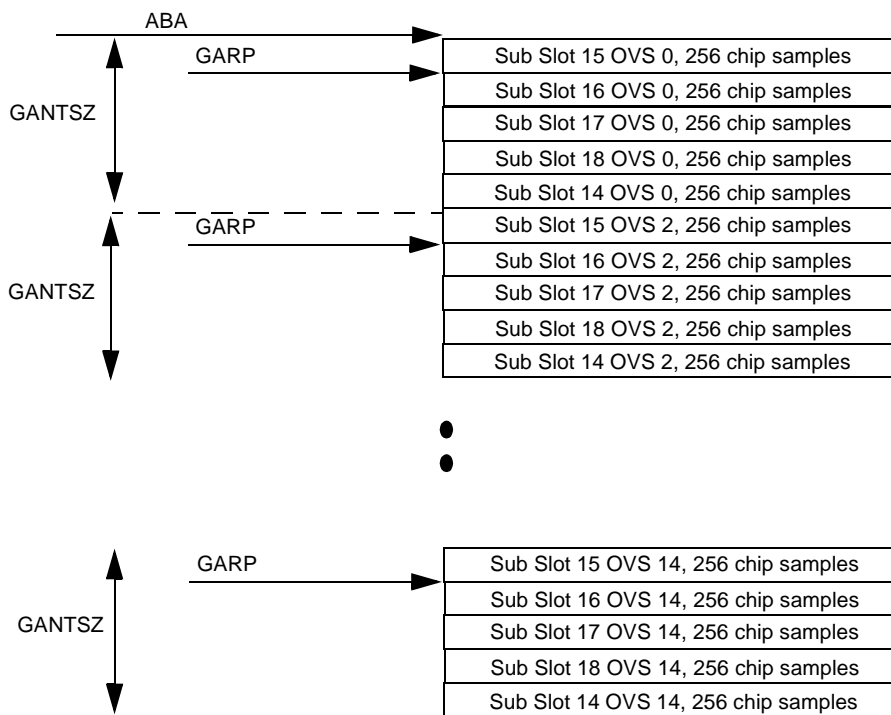
Figure 26-110. Single Antenna Input Data Structure Where GANTSZ=5, INT\_MODE = 0, IIL=2
