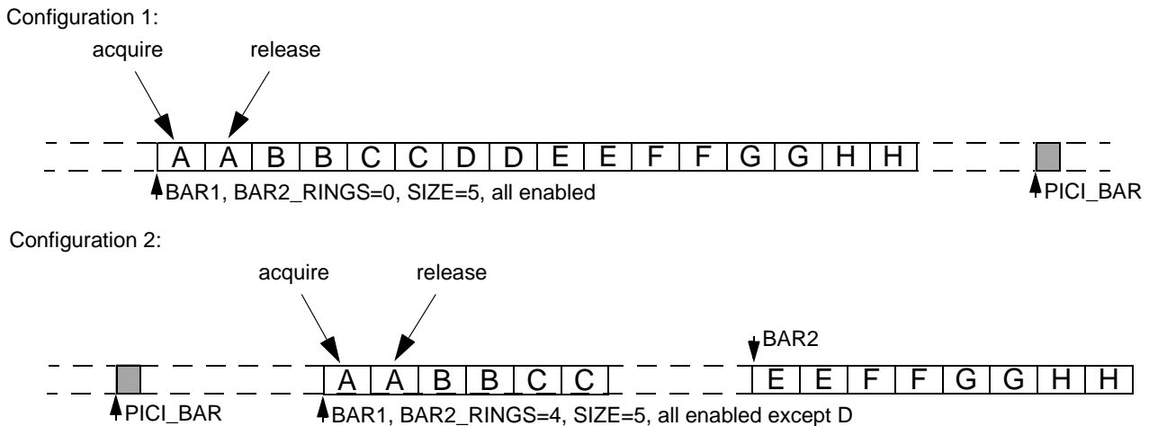
Figure 16-101. Example Ring Buffer Memory Footprints
