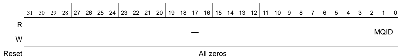
Figure 16-44. Inbound Block m Type8 Classification n Message Queue Register (IBmT8CnMQR)
