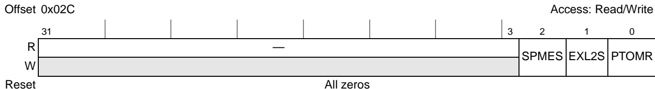
Figure 17-21. PCI Express Power Management Command Register (PEX_PMCR)
