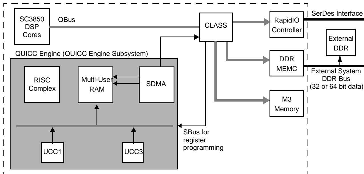
Figure 19-4. MSC8157 Data Paths
