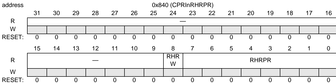
Figure 18-156. CPRInRHRPR
