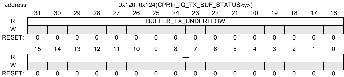
Figure 18-58. CPRIn_IQ_TX_BUF_STATUS<Y>
