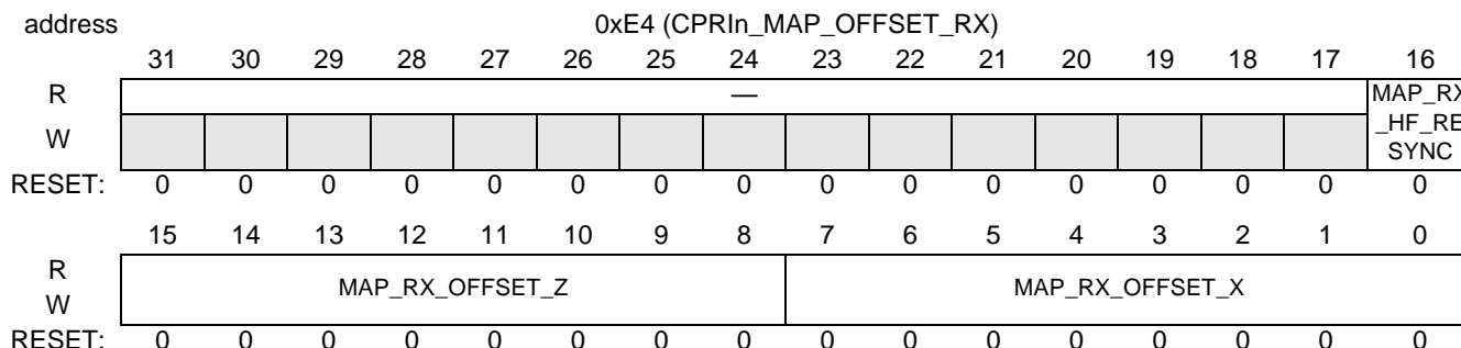
Figure 18-54. CPRIn_MAP_OFFSET_RX
