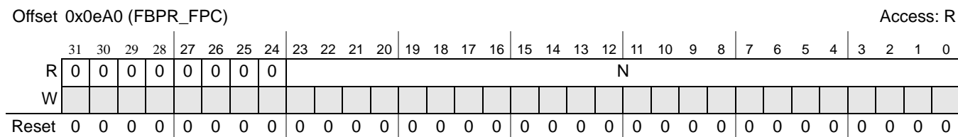
Figure 16-129. Free Buffer Proxy Record Free Pool Count Register (FBPR_FPC)
