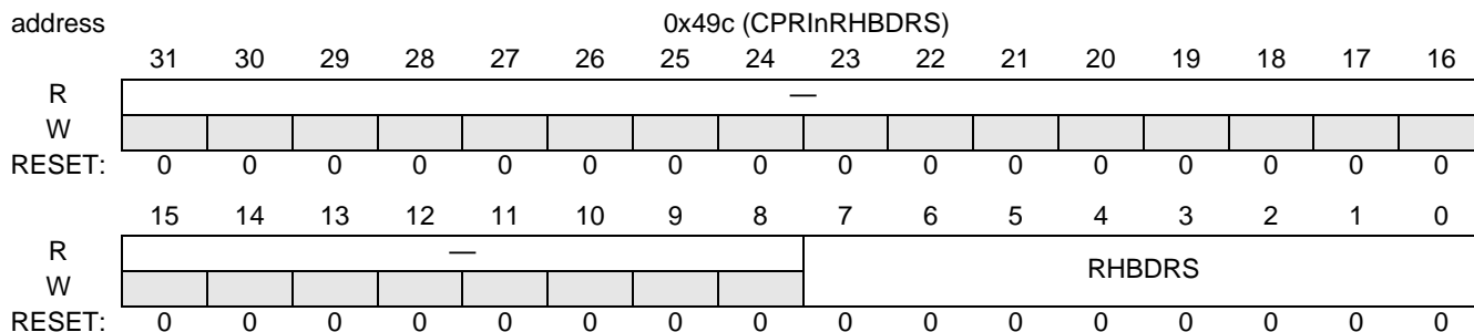
Figure 18-97. CPRInRHBDRS
