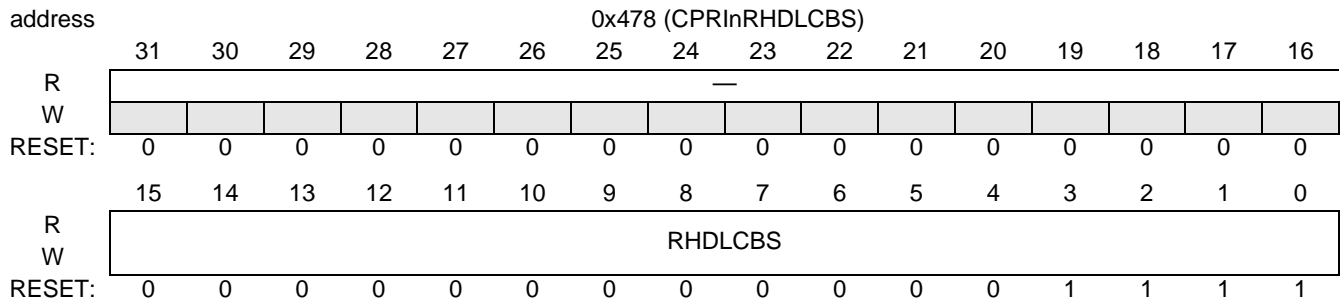
Figure 18-88. CPRInRHDLCS
