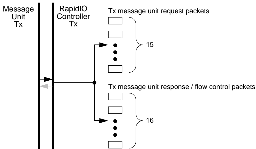
Figure 16-5. Tx Message Unit Packet Buffers
