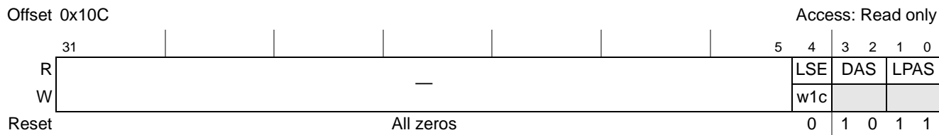
Figure 17-25. PCI Express Link Speed Status Register (PEX_LSSR)
