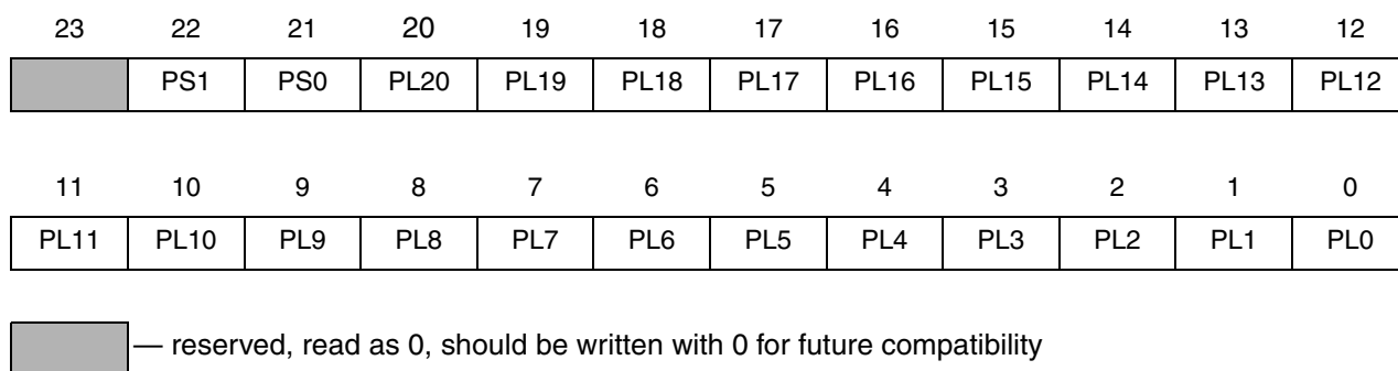
Figure 11-4 Timer Prescaler Load Register (TPLR)
