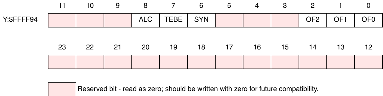
Figure 9-9 SAICR_1 Register
