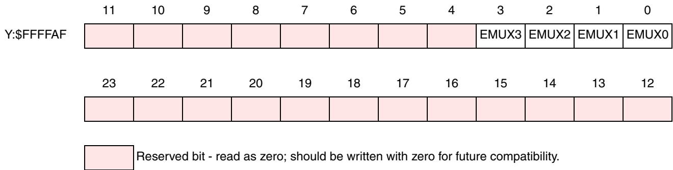
Figure 9-2 EMUXR Register
