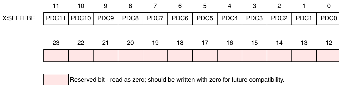
Figure 8-20 PRRC Register
