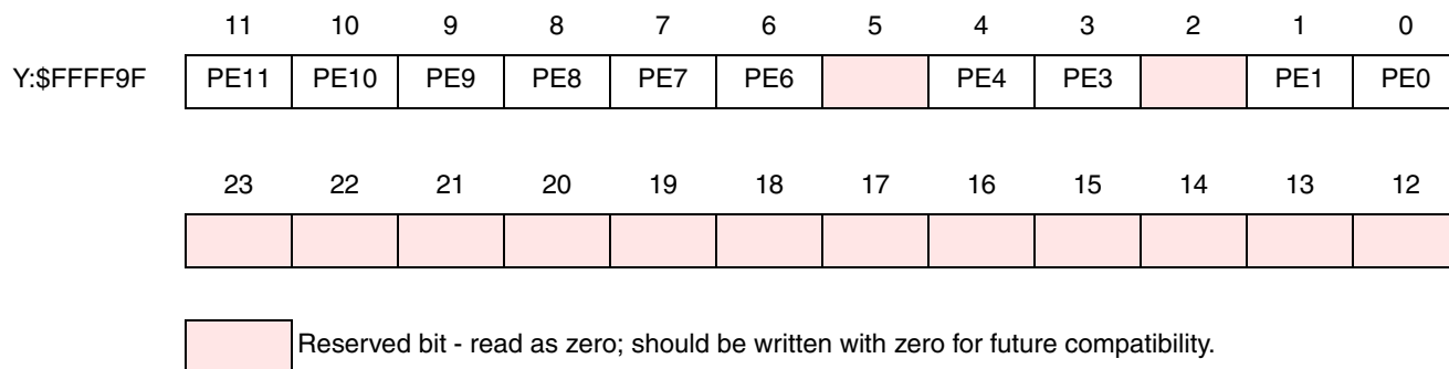
Figure 9-15 PCRE Register
