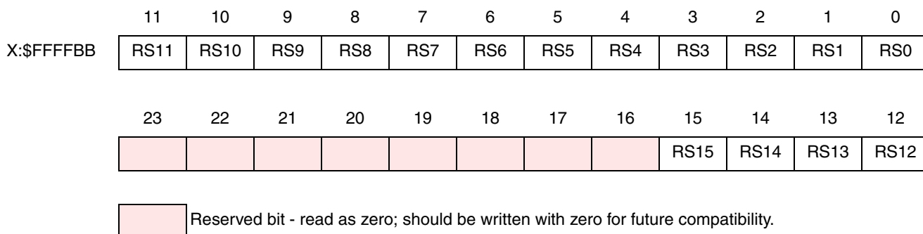
Figure 8-17 RSMA Register
