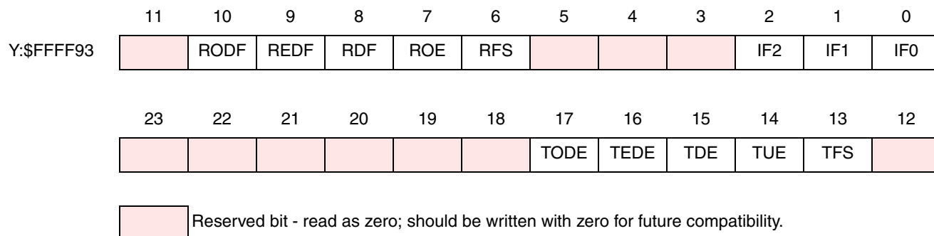
Figure 9-10 SAISR_1 Register
