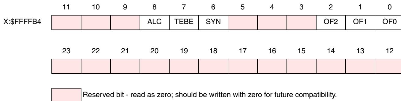
Figure 8-10 SAICR Register
