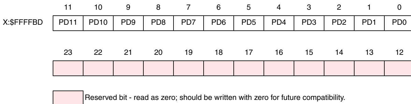
Figure 8-21 PDRC Register
