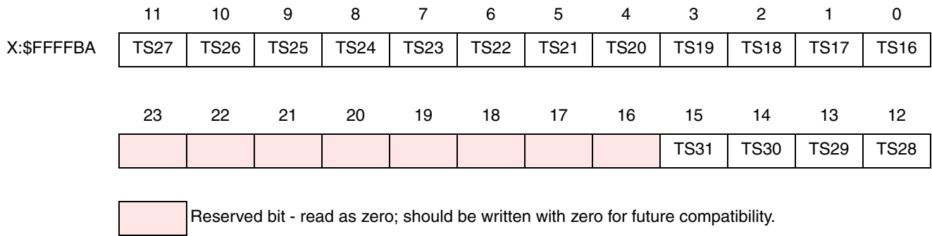
Figure 8-16 TSMB Register
