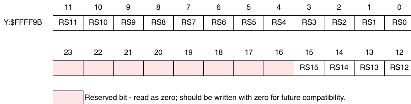
Figure 9-13 RSMA_1 Register
