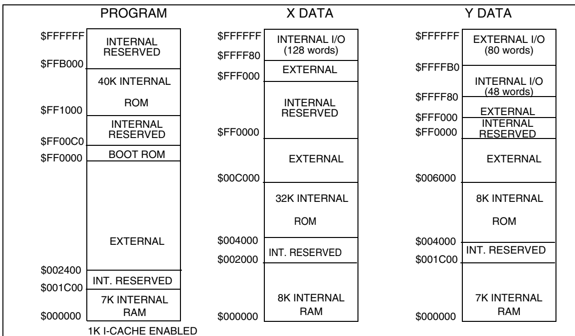
Figure 3-7 Memory Maps for MSW=(0,1), CE=1, MS=1, SC=0
