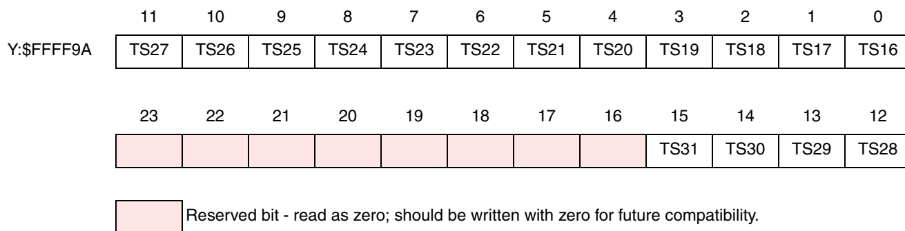
Figure 9-12 TSMB_1 Register
