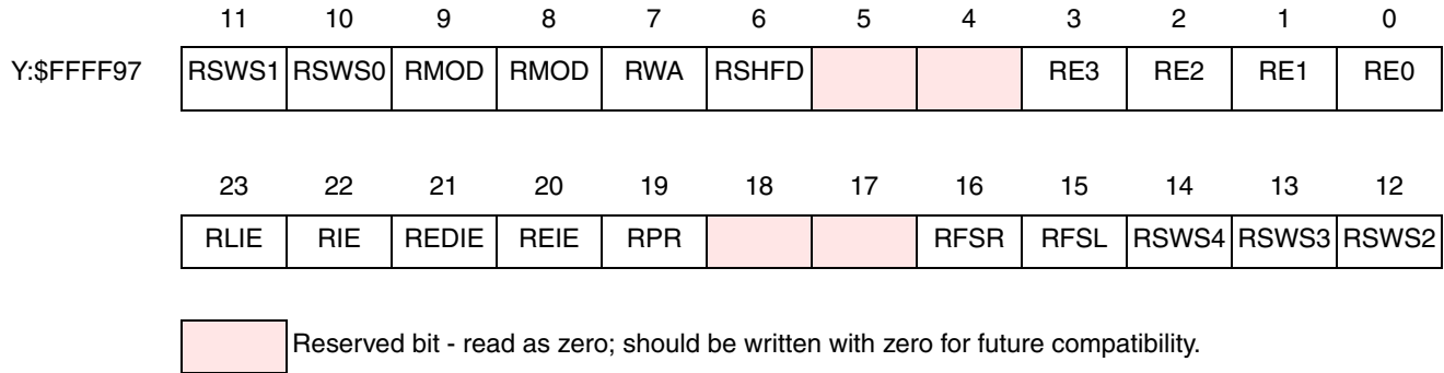
Figure 9-8 RCR_1 Register
