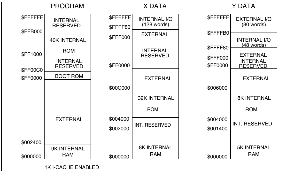
Figure 3-6 Memory Maps for MSW=(0,0), CE=1, MS=1, SC=0
