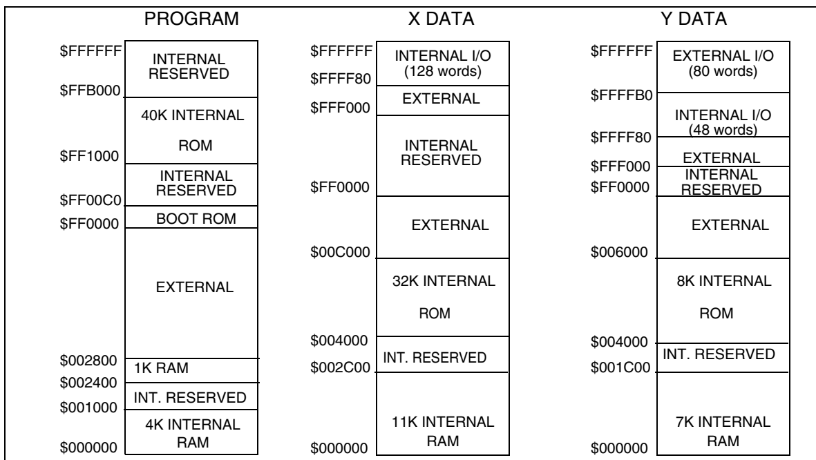
Figure 3-5 Memory Maps for MSW=(1,0), CE=0, MS=1, SC=0
