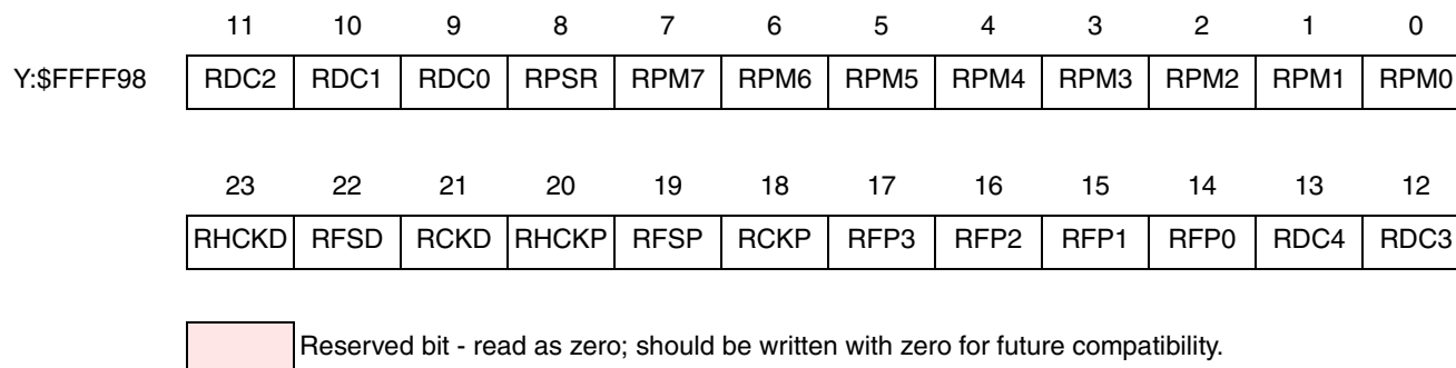
Figure 9-7 RCCR_1 Register
