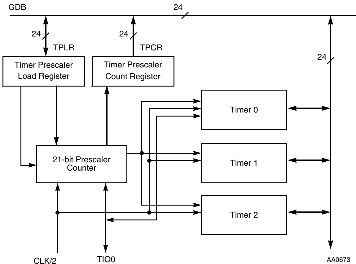
Figure 11-1 Timer/Event Counter Block Diagram
