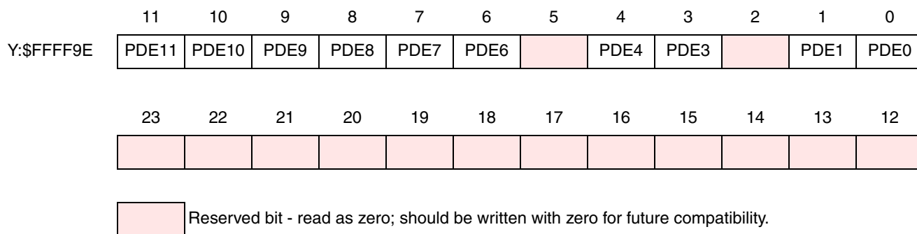
Figure 9-16 PRRE Register
