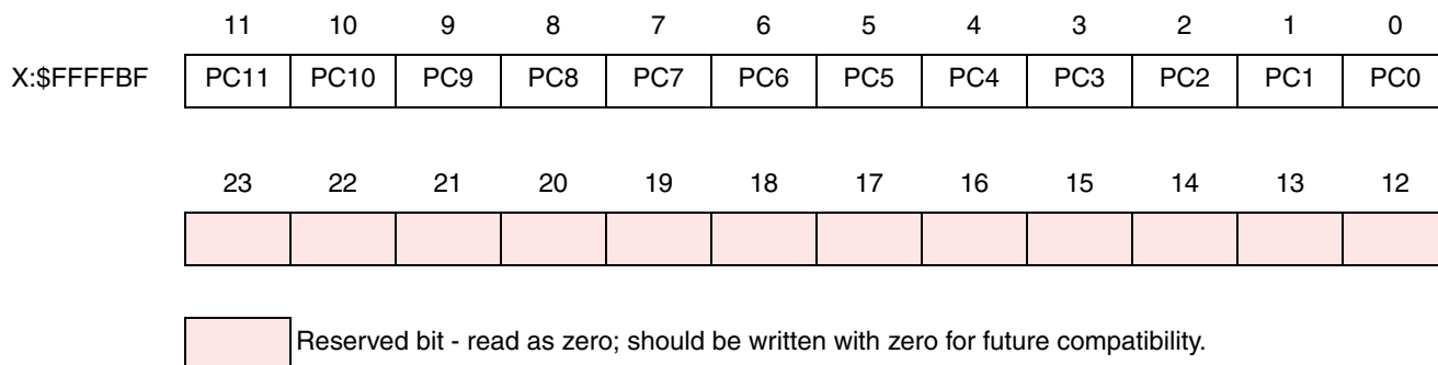
Figure 8-19 PCRC Register
