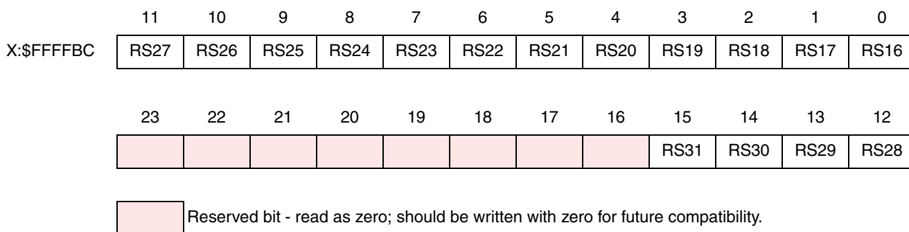
Figure 8-18 RSMB Register
