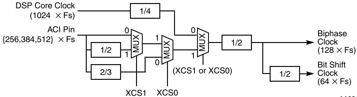
Figure 10-5 Clock Multiplexer Diagram
