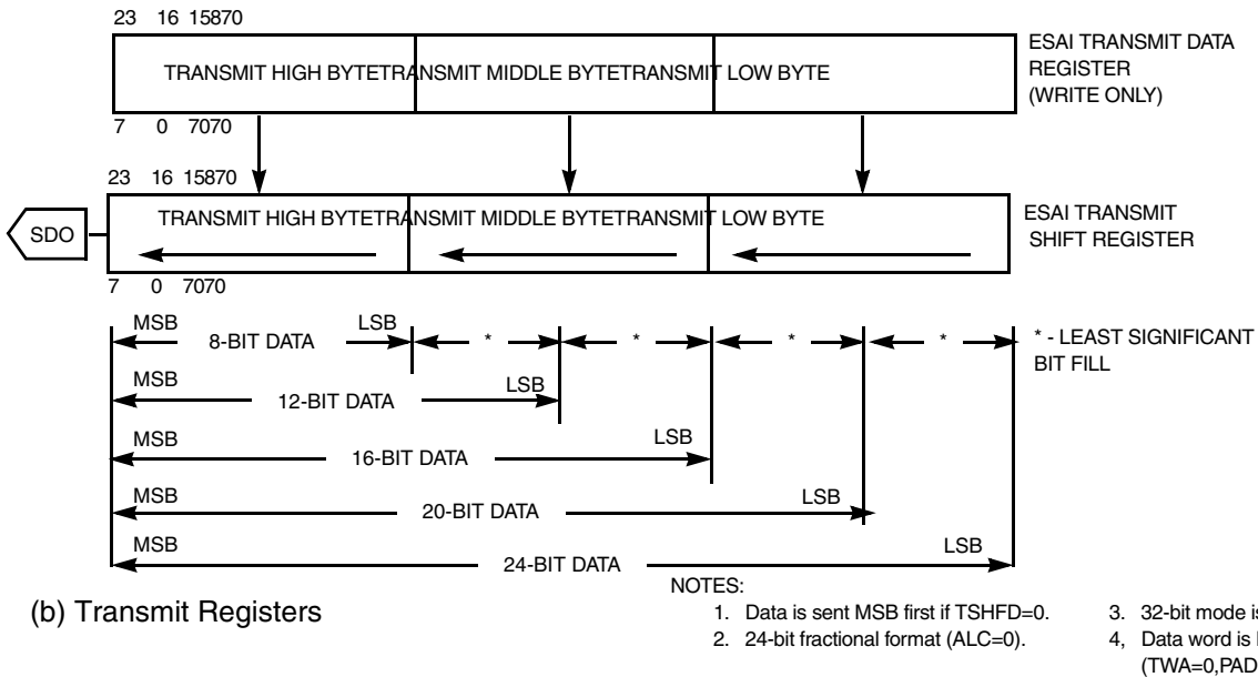
Figure 8-13 ESAI Data Path Programming Model ([R/T]SHFD=0)
