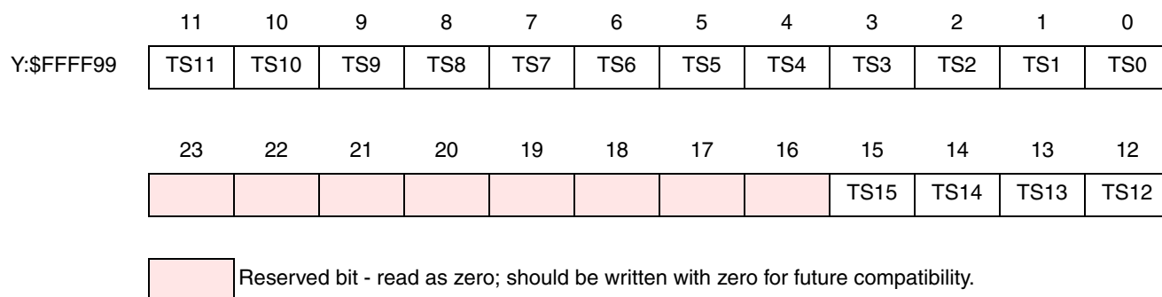
Figure 9-11 TSMA_1 Register
