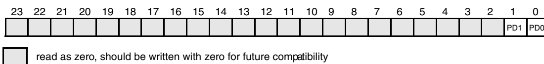
Figure 10-8 Port D Data Register (PDRD)
