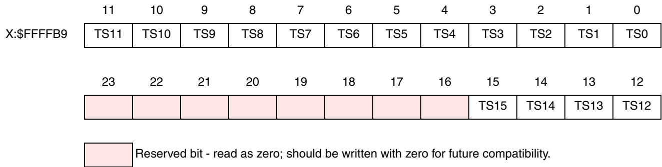
Figure 8-15 TSMA Register
