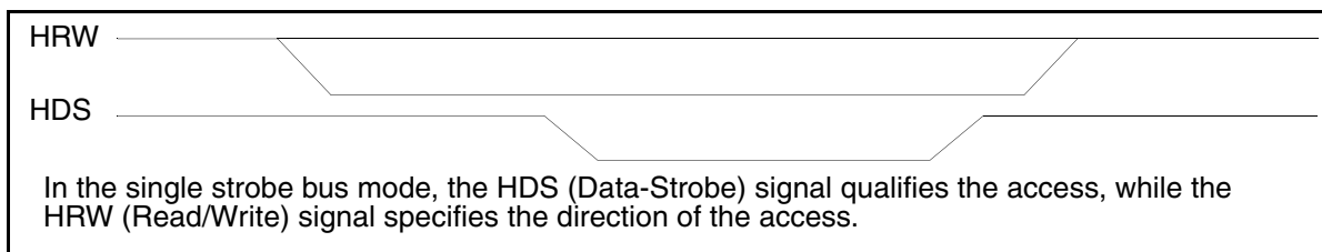
Figure 6-7 Single strobe bus
