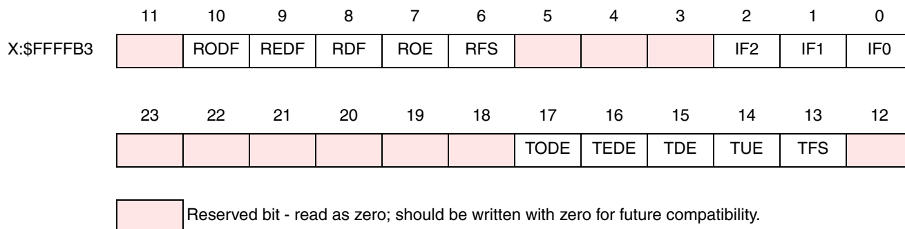
Figure 8-12 SAISR Register
