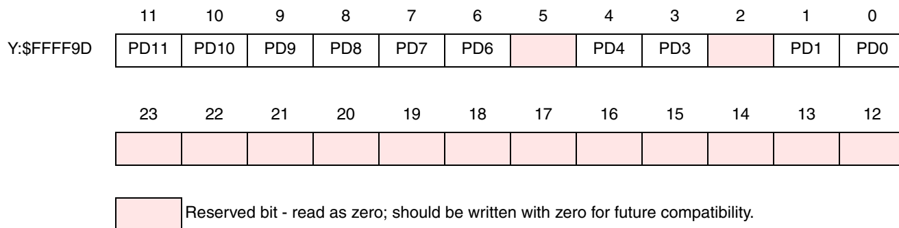
Figure 9-17 PDRE Register
